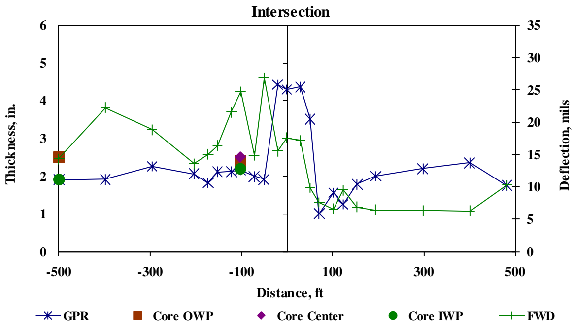
Figure 5.16 - GPR, FWD and Cores on SH 155.
