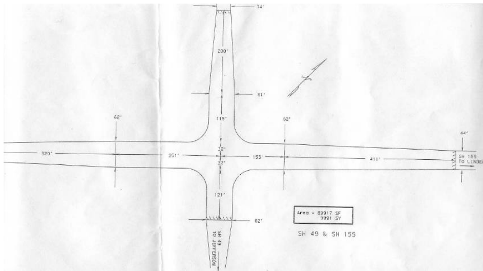
Figure 5.2 - Geometry of SH 155 and SH 49 Intersection.
