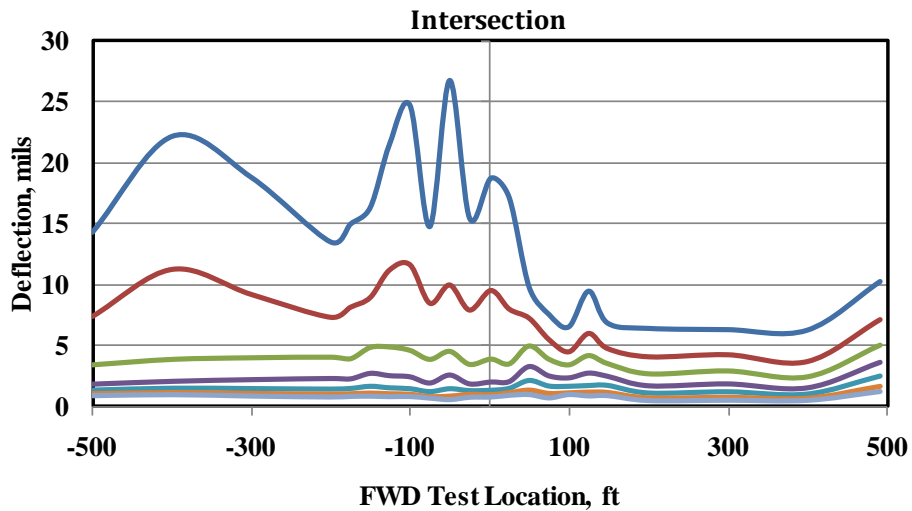
Figure 5.13 - FWD Deflection Results on Eastbound SH 155.
