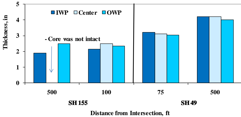
Figure 5.10 - Core Average Thicknesses as Approaching the Intersection.
