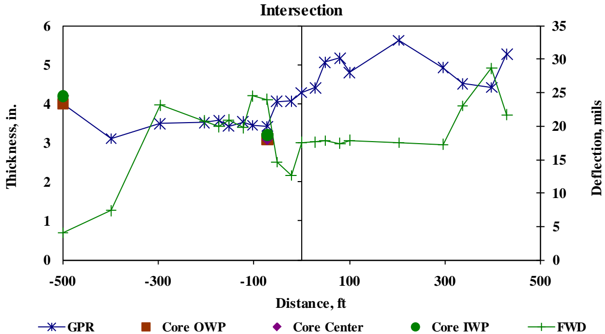
Figure 5.17 - GPR, FWD and Cores on SH 49.
