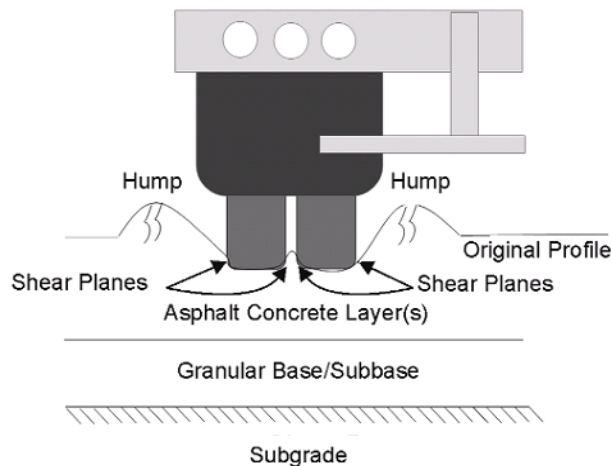
Figure 2.4 - Instability or Plastic Flow on Asphalt Pavements (Federation of Canadian Municipalities and Canadian National Research Council 2003).
