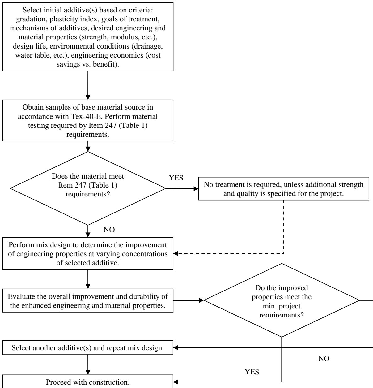
Figure 2.9 - TxDOT Flowchart for Base Treatment (TxDOT, 2005)
