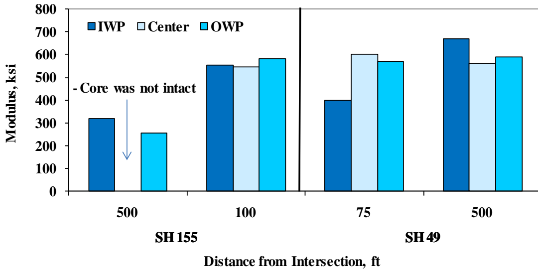
Figure 5.11 - Core Average Modulus as Approaching the Intersection.
