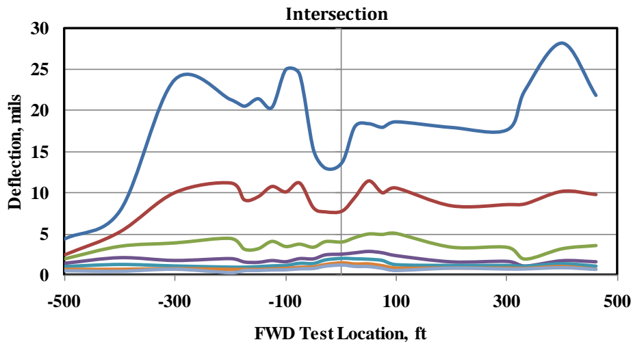
Figure 5.13 - FWD Deflection Results on Eastbound SH 155.
