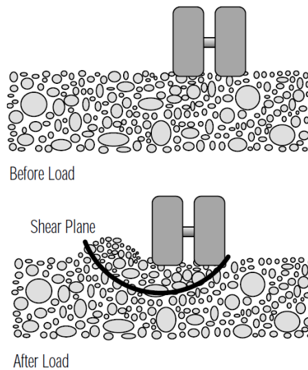
Figure 8.4 - Illustration of Instability Rutting.
