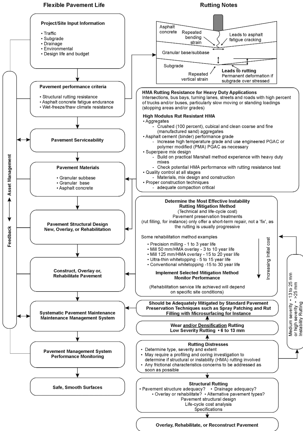
Figure 2.8 - Flowchart of Activities for Mitigating Intersection Rutting.
