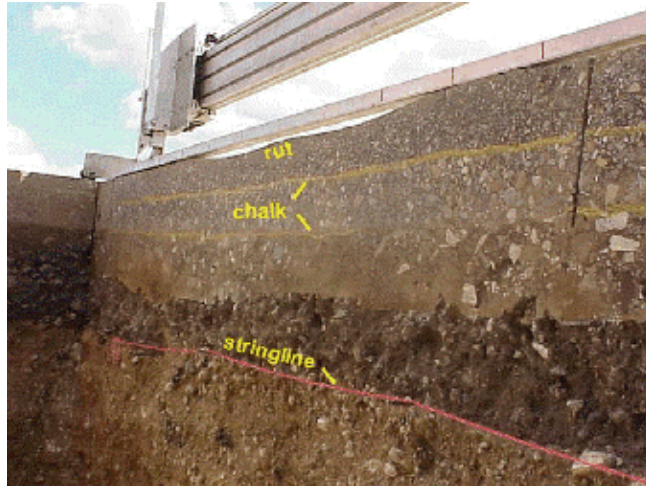
Figure 8.2 - Trench as part of a Forensic study to Identify Structural Rutting.
