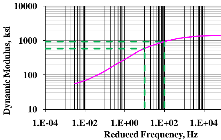
Figure 8.5 - Example of Dynamic Modulus Test Results a.k.a. Master Curve.
