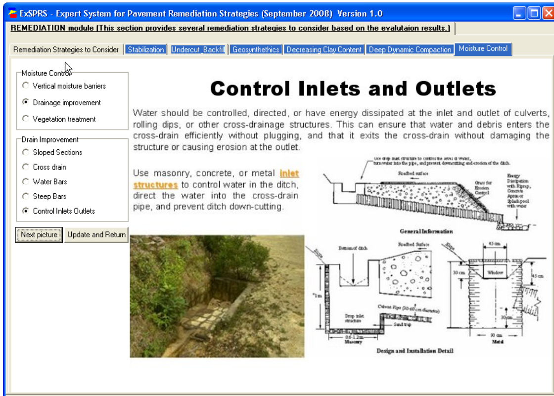
Figure 4.11—Moisture Control Method of Using Inlets and Outlets
