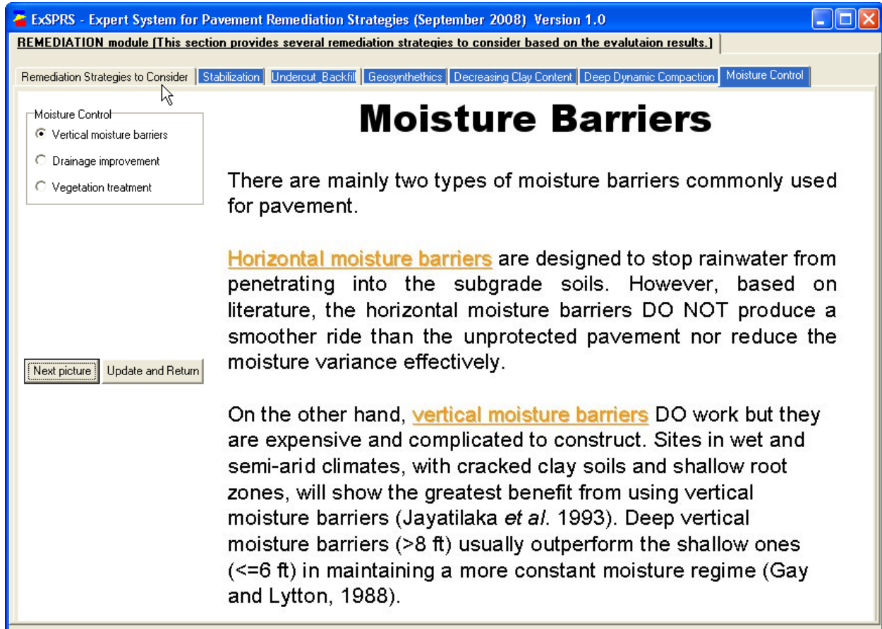
Figure 4.6—Moisture Control Method of Using Moisture Barriers
