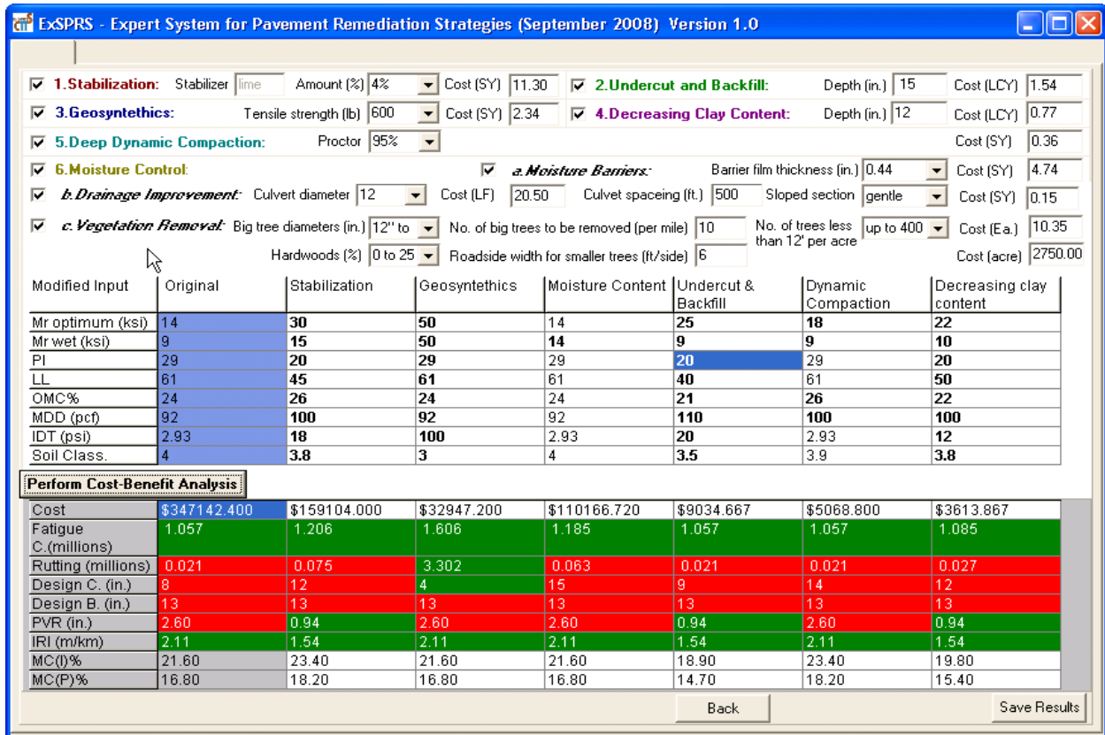
Figure 5.3- Cost-Benefit Results for the Remediation Strategies
