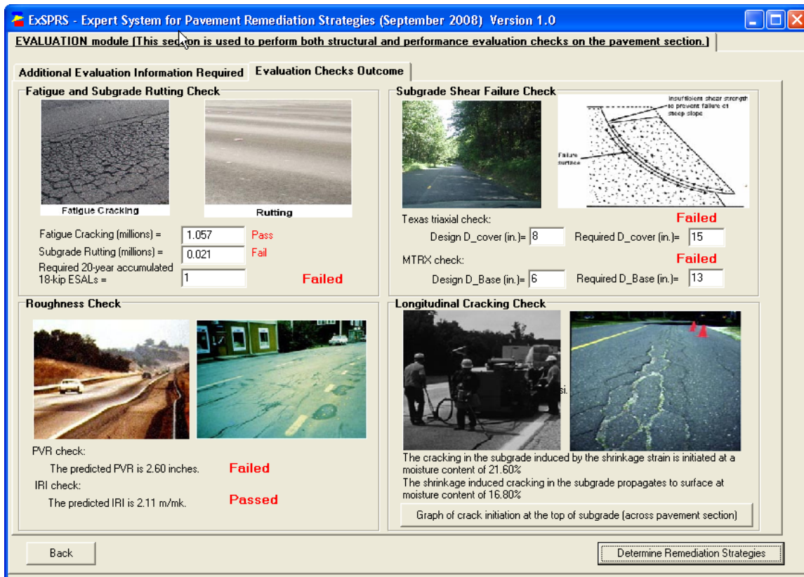
Figure 3.3—Evaluation Checks Outcome
