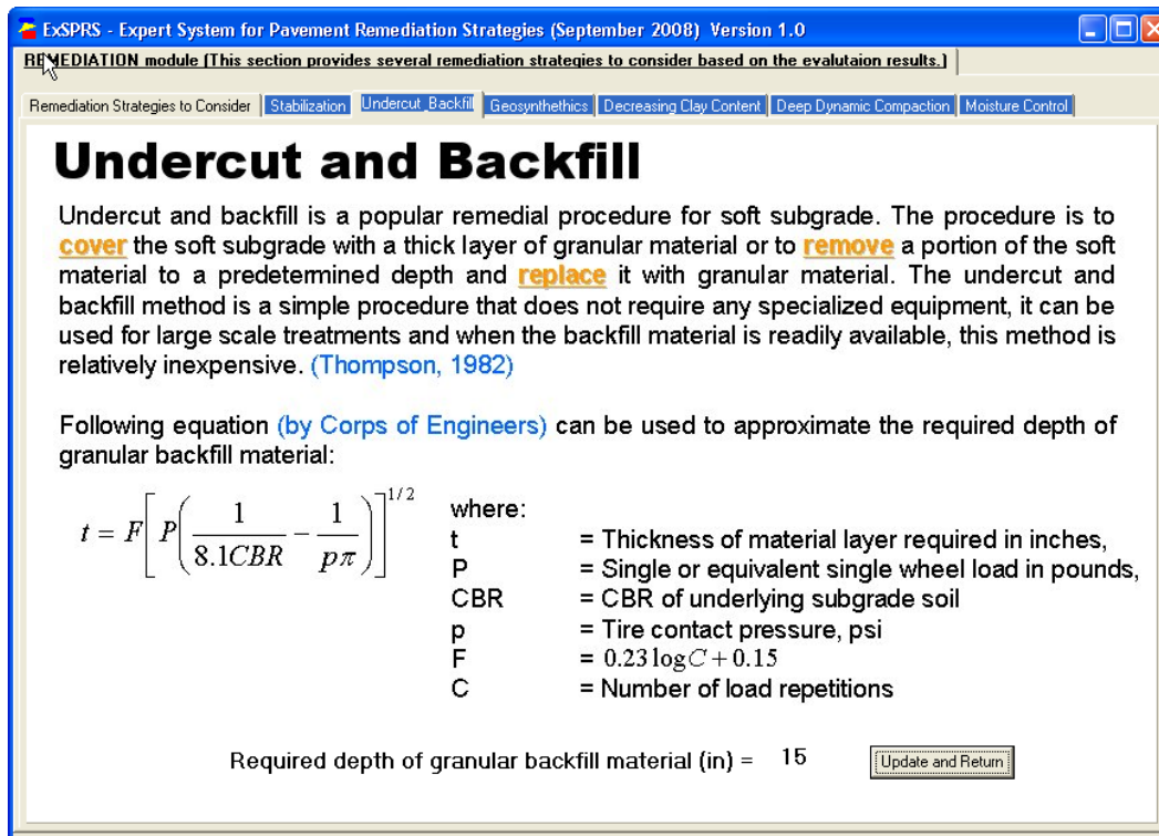
Figure 4.14—Undercut and Backfill
