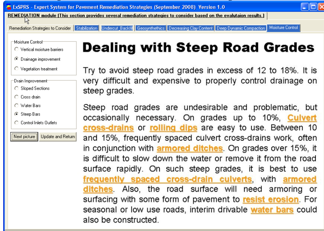
Figure 4.10—Moisture Control Method of Dealing with Steep Grades
