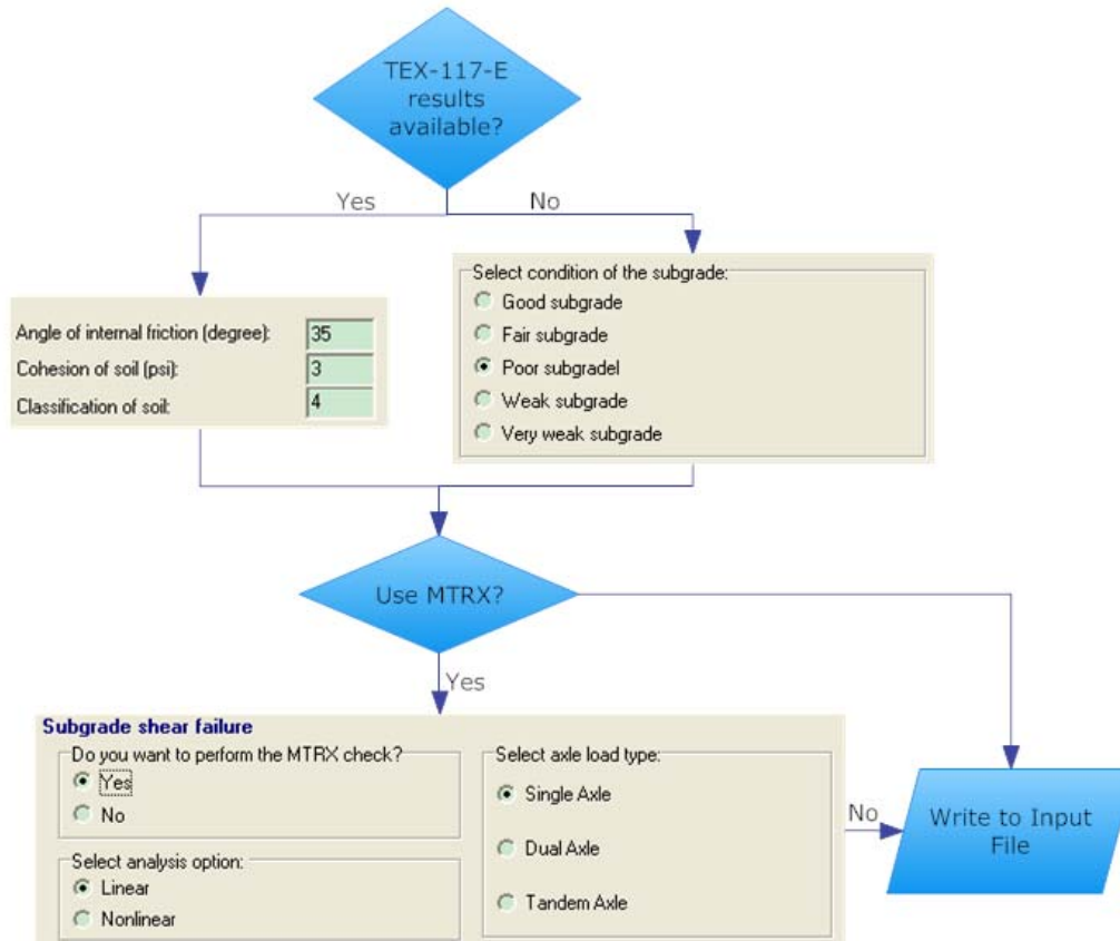
Figure 3.2—Subgrade Shear Failure Check Input Structure
