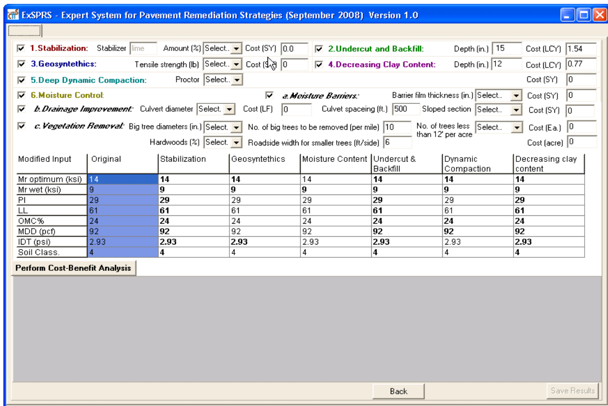
Figure 5.1—Cost and Benefit Analysis
