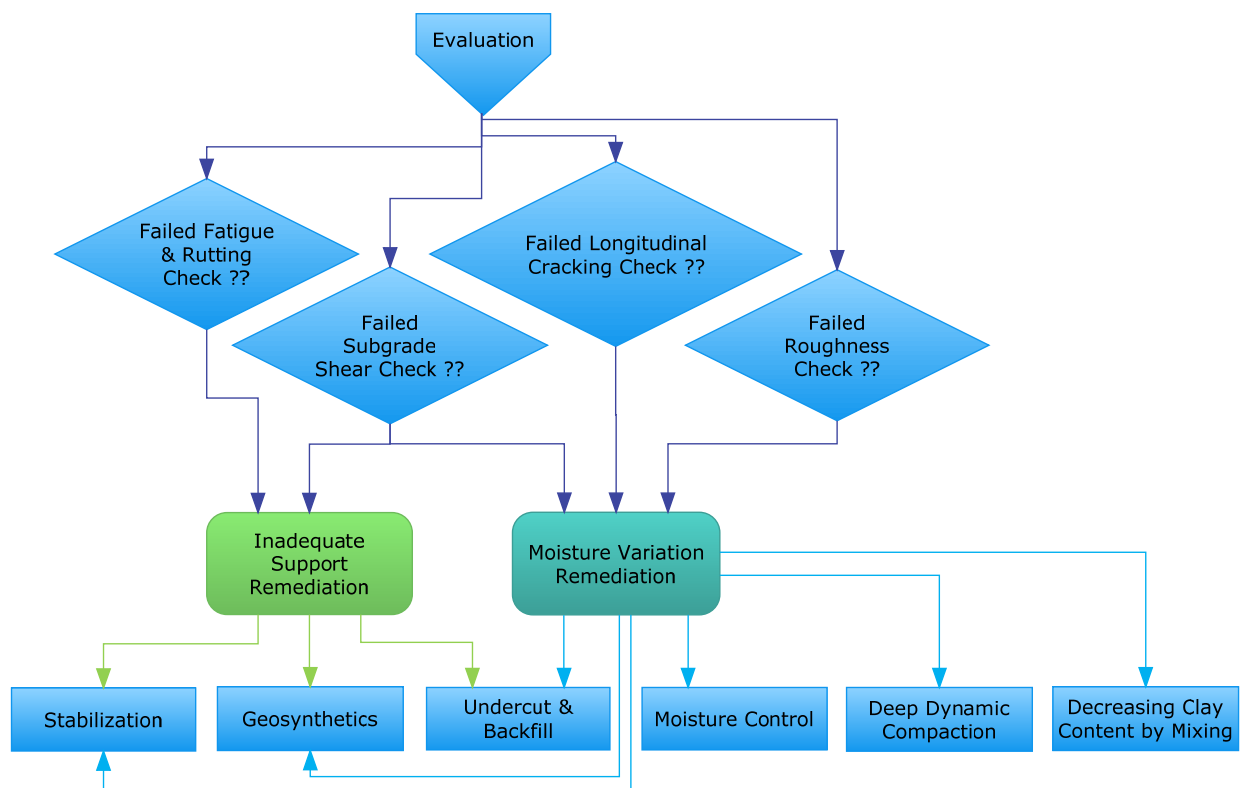
Figure 4.1— Logic Flowchart of Recommended Remediation Strategies
