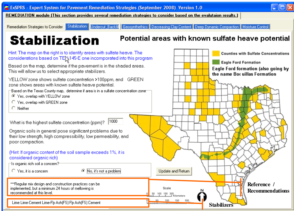
Figure 4.3—Stabilization Window of Remediation Module
