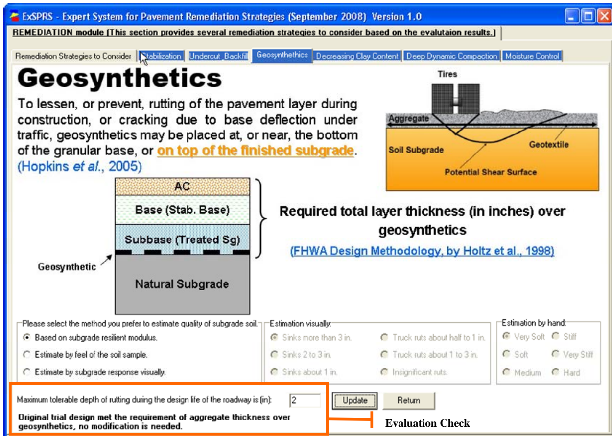
Figure 4.4—Use of Geosynthetics
