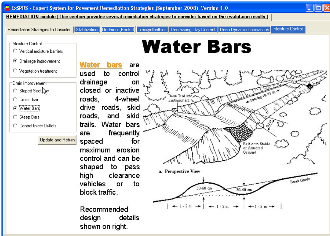
Figure 4.9—Moisture Control Method of Using Water Bars
