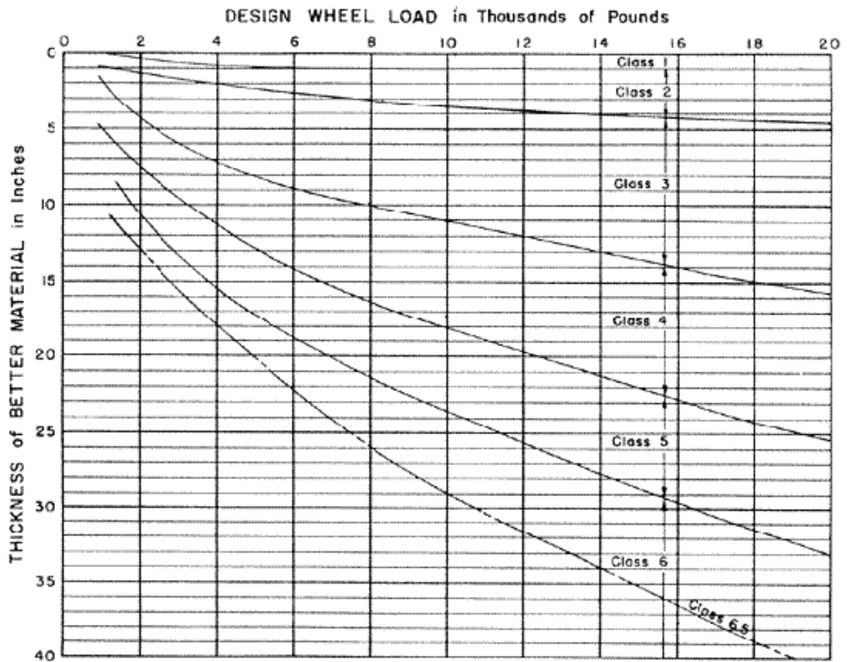
Figure 5.11— IEX-11/-E Flexible Base Design Chart
