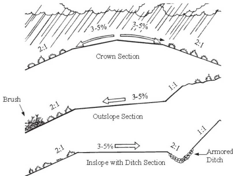
Figure 5.6—Sloped Surface Drainage Options
