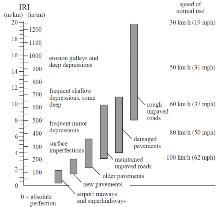
Figure 4.5—Physical Interpretation of the Open-Ended IRI Scale (Replotted from Sayers, et al., 1986)
