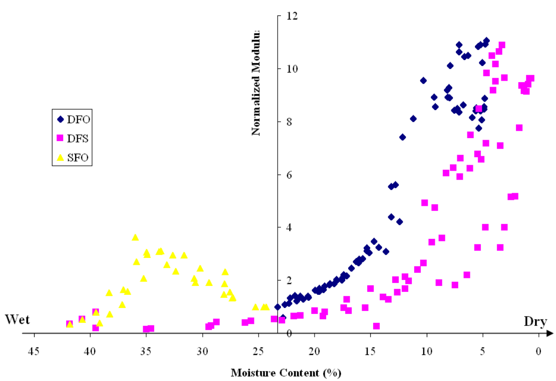
Figure 4.28—Normalized Modulus vs. Moisture Content for Different Moisture Conditioning Paths (Paris)
