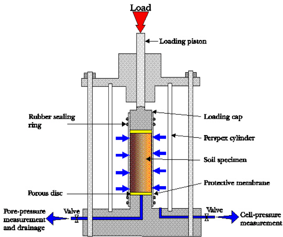
Figure 2.1—Triaxial Test Apparatus
