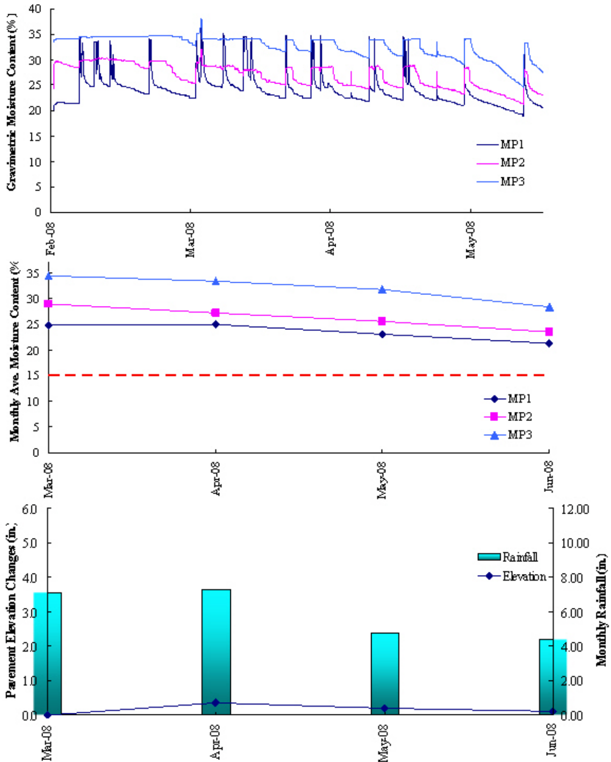
Figure E. 9— Atlanta Site Field Measurements Plot
