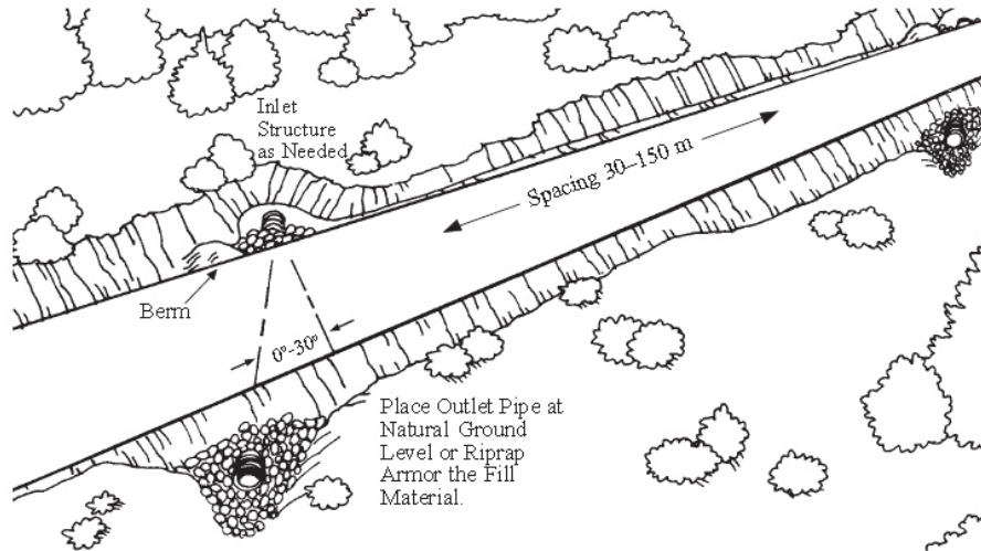
Figure 5.7—Details of Culvert Cross-Drains
