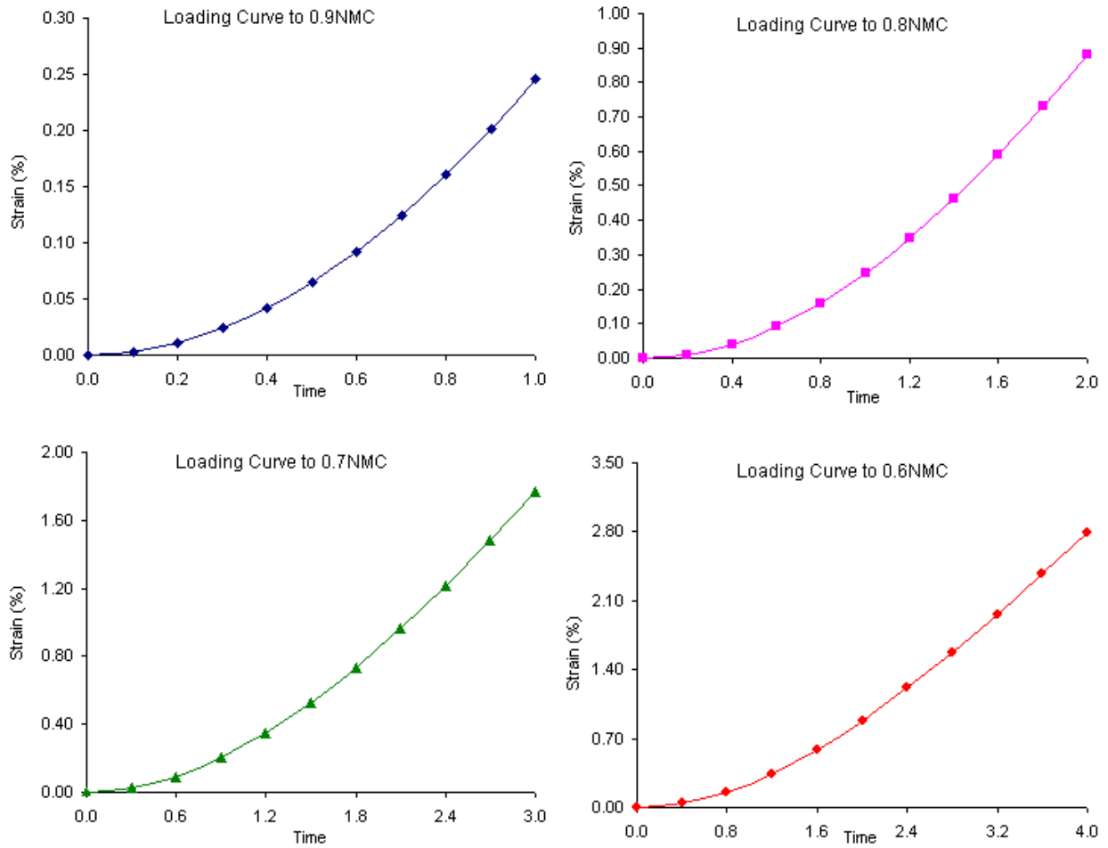
Figure C. 3—Example of Loading Curves for Fracture Model (Paris, DFO)
