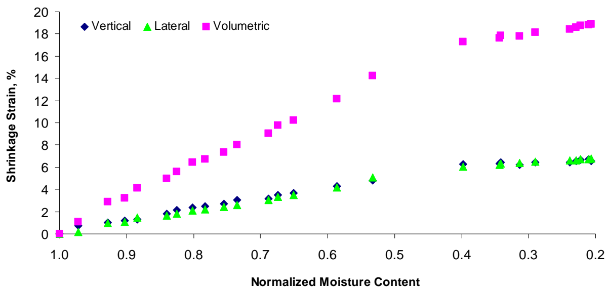
Figure 4.8—Shrinkage Strain Variations with NMC (Paris, DFO)
