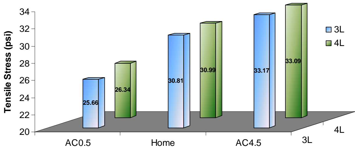
Figure D. 1— AC Layer Thickness Effects on Average of Top 50 Tensile Stresses
