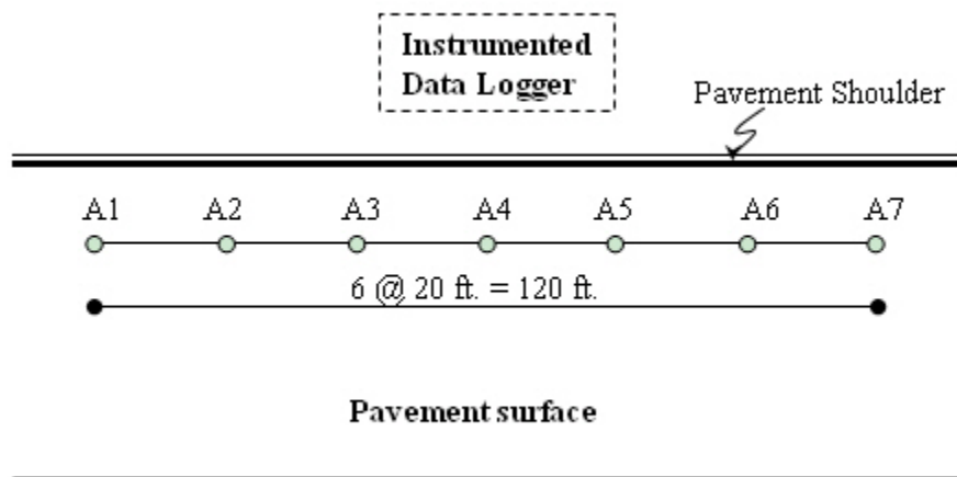
Figure 7.8—Schematic of Elevation Survey Section (by UTA)
