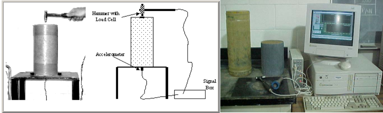
Figure 2.5—Free-Free Resonant Column System (from Nazarian and Yuan, 2003)
