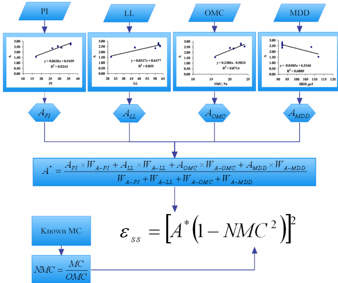
Figure 4.10—Flowchart of Shrinkage Strain Prediction Relationship Based on Index Properties
