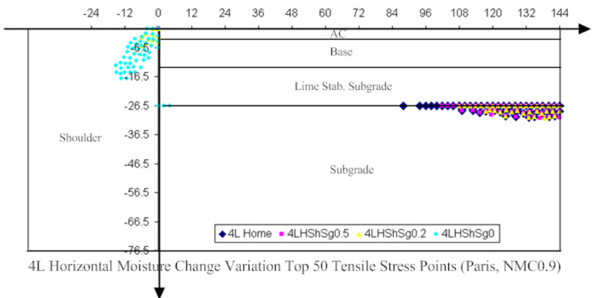
Figure D. 11—Horizontal Moisture Change Variation Effects on Top 50 Points Distribution
