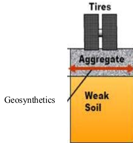
Figure 2.14—Improving Pavement by Using Geosynthetics (from Hopkins et al. , 2005)
