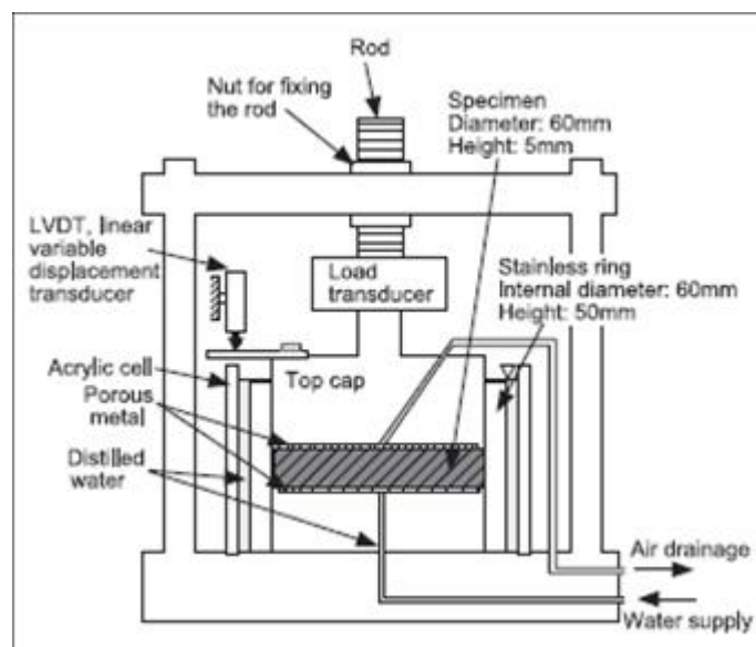
Figure 2.12—Swell Pressure Test Apparatus
