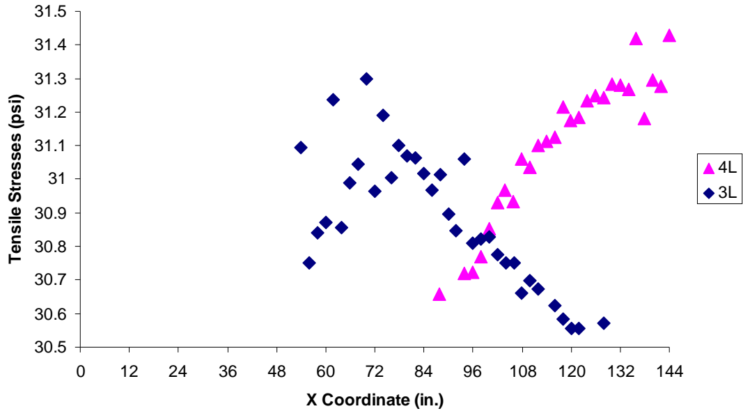
Figure 4.21—Maximum Tensile Stresses at Subgrade Top (Paris, 0.9NMC)
