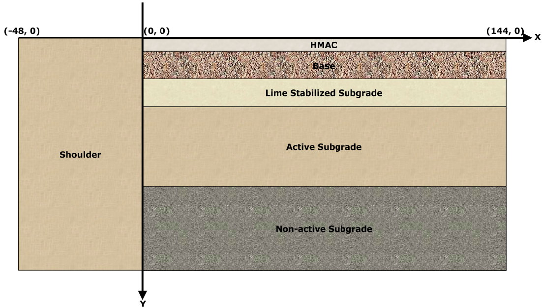
Figure 4.16—Typical Pavement Section Geometry Setup in FE Modeling
