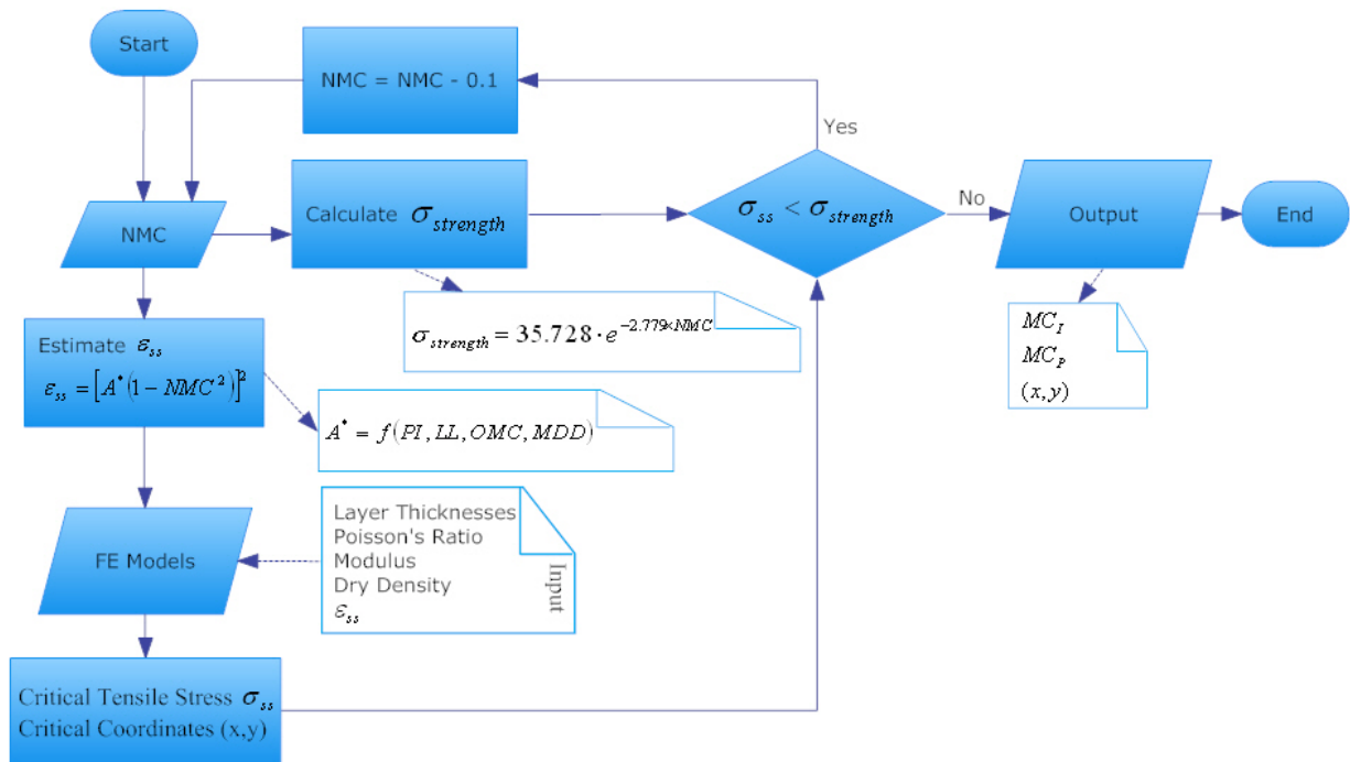
Figure 4.12—Longitudinal Shrinkage Cracking Model Algorithms
