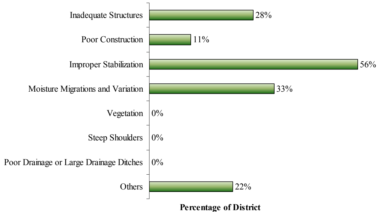
Figure 3.3—Causes for Transverse Cracking
