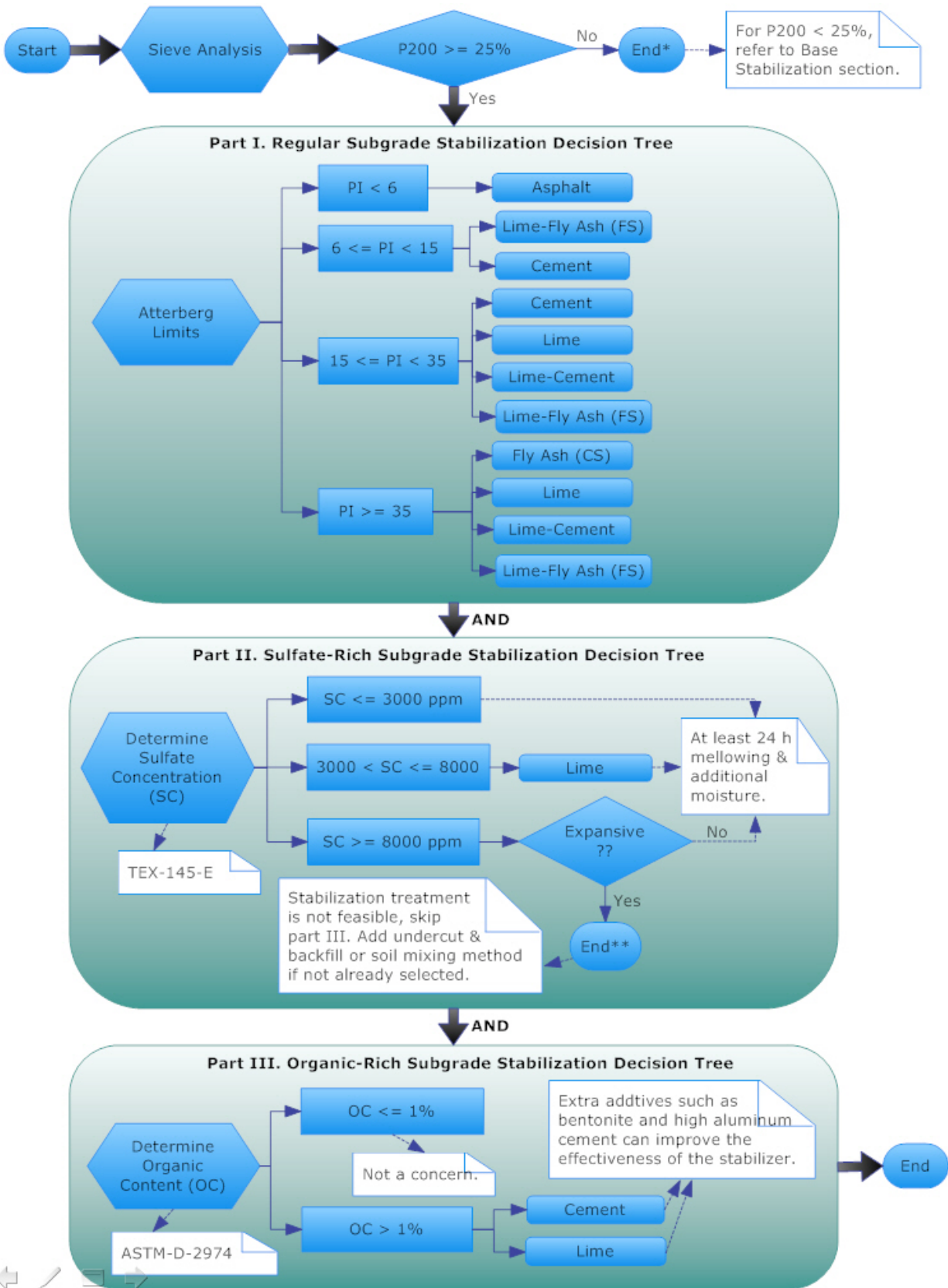
Figure 5.1—Stabilization Subroutine Flowchart
