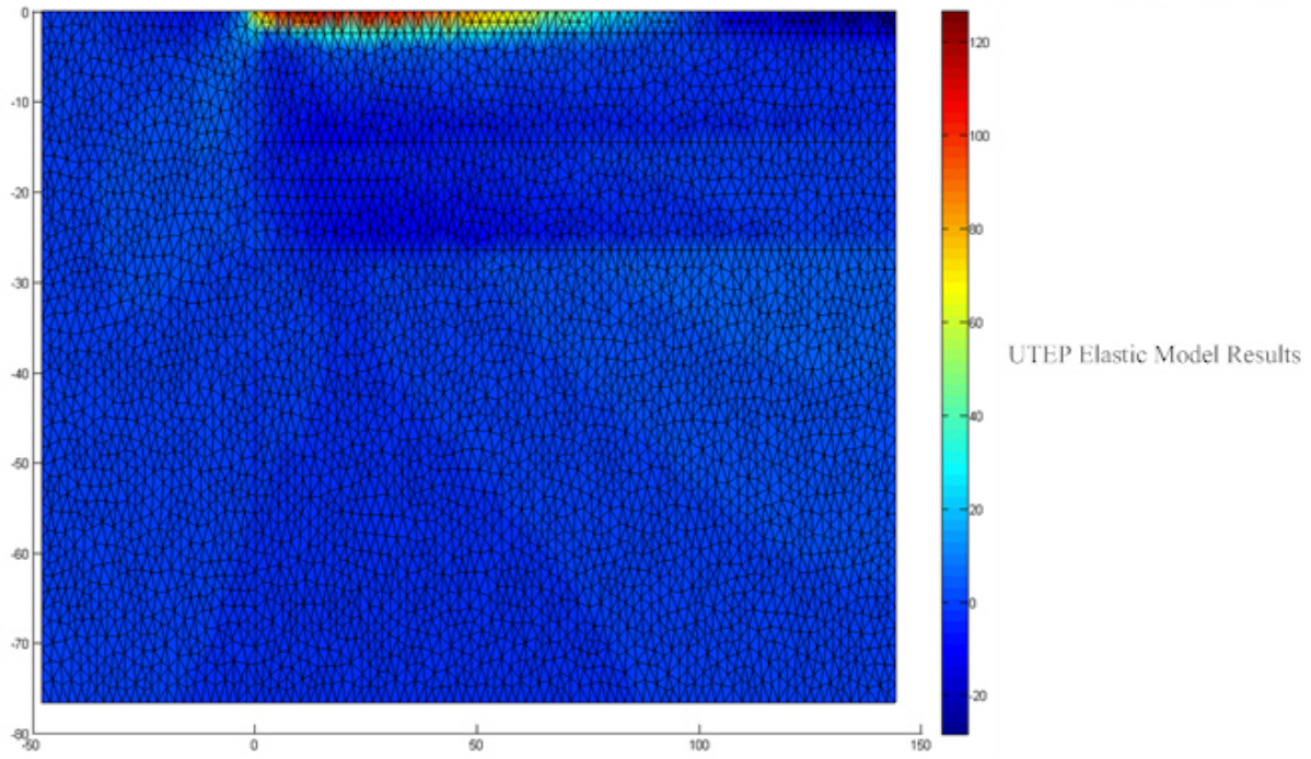
Figure 4.27—Comparisons of Tensile Stress Contours for Validation Study
