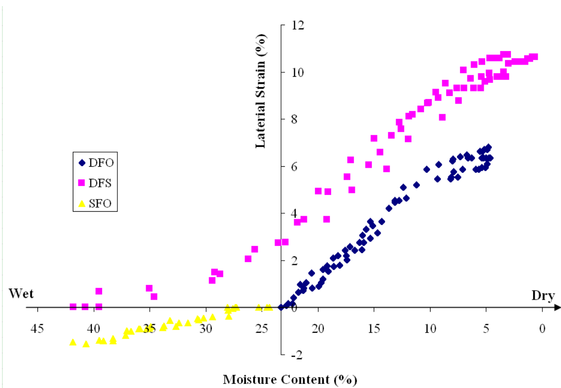
Figure 4.29—Lateral Strain vs. Moisture Content for Different Moisture Conditioning Paths (Paris)
