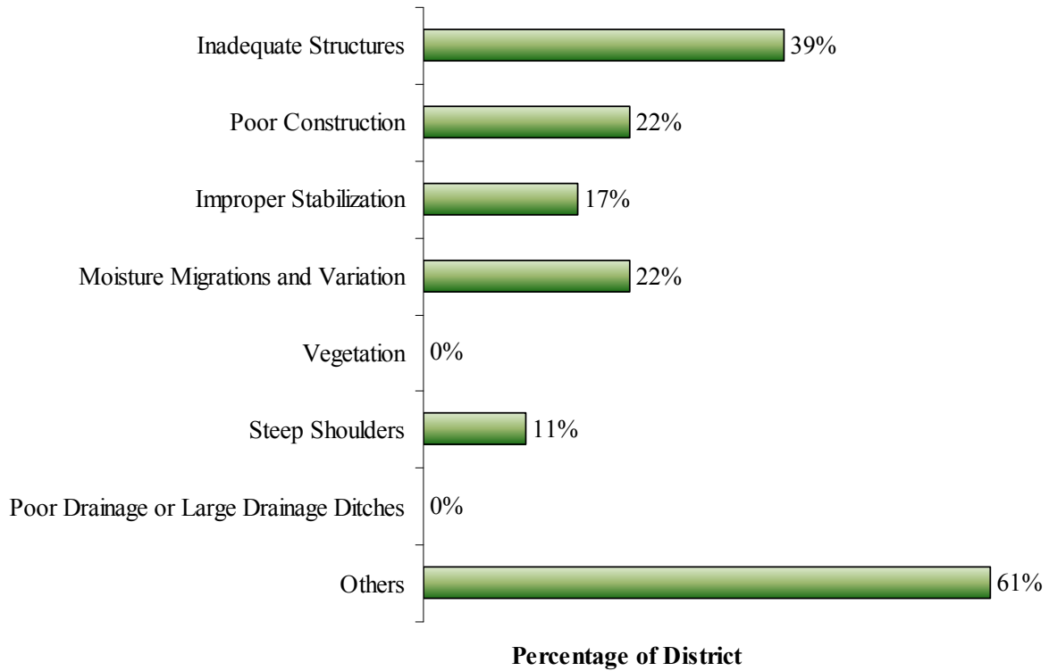
Figure 3.5—Causes for Shoving
