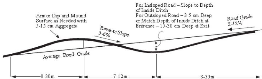
Figure 5.8—Details of Rolling Dip Cross-Drains
