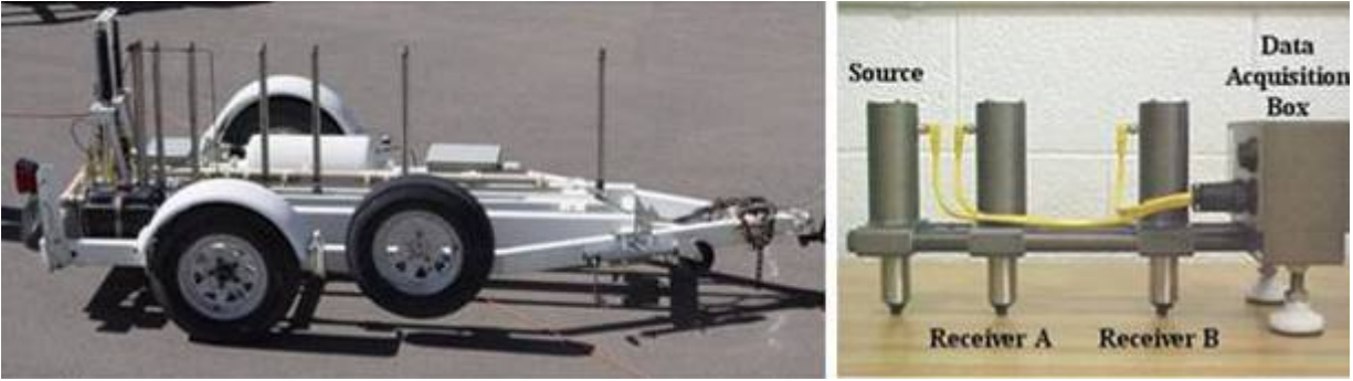
Figure 2.10—Photograph of SPA (left) and PSPA Sensors (right)
