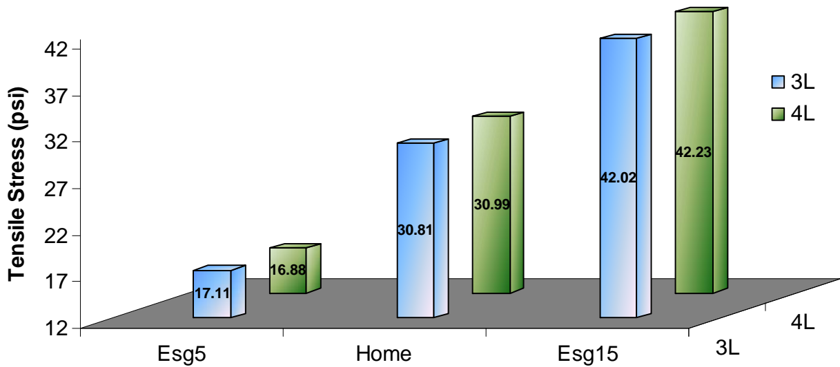
Figure D. 6— Subgrade Layer Modulus Effects on Average of Top 50 Tensile Stresses
