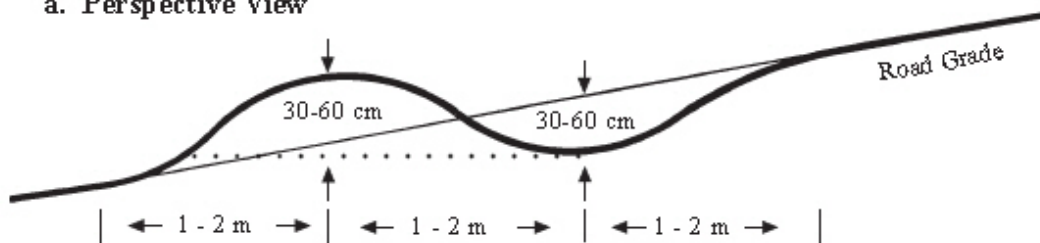
Figure 5.9—Details of Water Bars
