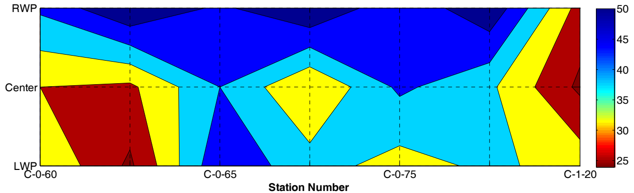
Figure D.5 – Contour Maps of Field Seismic Modulus of Medium PI Pharr Sites after 24 Hours of Compaction
