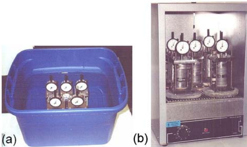
Figure 2.12 – Wet (a) and Dry Cycles Setup Used by Hoyos et al. (2005)
