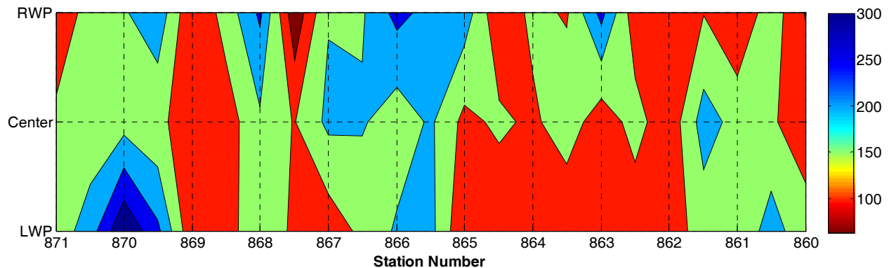
Figure D.4 – Contour Maps of Field Seismic Modulus of Wichita Falls after 3 Days of Compaction
