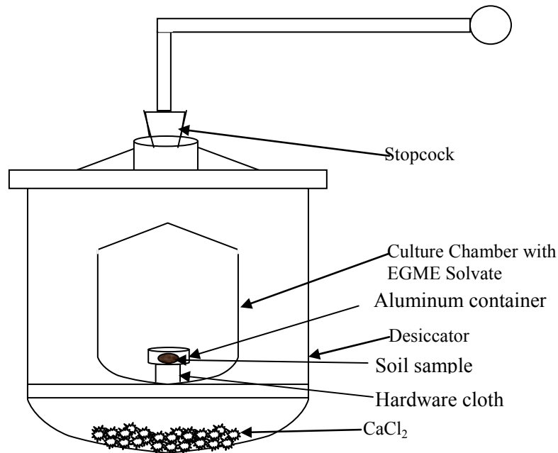
Figure C.2 – Schematic of the Specific Surface Area Apparatus
