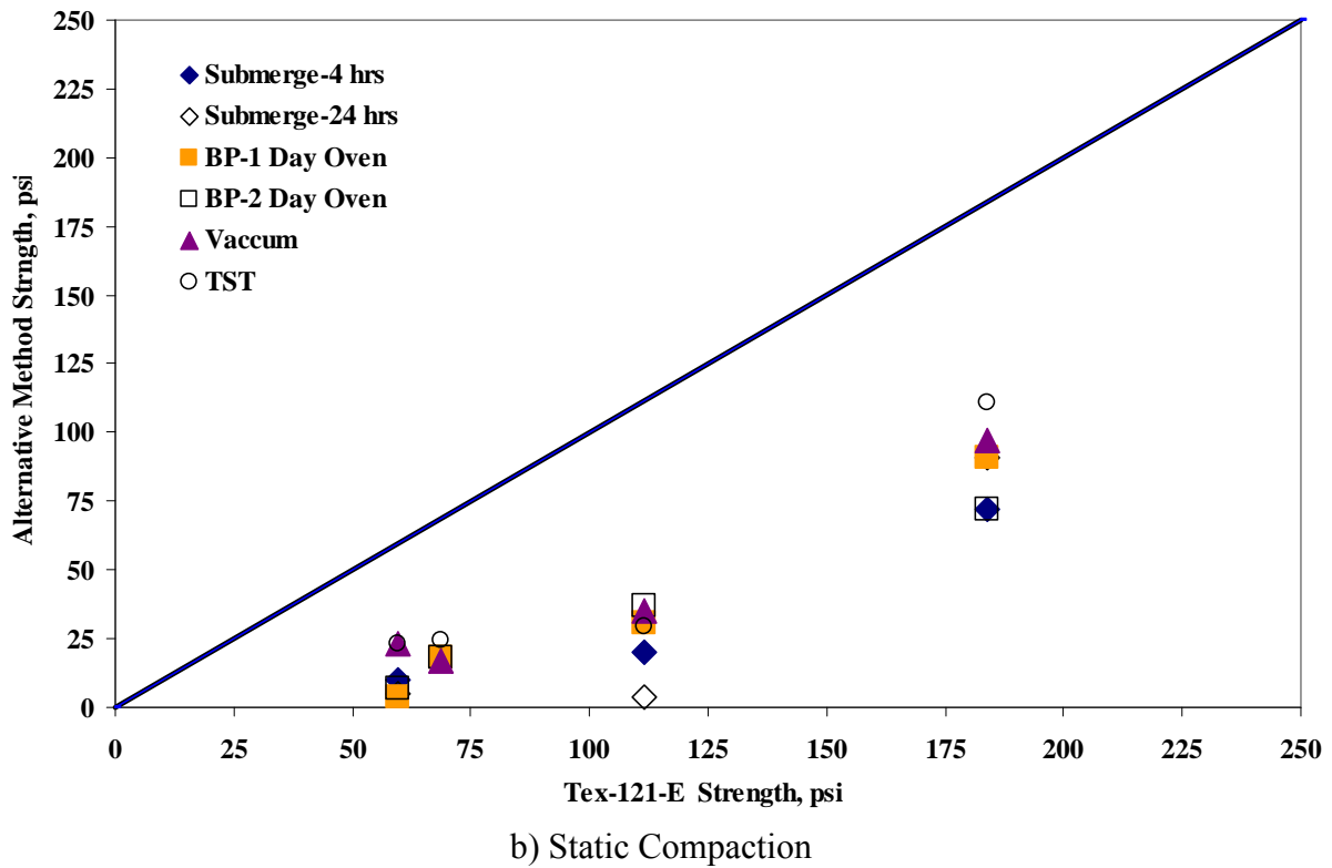
Figure 4.25 – Comparison of Strengths from Tex-121-E with Other Moisture Conditioning Methods
