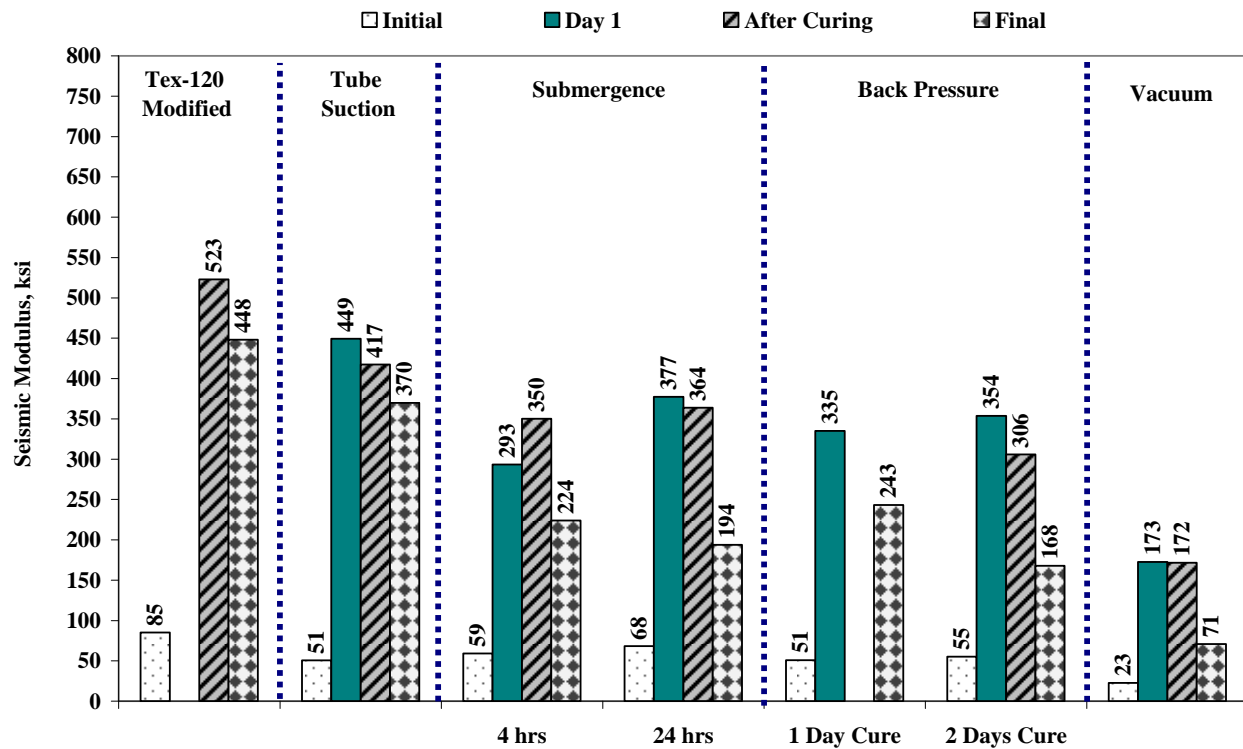
Figure 4.35 – Seismic Modulus Results of Moisture Conditioning Tests for Wichita Falls Material
