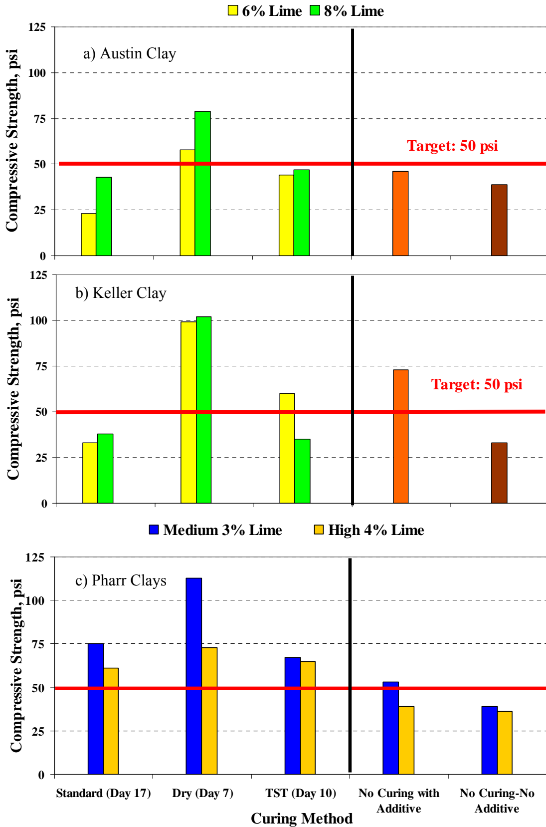
Figure 6.2 – Unconfined Compressive Strength Results for Soil-lime Specimens
