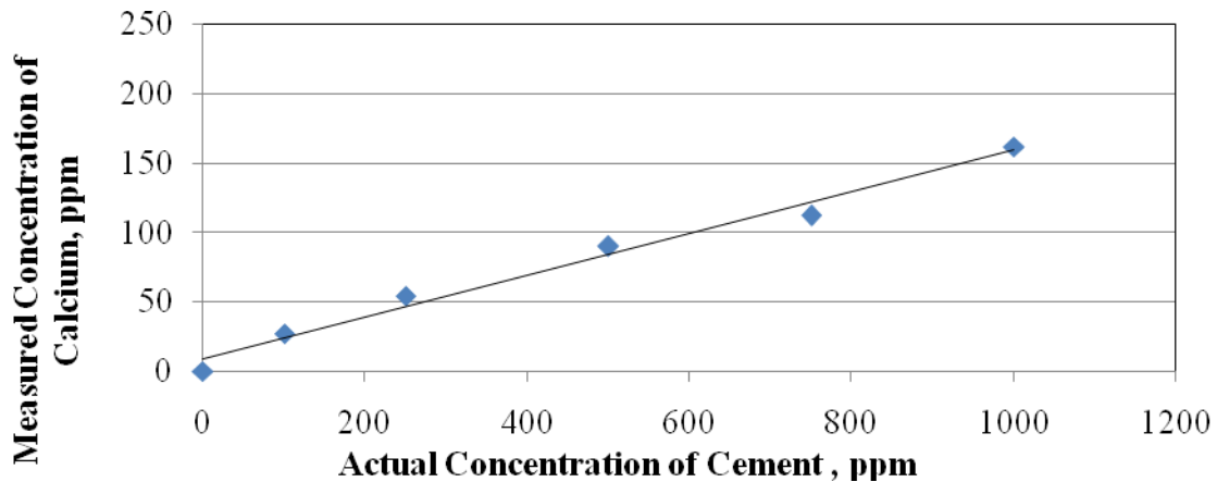
Figure 5.7 – Calibration Curve for Obtaining the Concentration of Cement from Concentration of Ca
