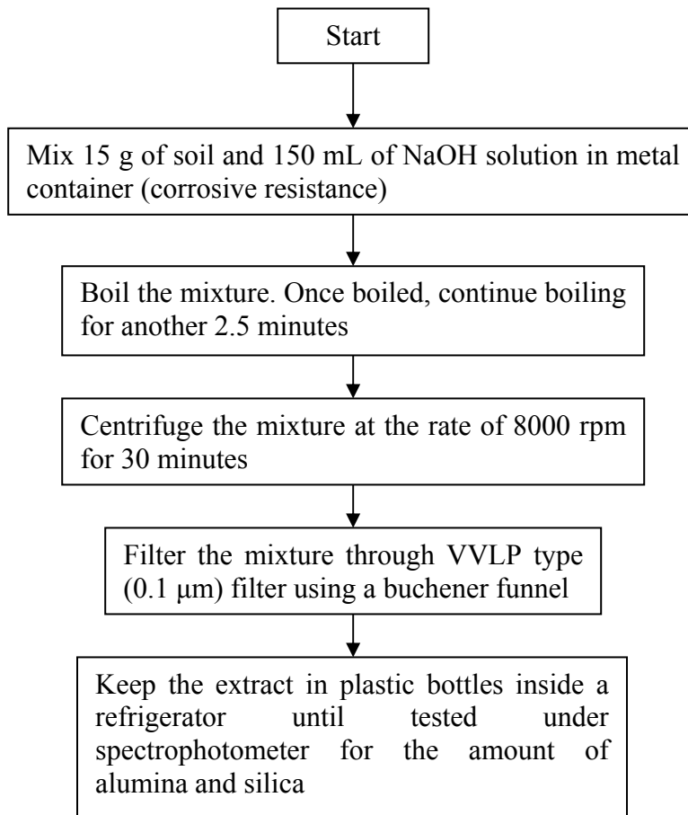
Figure C.1 – Flow Chart Showing the Test Procedure Followed for the Determination of Reactive Alumina and Silica
