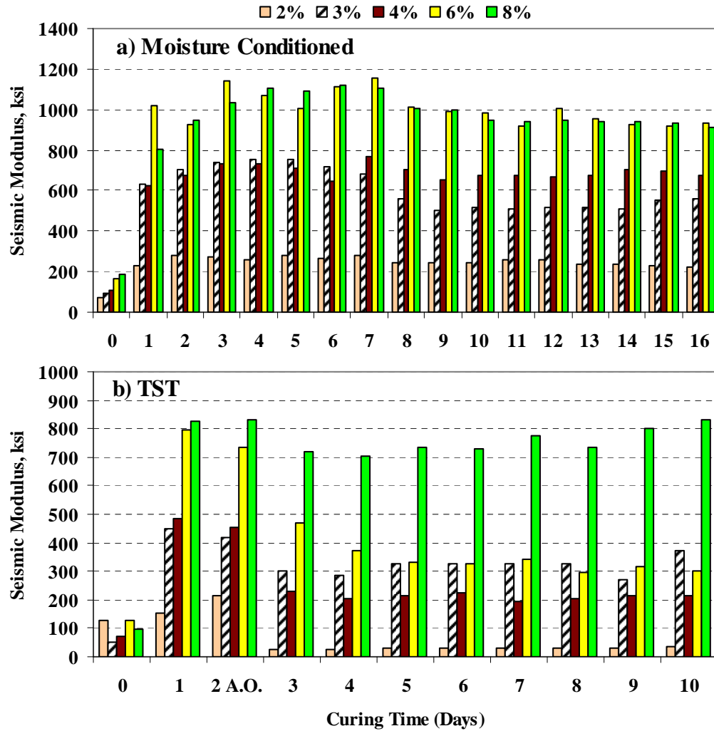
Figure 3.12 – FFRC Seismic Modulus Results for Wichita Falls Soil–Cement Specimens
