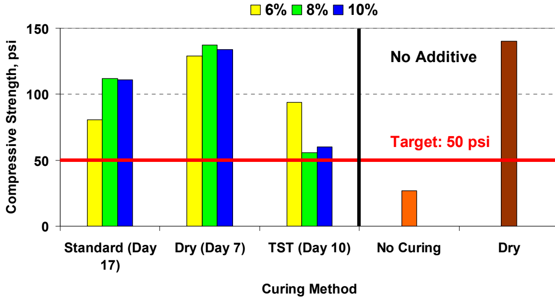
Figure 3.2 – Unconfined Compressive Strength Results for El Paso Soil-Lime Specimens
