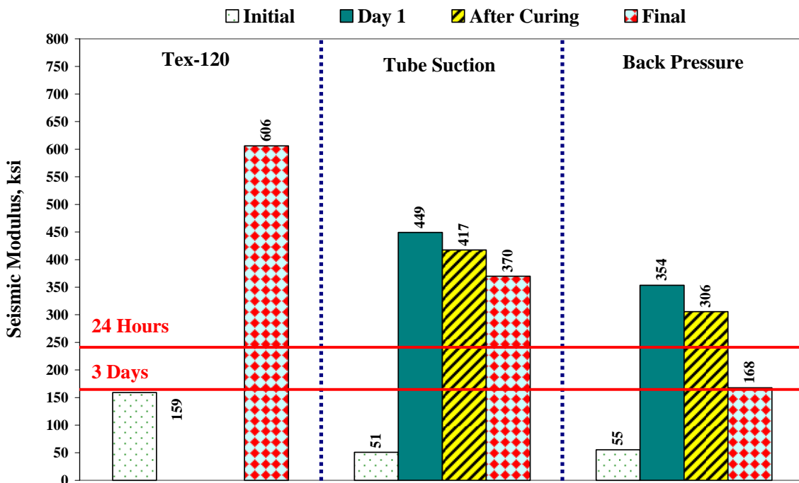
Figure 6.19 – Seismic Modulus Variation of Laboratory and Field Tests for Wichita Falls Site
