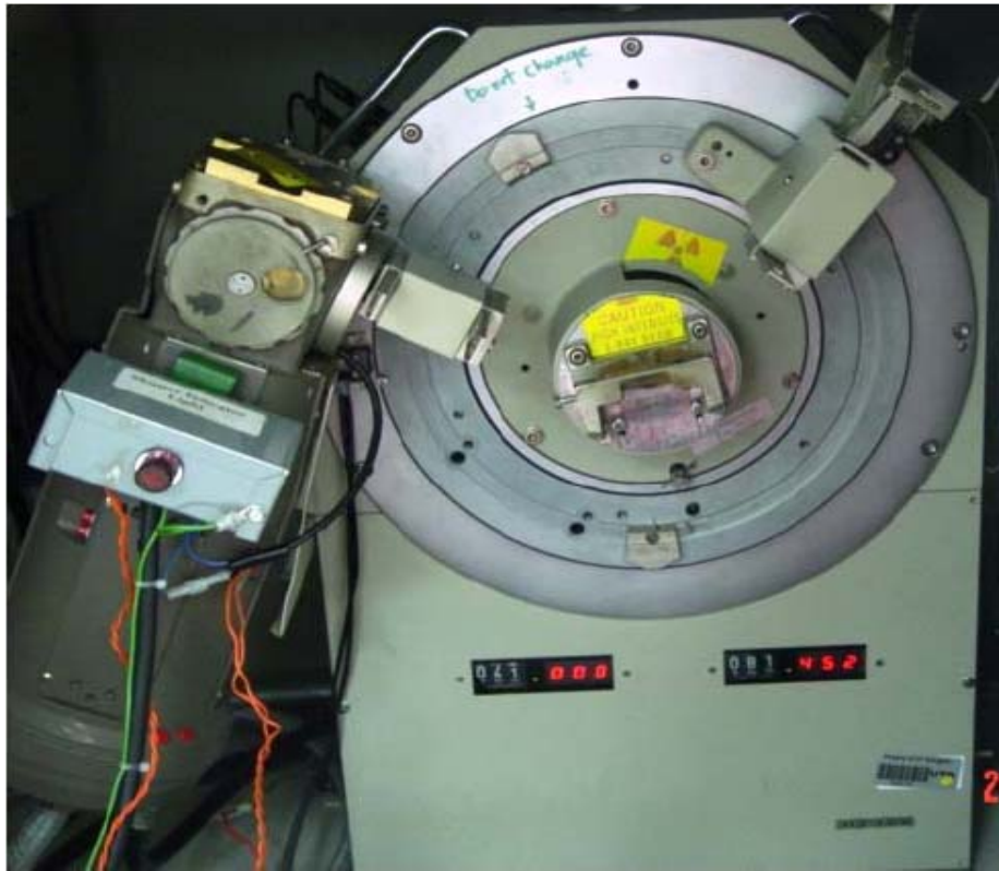
Figure 3.15 – Siemens D-500 X-Ray Diffractometer
