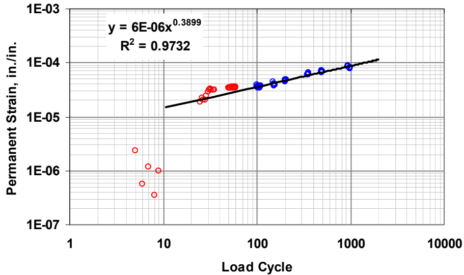
Figure 3.5 – Permanent Deformation Results for El Paso Lime Specimens with 8% Lime
