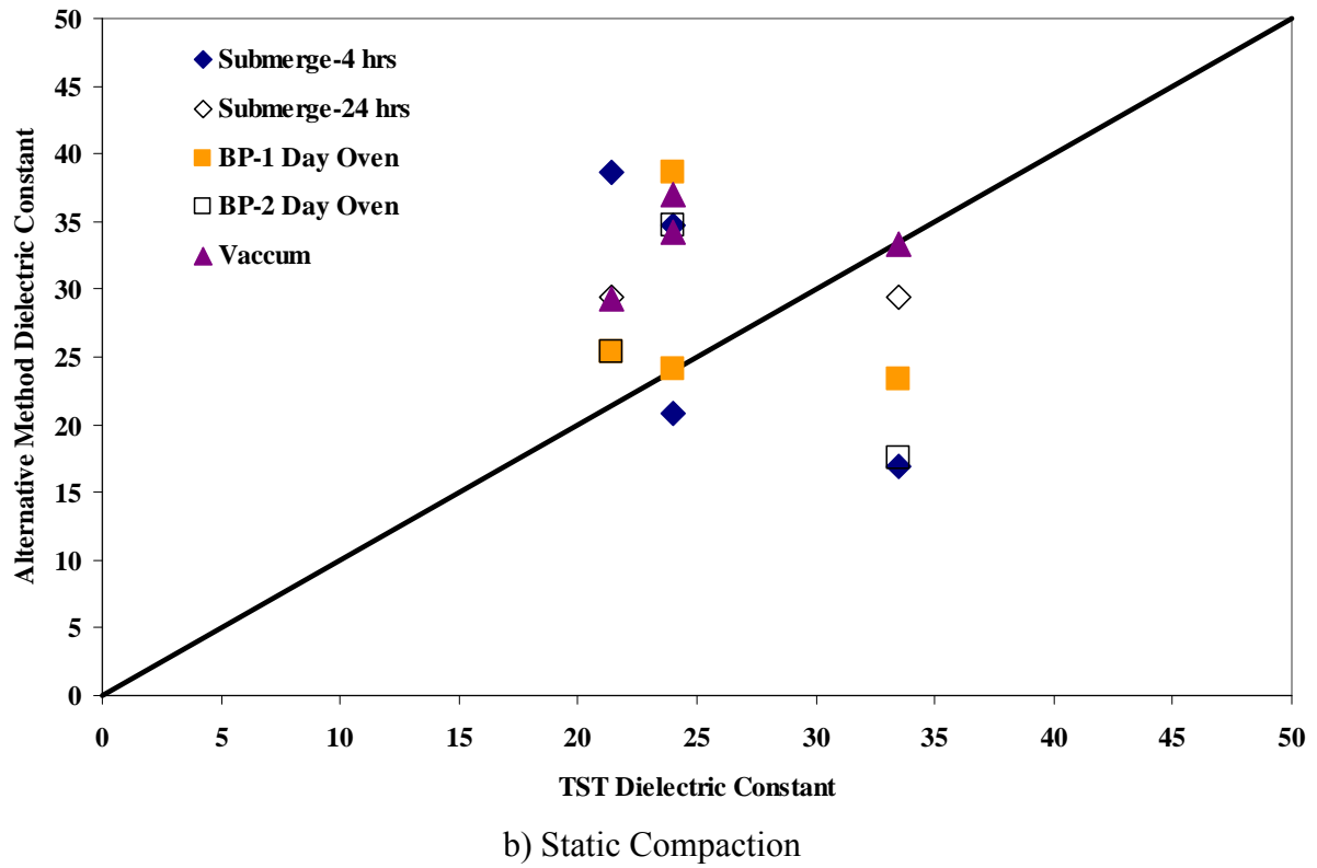
Figure 4.32 – Comparison of Dielectric Constants from TST Protocol with Other Moisture Conditioning Methods
