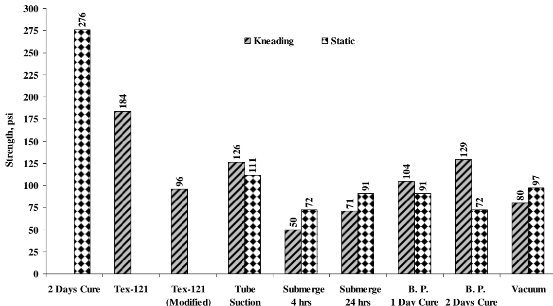
Figure 4.13 – Variations in Conditioned Unconfined Compressive Strengths for Different Moisture Conditioning Processes
