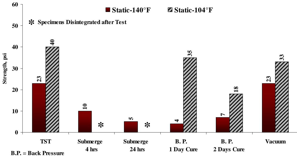
Figure 4.22 – Strength Results on Saturated Specimens for Different Curing Temperatures
