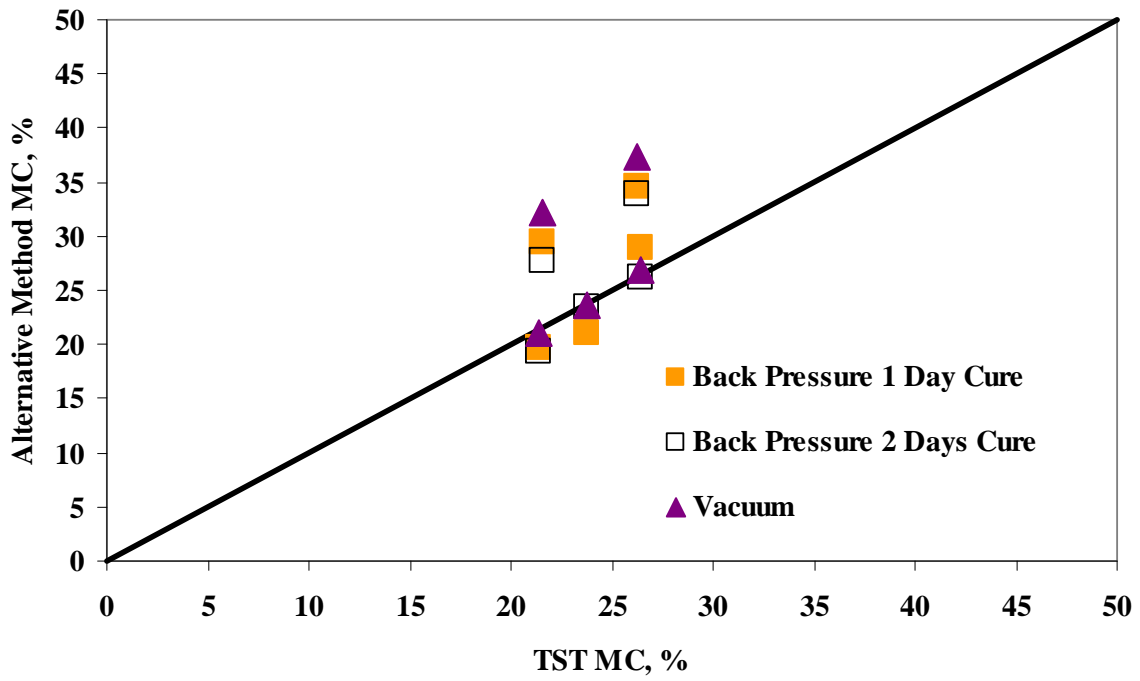
Figure 6.6 – Comparison of Moisture Contents from Different Moisture Conditioning Methods
