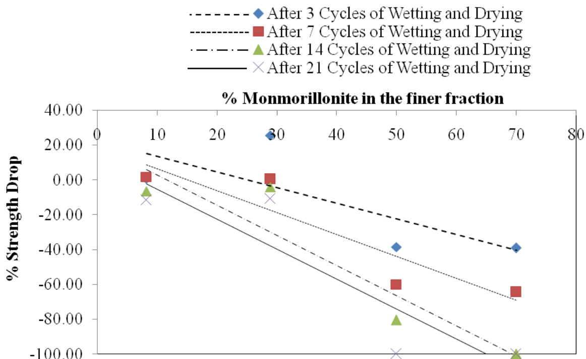
Figure 5.16 – Percentage Drop in Strength Variation with Percentage of Montmorillonite in Different Soils for Wetting Drying Cycles
