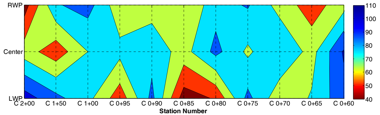
Figure D.6 – Contour Maps of Field Seismic Modulus of Medium PI Pharr Sites after 5 Days of Compaction
