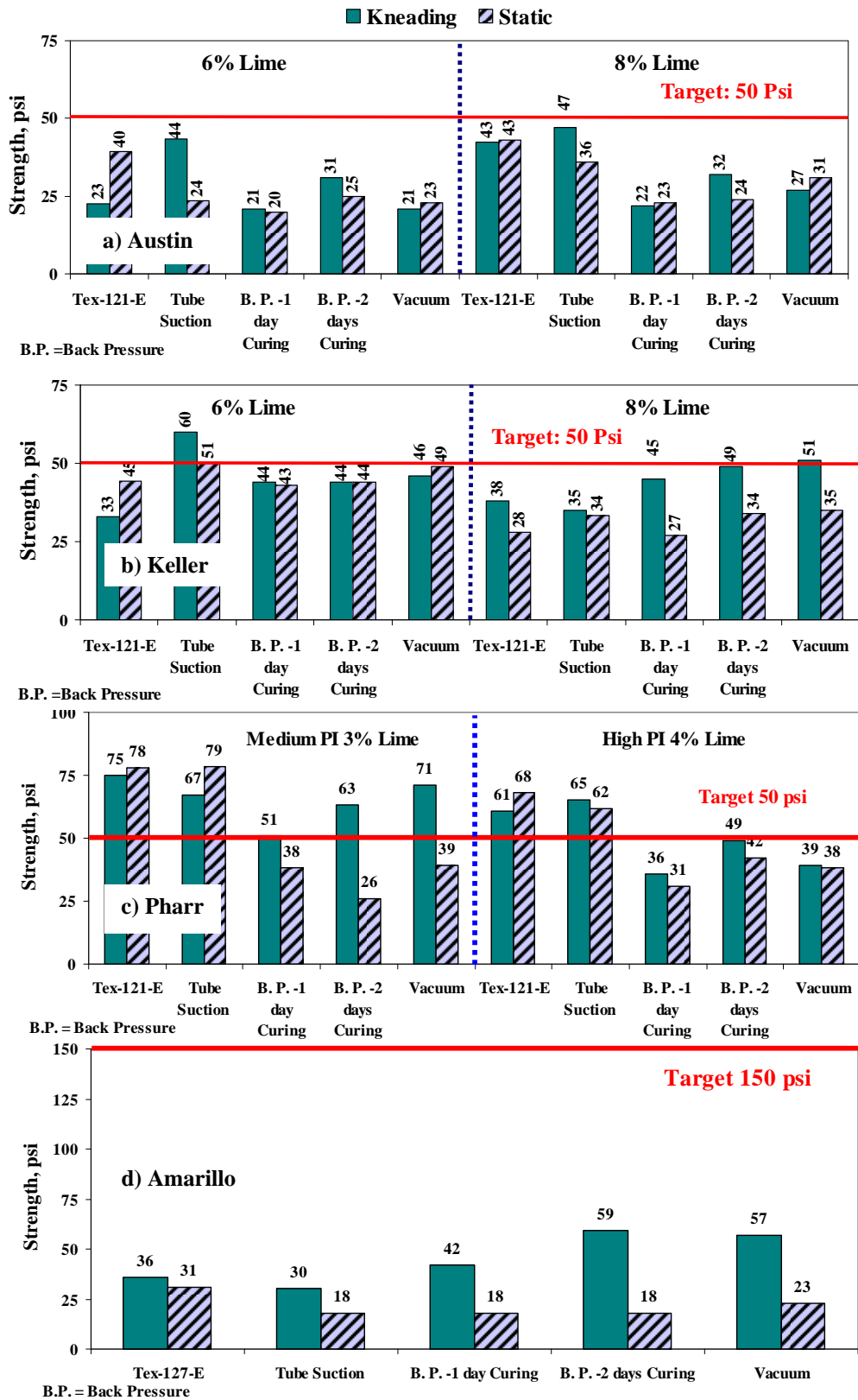
Figure 6.4 – Variations in UCS for Different Moisture Conditioning Processes
