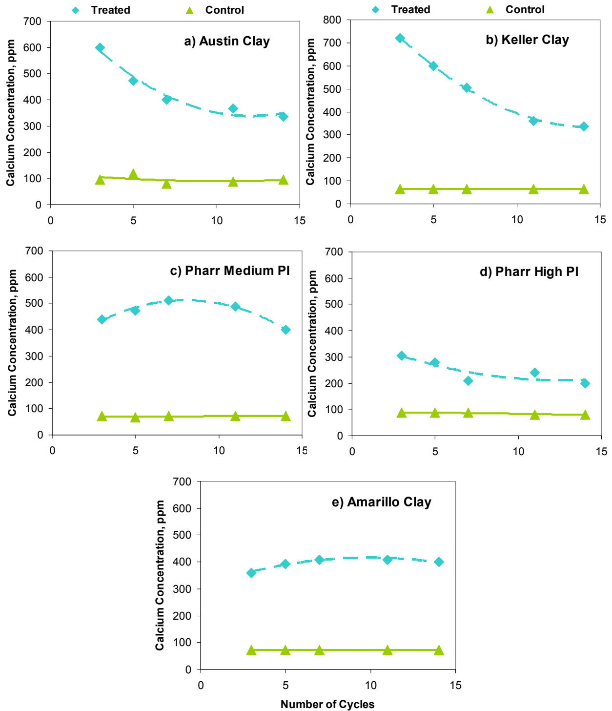
Figure 6.8 – Variation of Calcium Concentration of Validation Soil Samples
