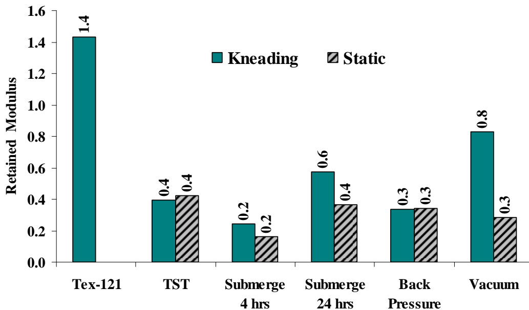
Figure 4.15 – Retained Moduli between Specimens after Moisture Conditioning and after Curing Period
