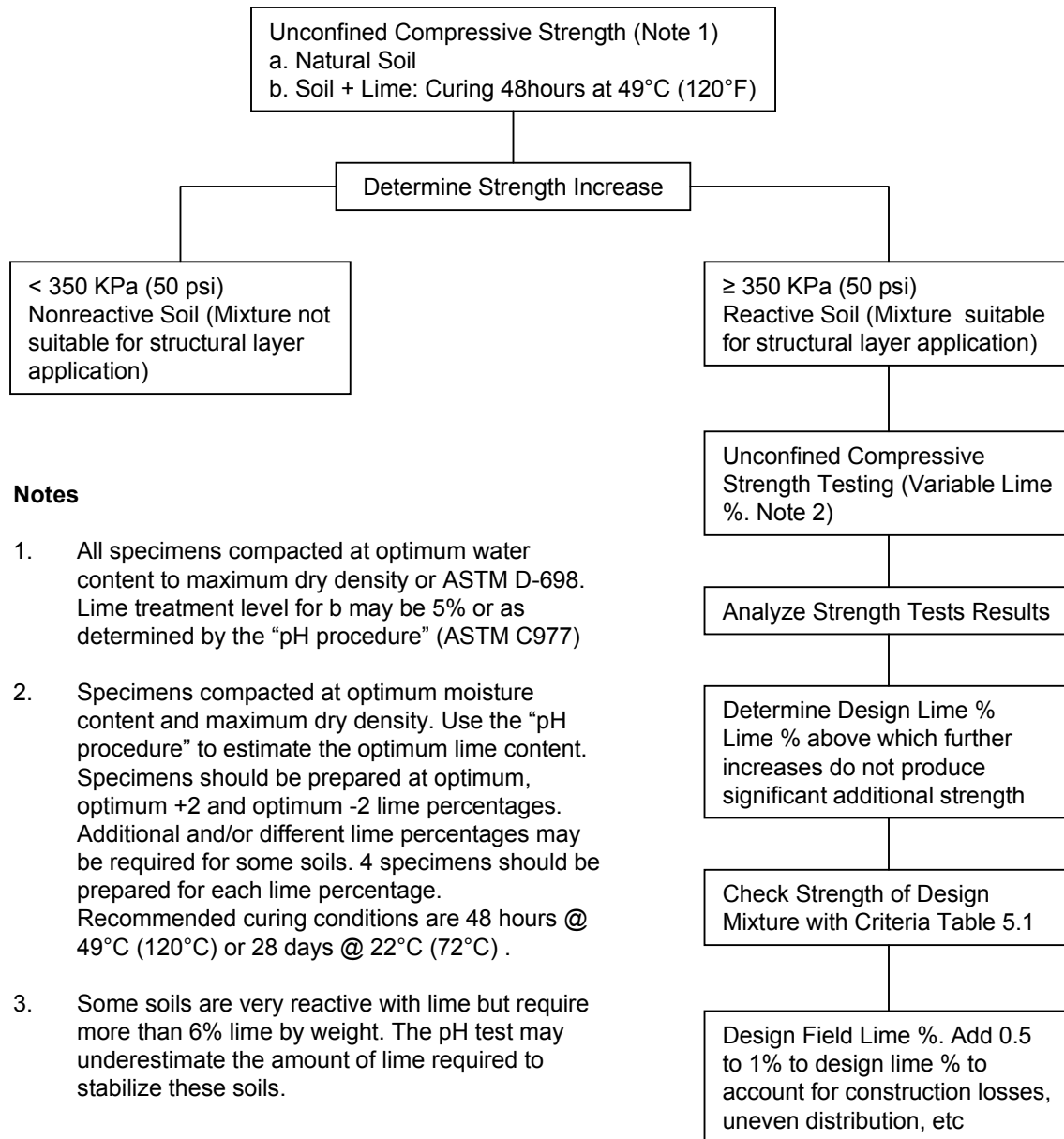
Figure 2.8 – Thompson Mixture Design Flow Chart (after Little et al., 1987)
