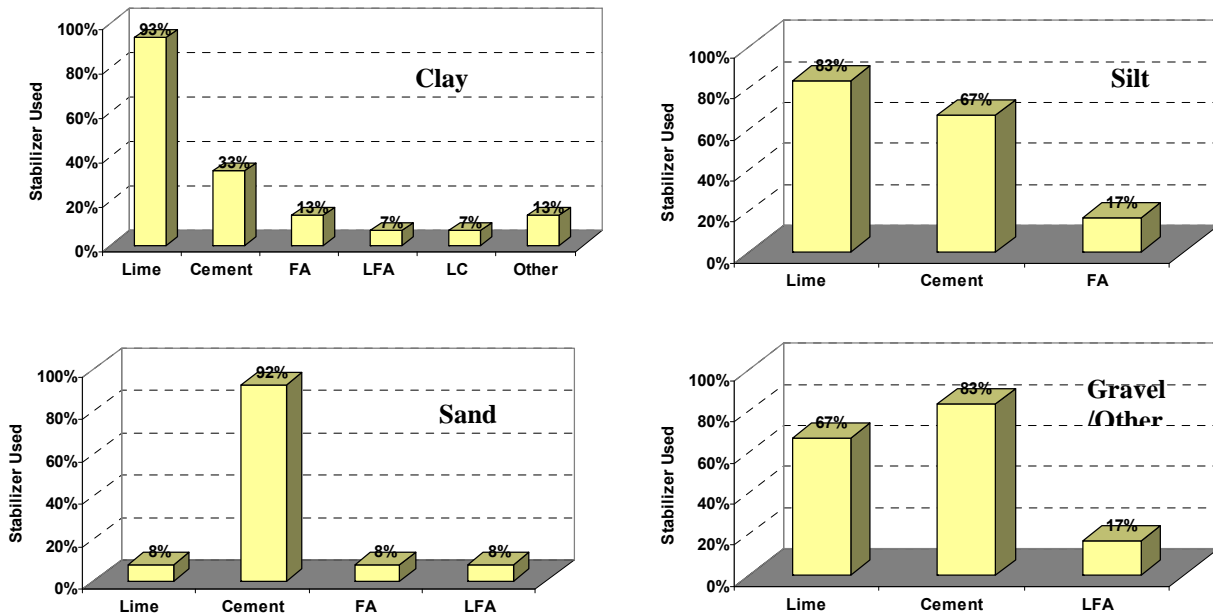
Figure A.5 – Distribution of Stabilization Types for Subgrade Types in State
