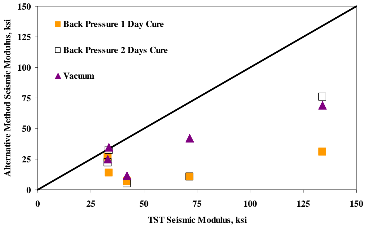
Figure 6.7 – Comparison of Moduli from Different Moisture Conditioning Methods
