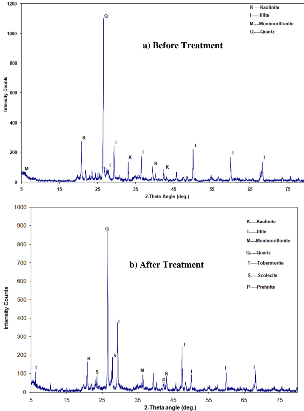
Figure 3.16 – XRD Results of El Paso Soil
