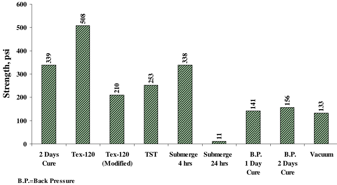
Figure 4.33 – Strength Results of Moisture Conditioning Tests for Wichita Falls Material
