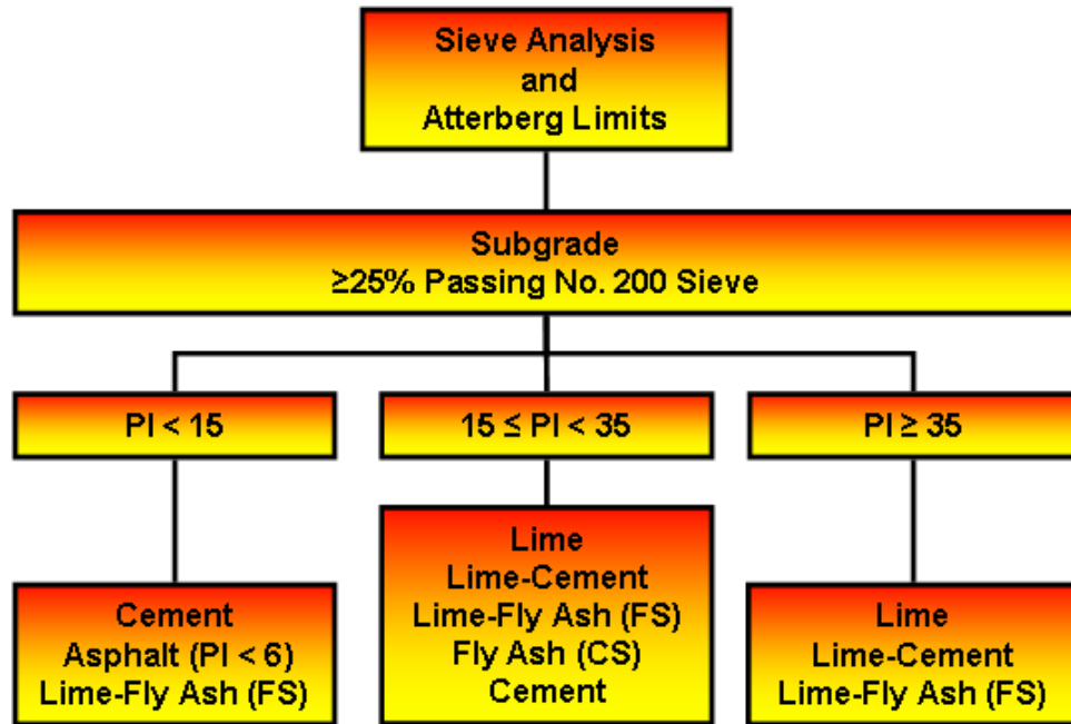
Figure 2.3 – Additive Selection Criteria for Subgrade Material Using Soil Classification
