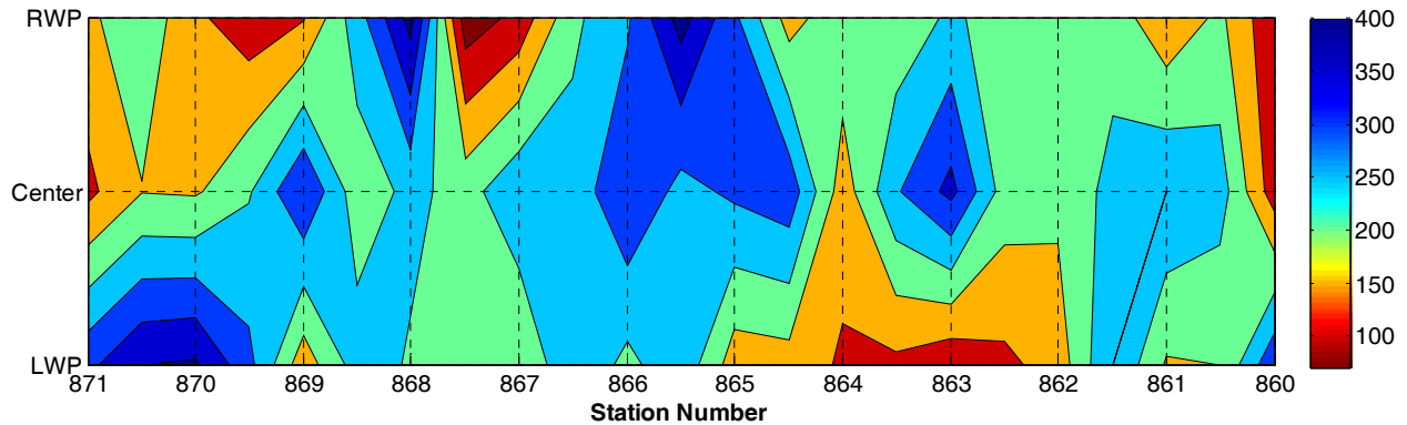
Figure D.3 – Contour Maps of Field Seismic Modulus of Wichita Falls after 24 Hours of Compaction
