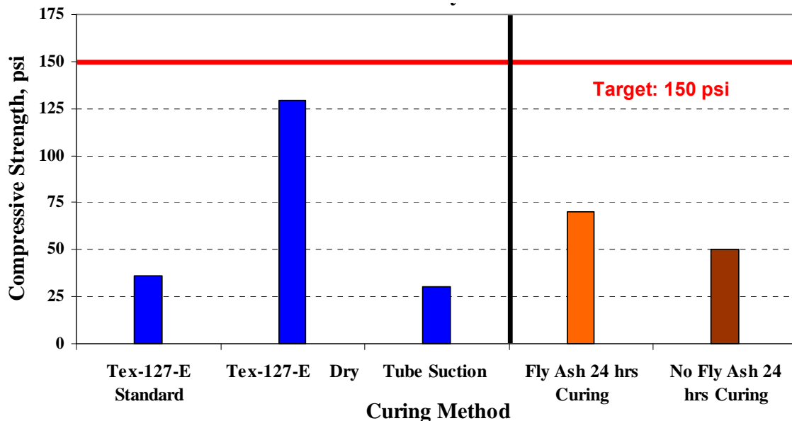
Figure 6.3 – Strength Results for Amarillo Specimens
