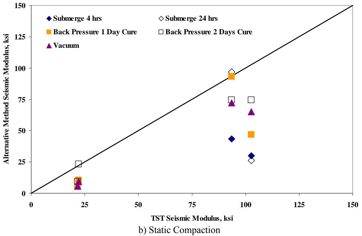
Figure 4.31 – Comparison of Moduli from TST Protocol with Other Moisture Conditioning Methods
