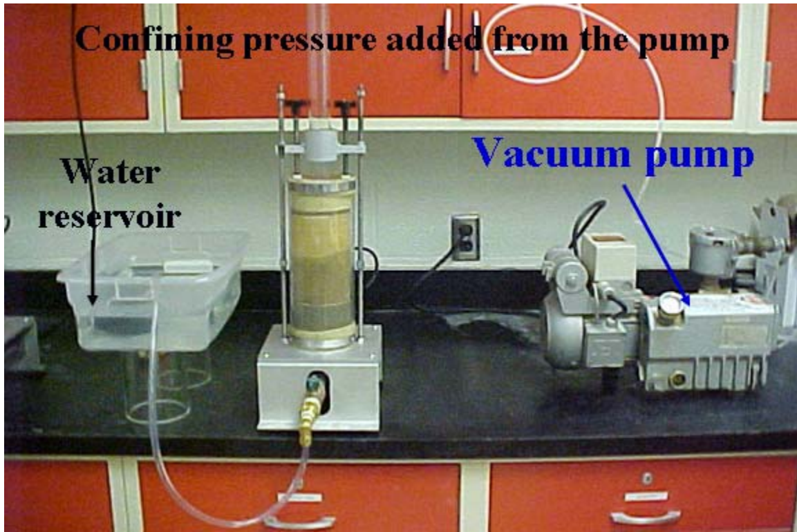
Figure 4.9 – Vacuum Test Setup
