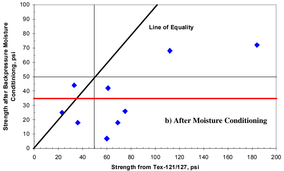
Figure 6.12 – Comparison of TxDOT Specifications Strength with Accelerated Methods
