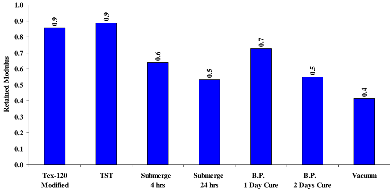
Figure 4.36 – Seismic Moduli Ratios between Specimens after Moisture Conditioning and after Curing Period
