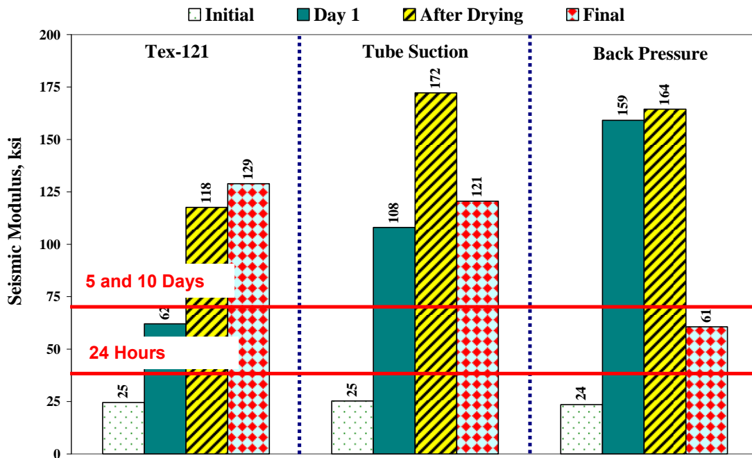
Figure 6.20 – Seismic Modulus Variation of Laboratory and Field Tests for Pharr Site
