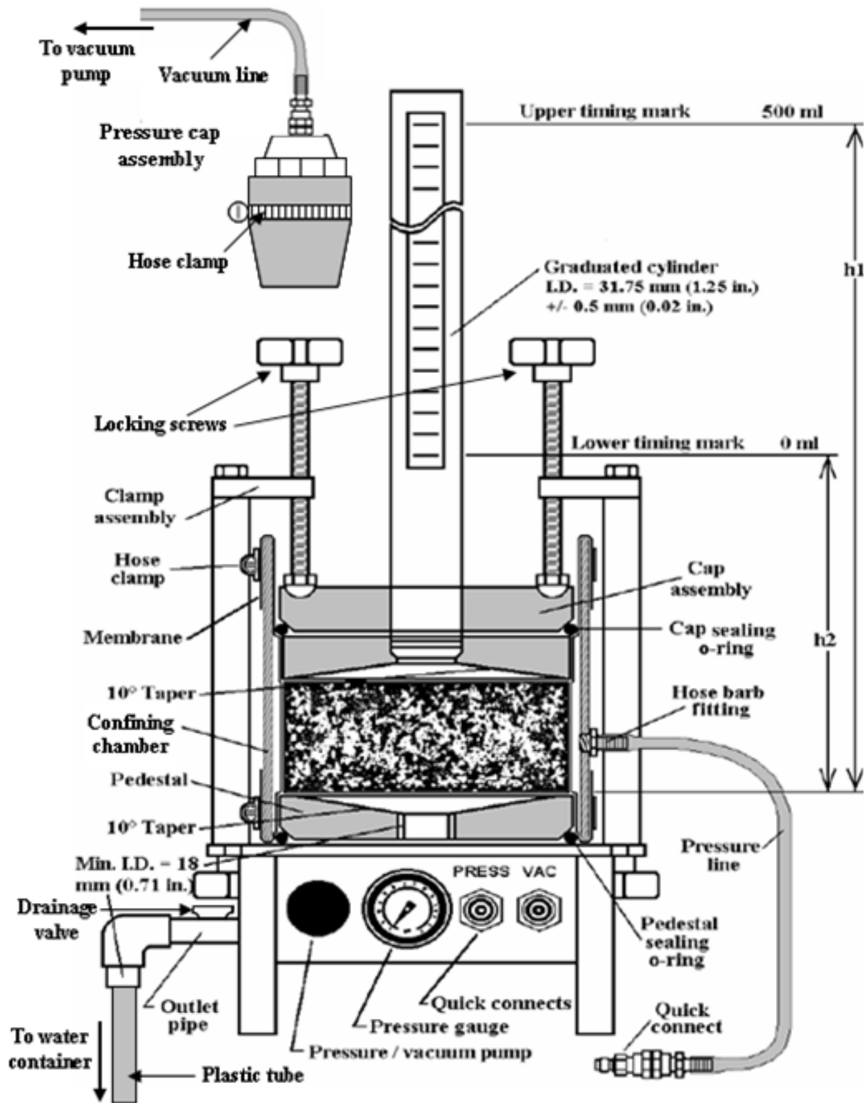
Figure C.4 – Vacuum Testing Apparatus
