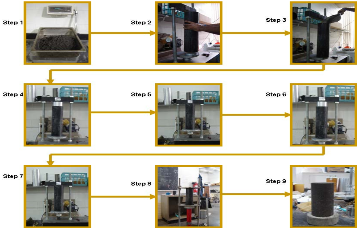
Figure 4.1 – Static Compaction Procedure
