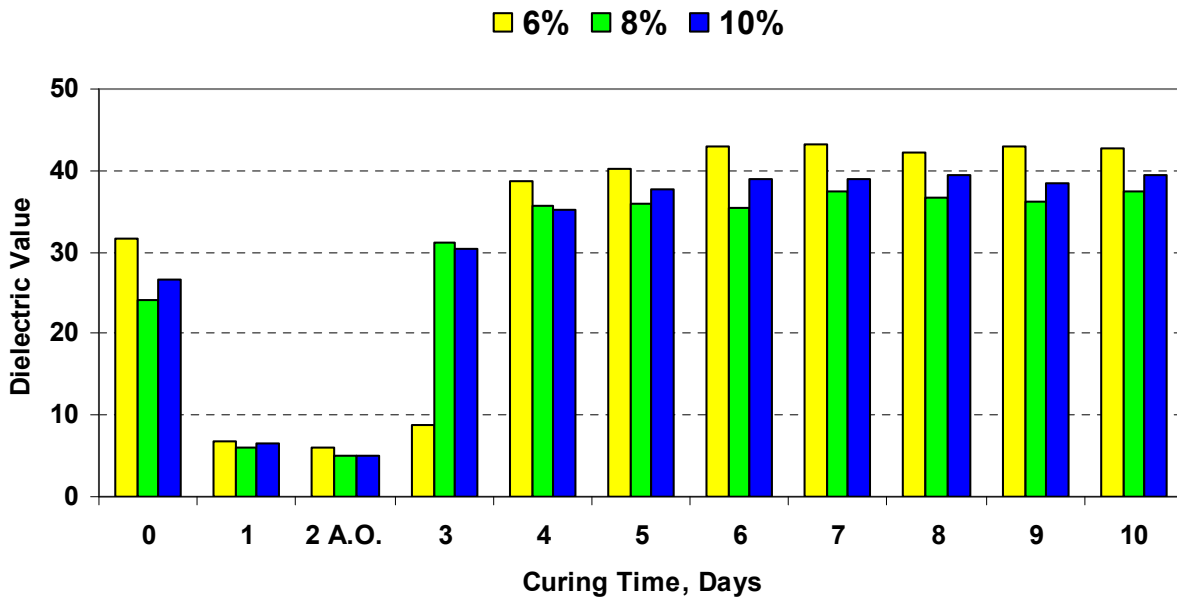
Figure 3.6 – Dielectric Results for El Paso TST Soil-Lime Specimens (A.O. = after specimen was removed from the oven)
