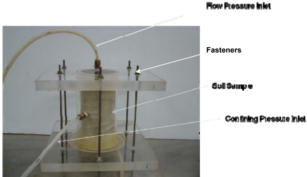
Figure 5.3 – Leachate Cell
