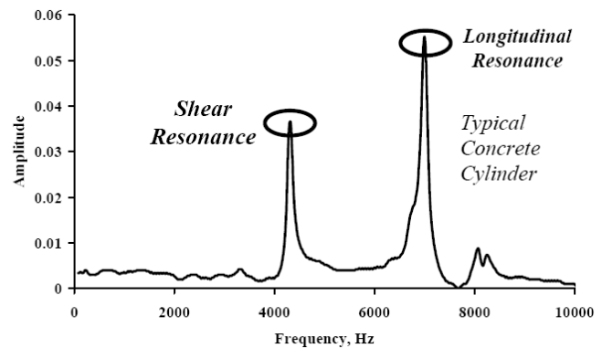
b) Typical Resonant Frequencies
