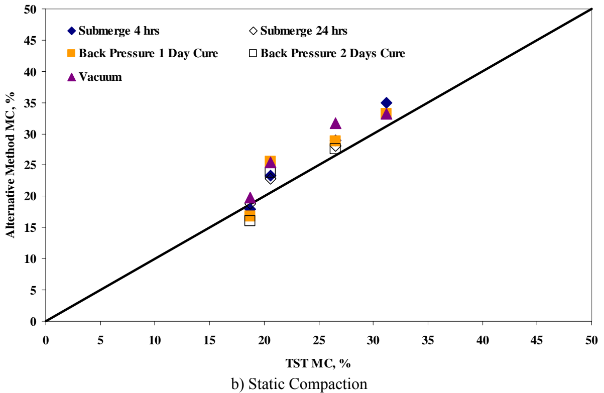
Figure 4.30 – Comparison of Moisture Contents from TST Protocol with Other Moisture Conditioning Methods
