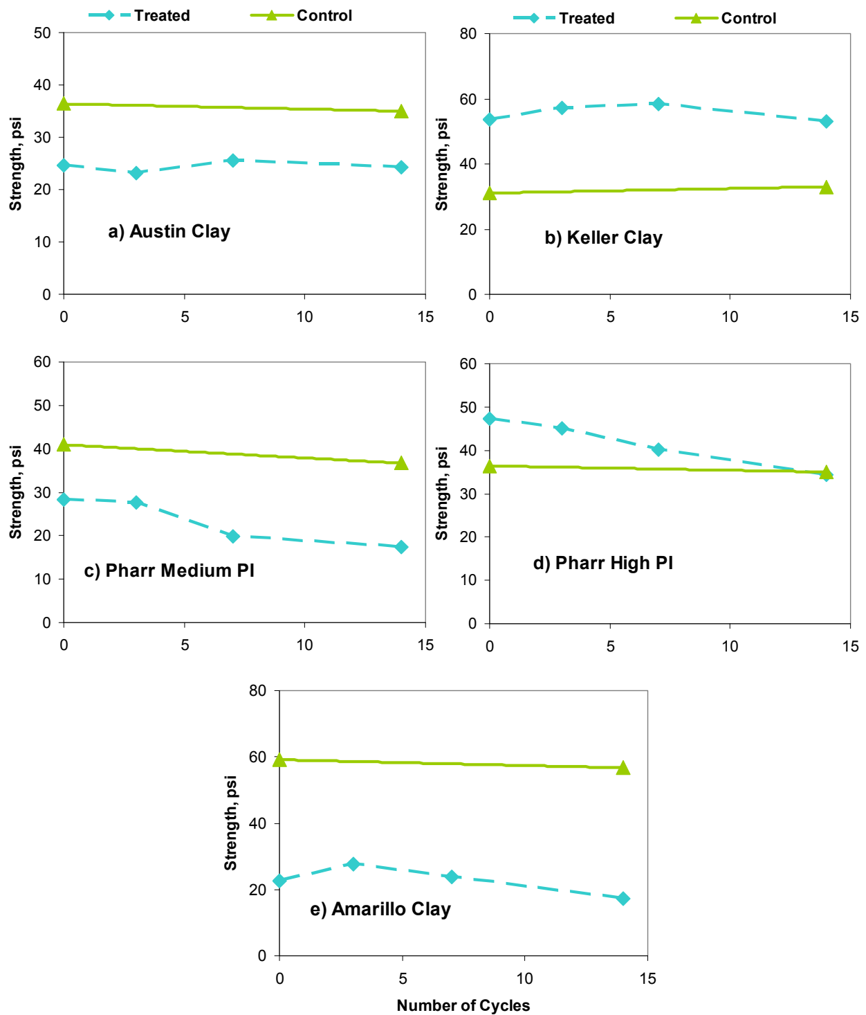
Figure 6.9 – Variation of UCS Strength with the Number of Leaching Cycles for Validation Soil Samples
