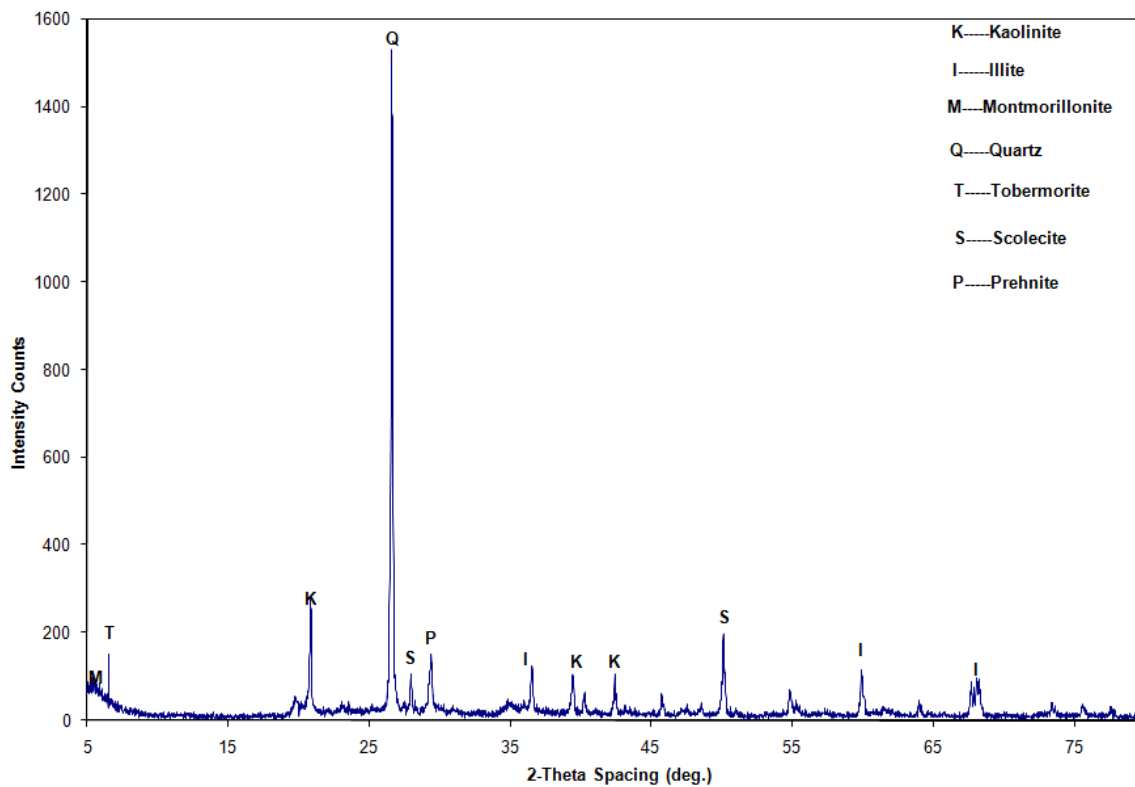
Figure B.2 – XRD Results of Bryan Soil after Treatment
