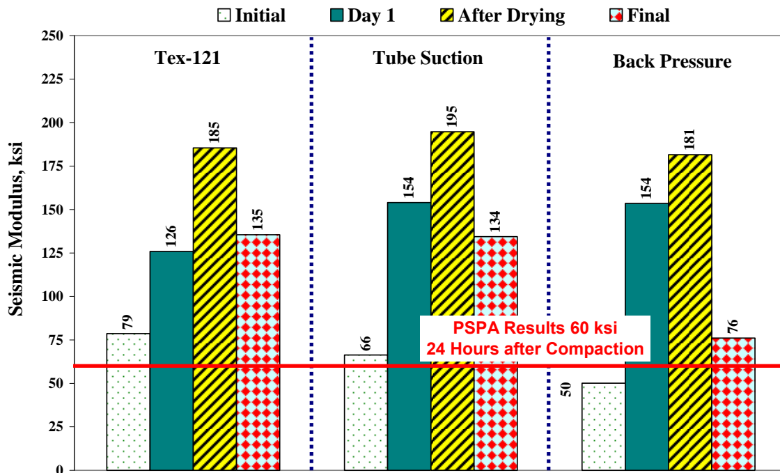
Figure 6.17 – Seismic Modulus Variation of Laboratory and Field Tests for Keller Site
