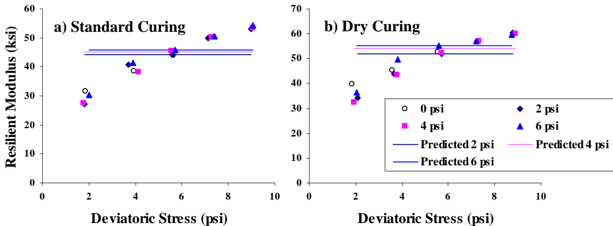
Figure 3.4 – Resilient Modulus Results for El Paso Specimens with 8% Lime
