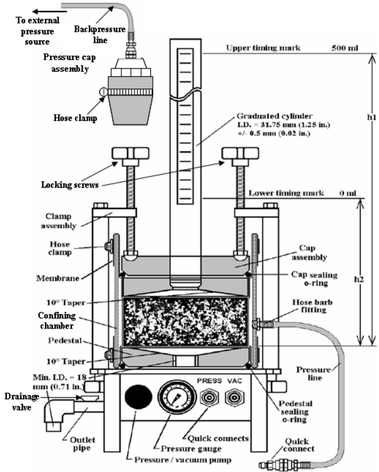
Figure C.3 – Permeability Testing Apparatus
