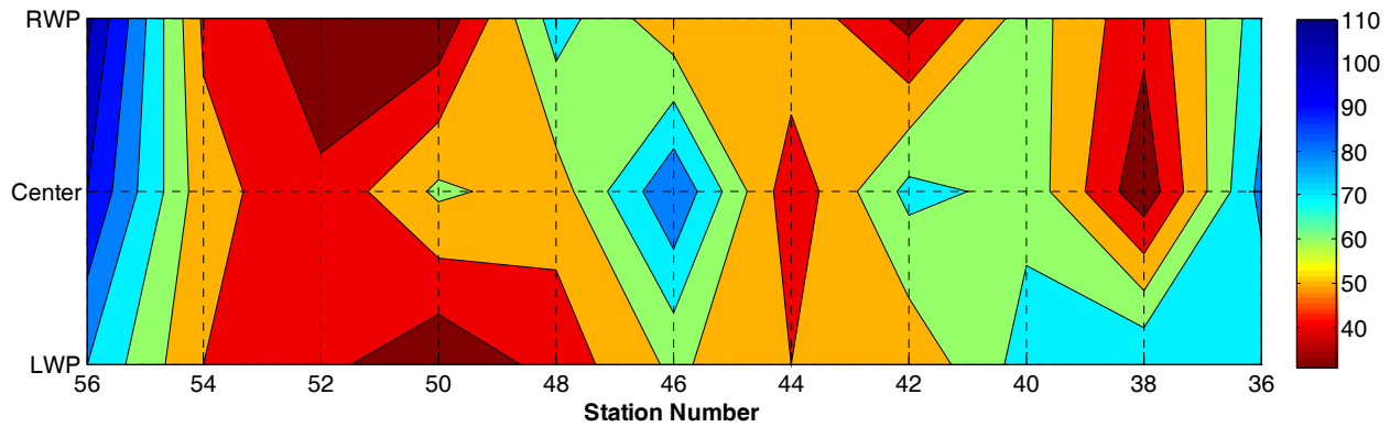
Figure D.2 – Contour Map of Field Seismic Modulus of Keller
