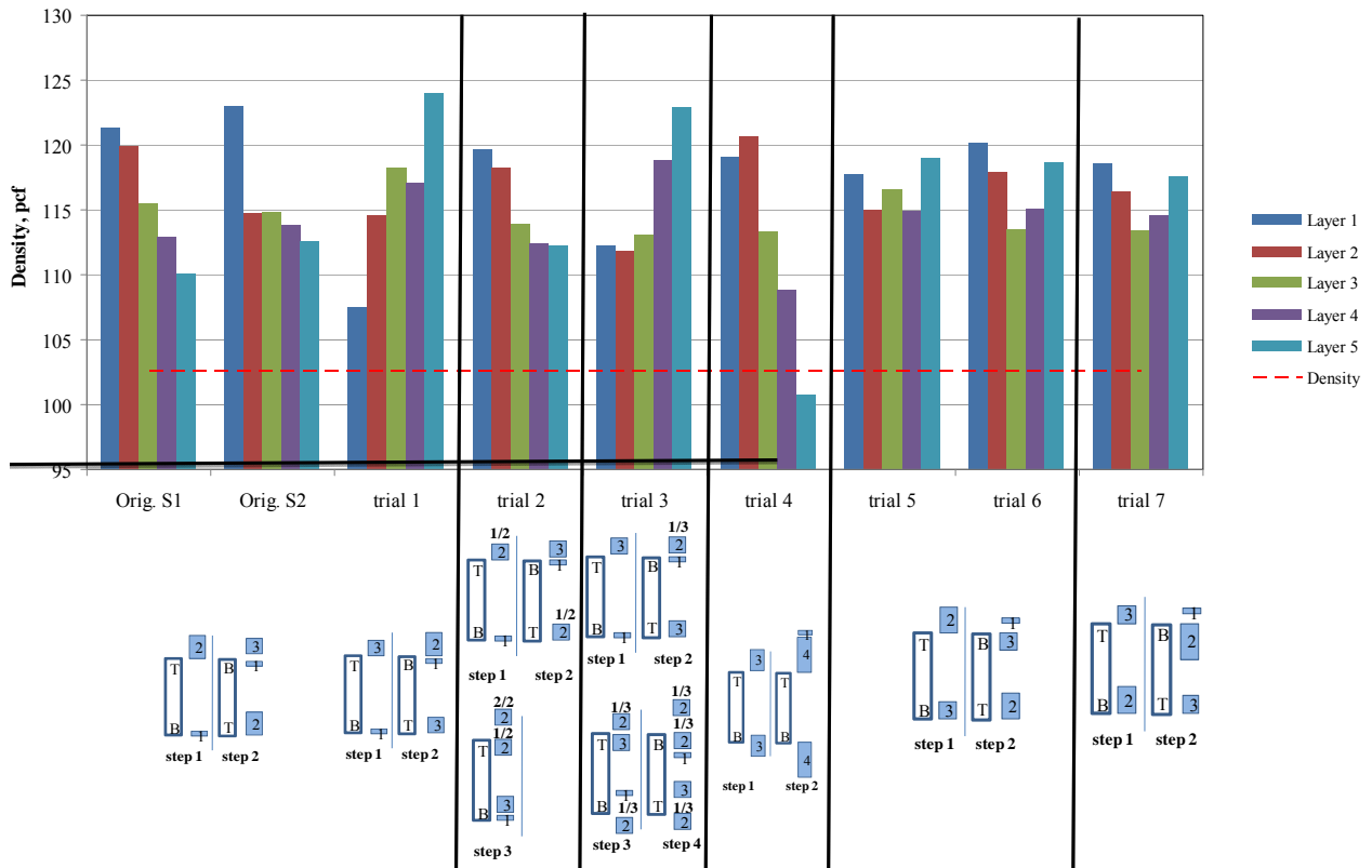
Figure 4.2 – Variation in Density Using Different Compaction Sequences
