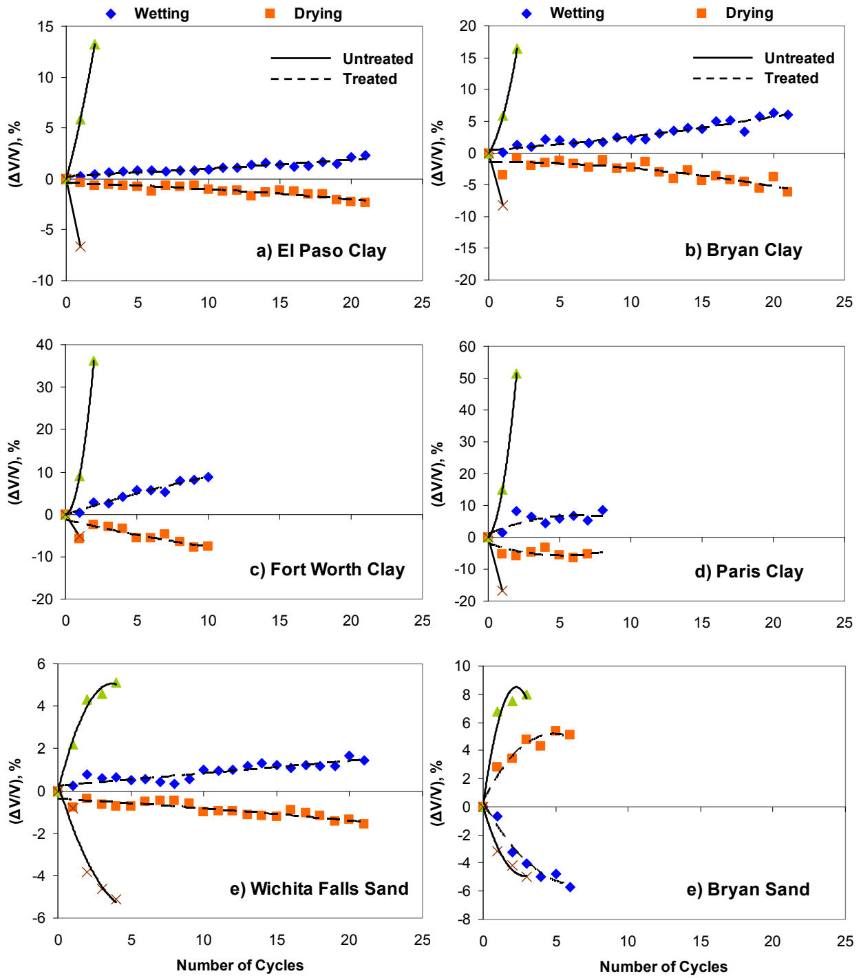
Figure 5.14 – Volumetric Changes in Different Soil Samples with Wetting/Drying Cycles
