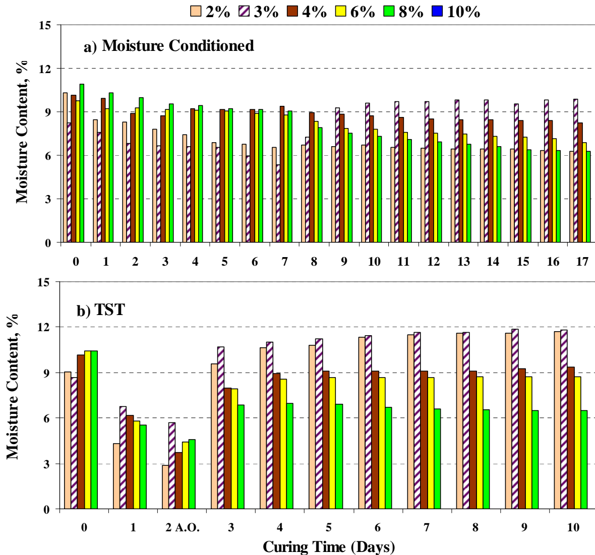
Figure 3.11 – Variation in Moisture Content for Wichita Falls Sand Specimens
