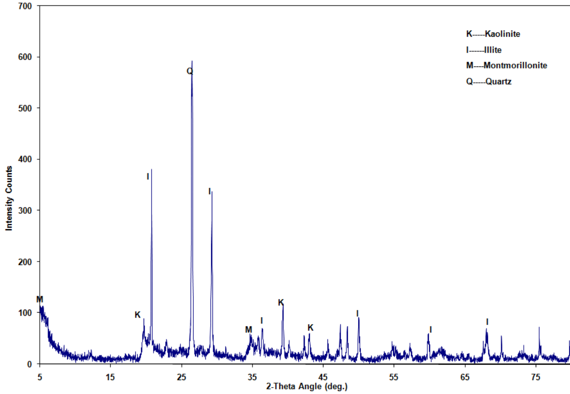
Figure B.3 – XRD Results of Fort Worth Soil before Treatment
