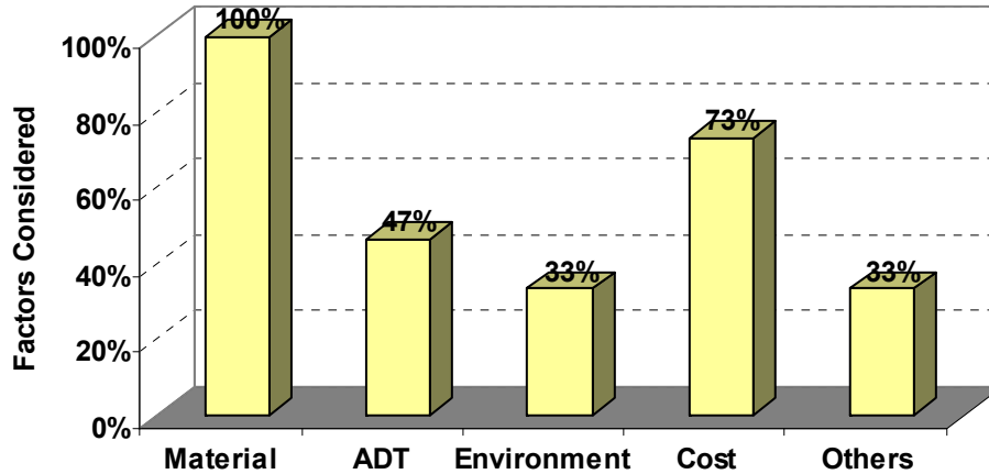
Figure A.6 – Distribution of Parameters Considered for Selection of Additives
