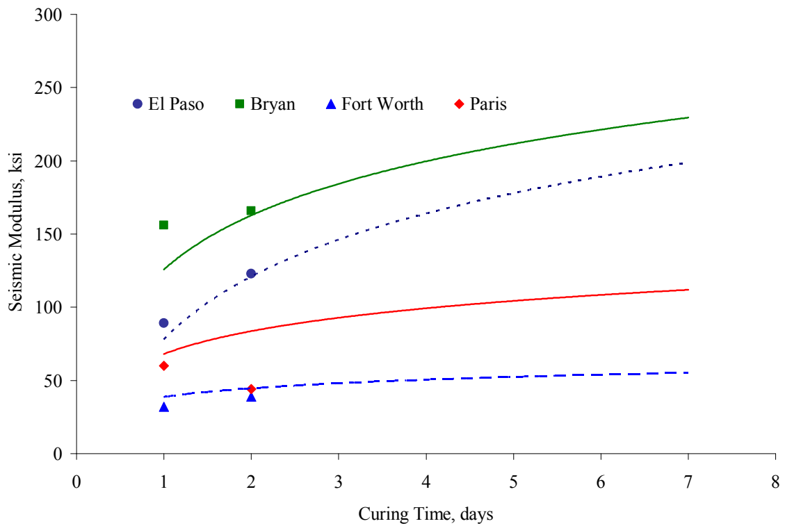
Figure 4.27 – Comparison of Curing Patterns from Tex-121-E with 2 Days at 104°F Oven
