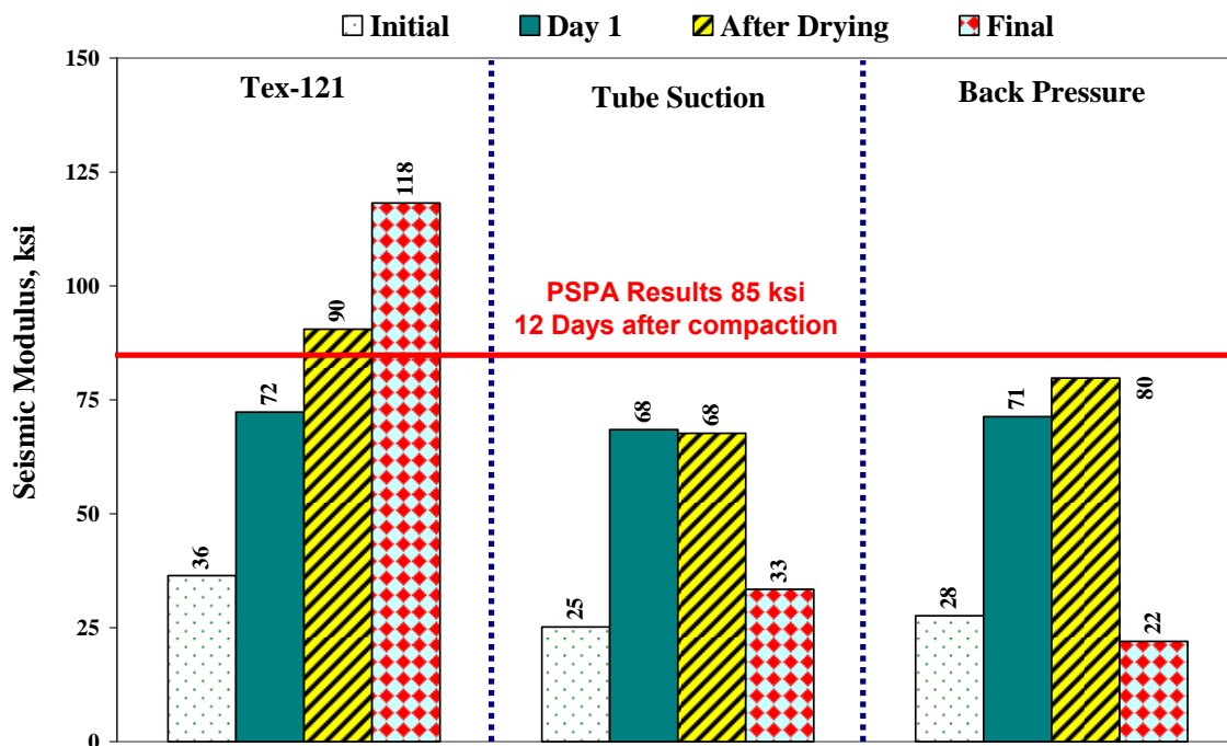
Figure 6.16 – Seismic Modulus Variation of Laboratory and Field Tests for Austin Site
