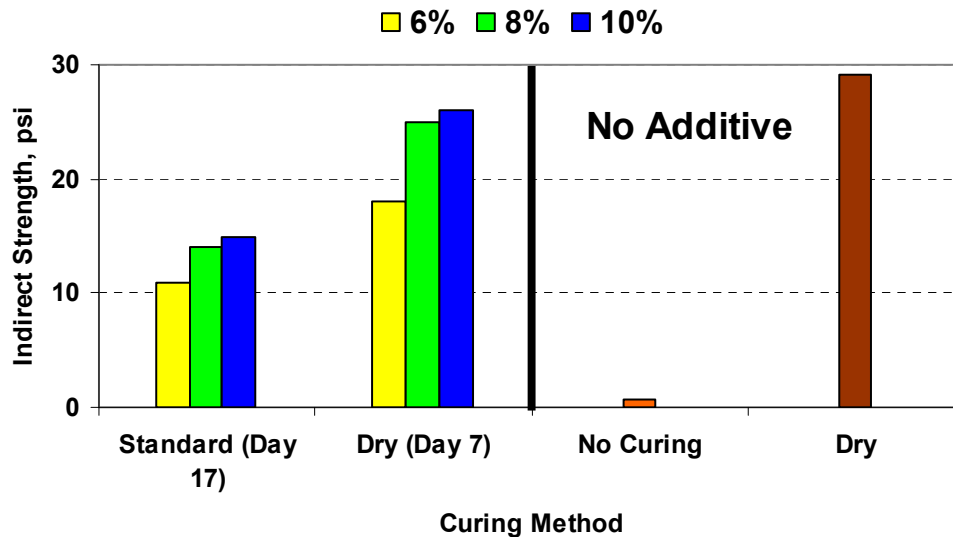
Figure 3.3 – Indirect Tensile Strength Results for El Paso Soil-Lime Specimens
