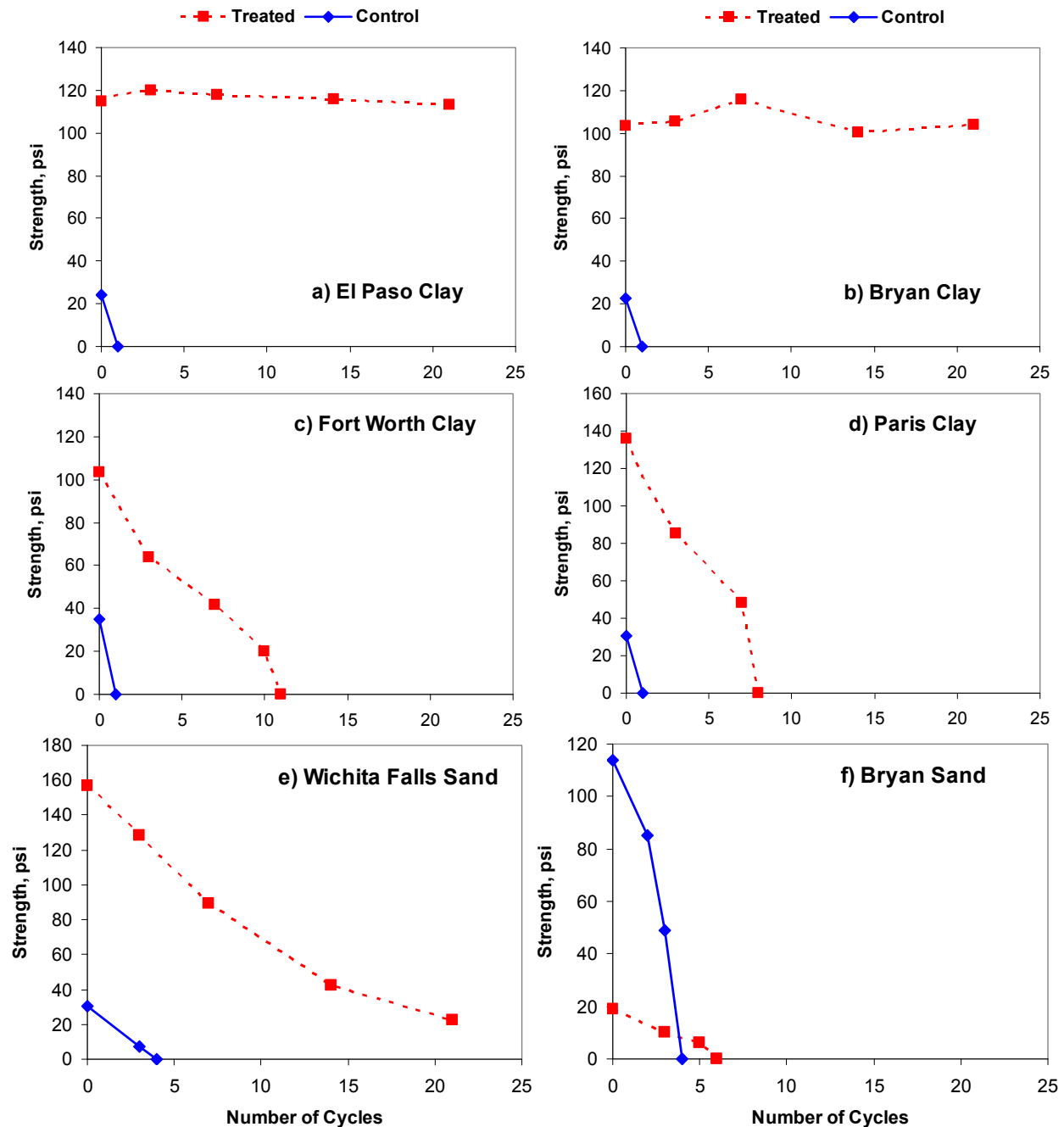
Figure 5.15 – UCS Strengths after Different Cycles of Wetting/drying for Different Soil Samples
