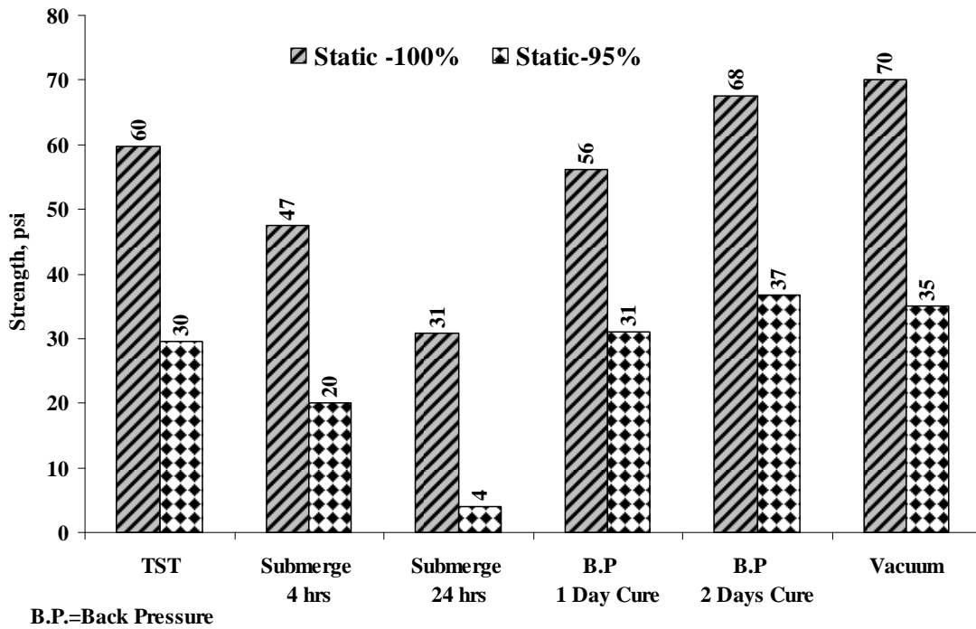
Figure 4.20 – Strength Results for Different Compactive Efforts (El Paso Material)
