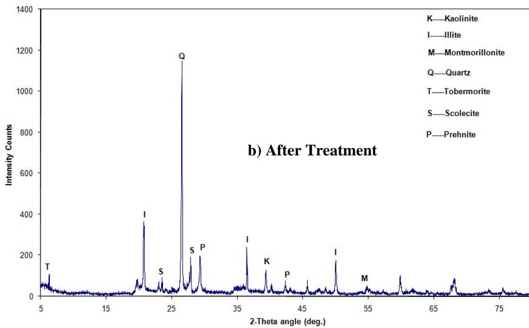
Figure 3.17 – XRD Results of Paris Soil
