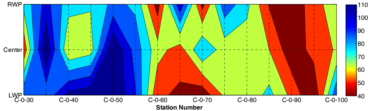
Figure D.7 – Contour Maps of Field Seismic Modulus of Medium PI Pharr Sites after 10 Days of Compaction
