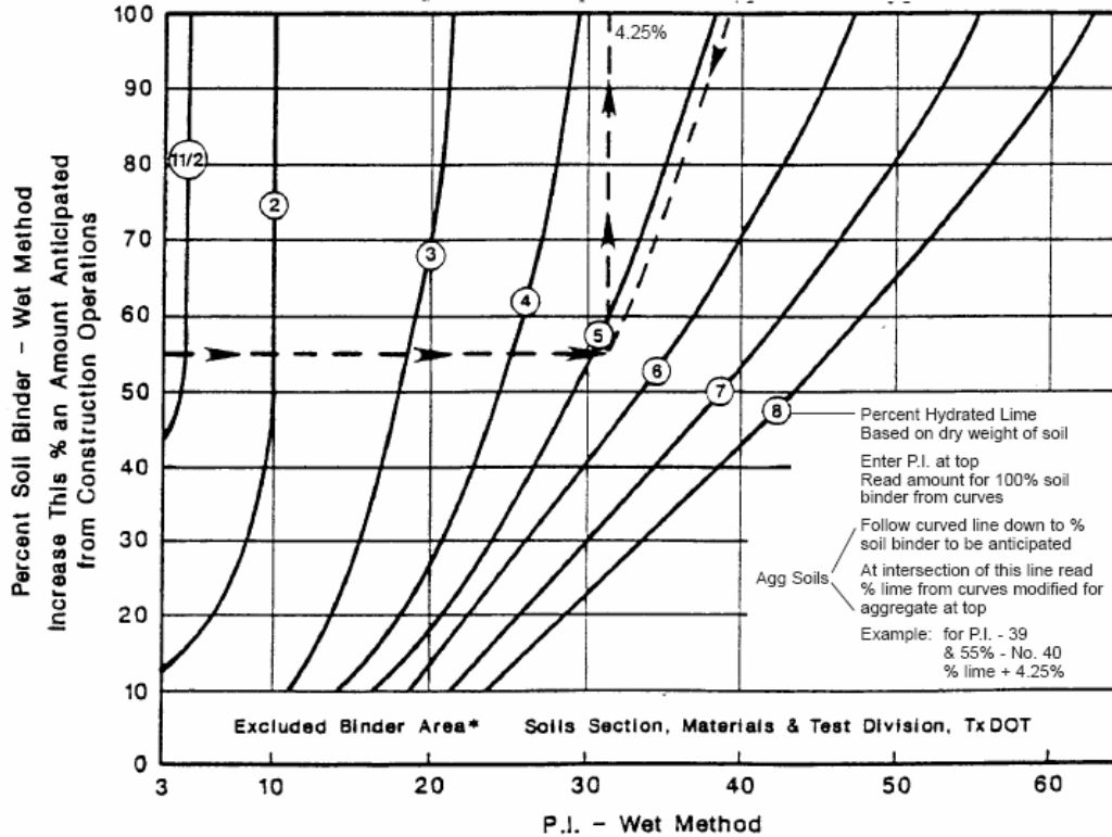
Figure 2.5 – PI Wet Method to Calculate Amount of Lime for Stabilization
