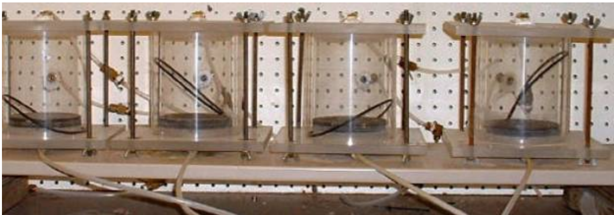
Figure 2.11 – Cyclic Wetting-Drying Setup
