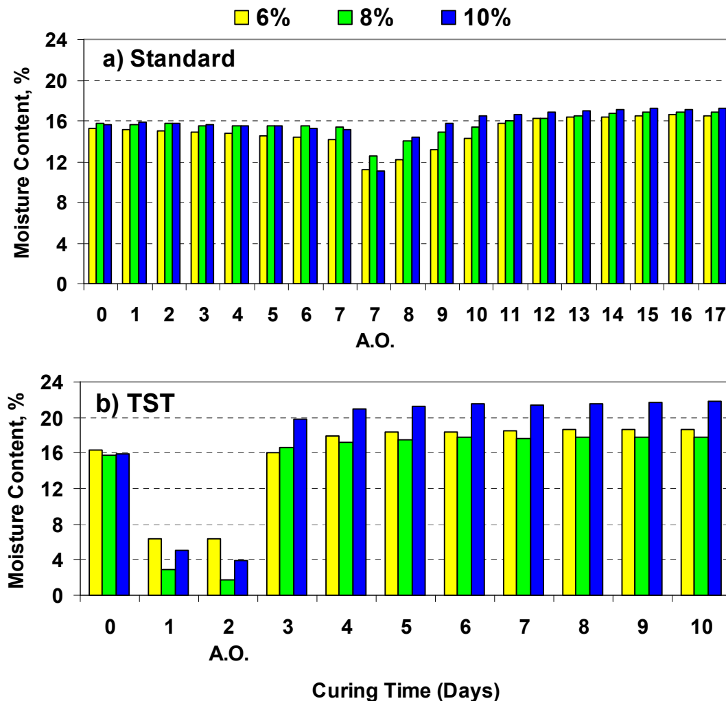
Figure 3.7 – Variations in Moisture Content for El Paso Clay Specimens (B.O. = before specimen placed in the oven, A.O. = after specimen was removed from the oven)
