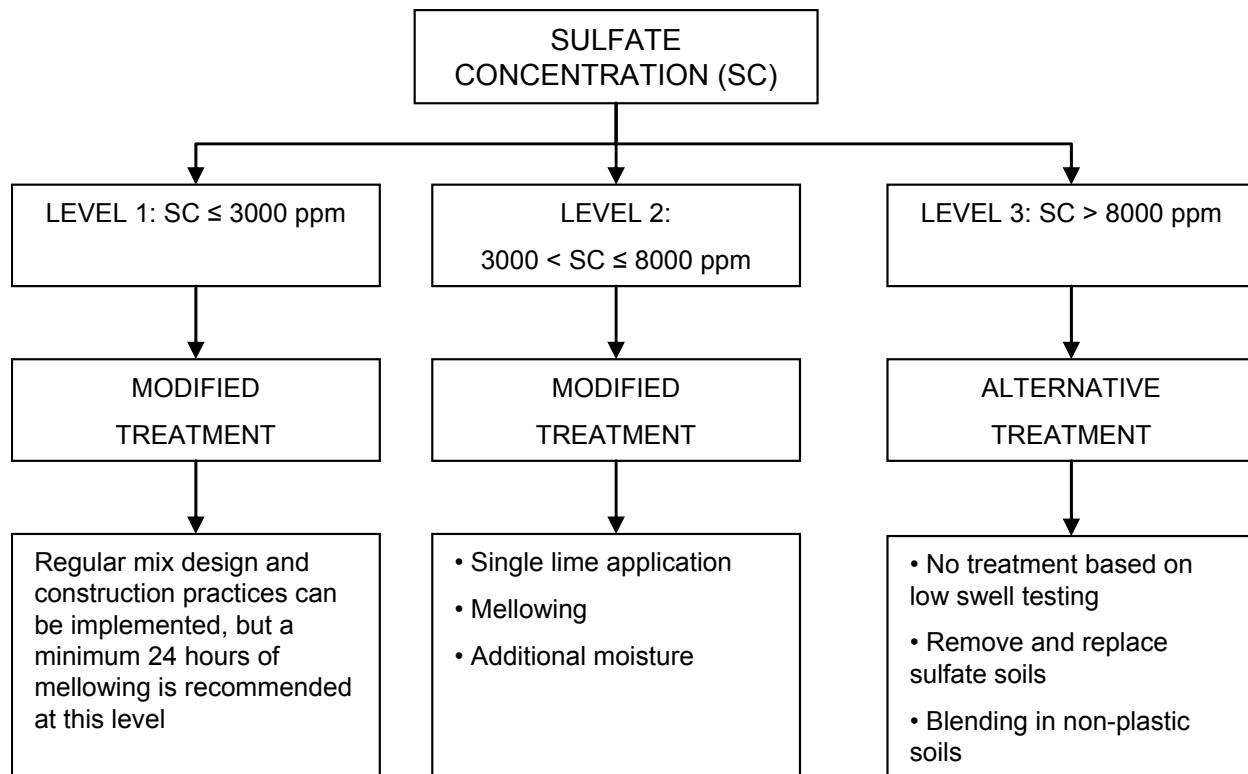
Figure 2.3 – Decision Tree to Determine Type of Treatment for Varying Sulfate Contents on Moderately to Highly Expansive Soils
