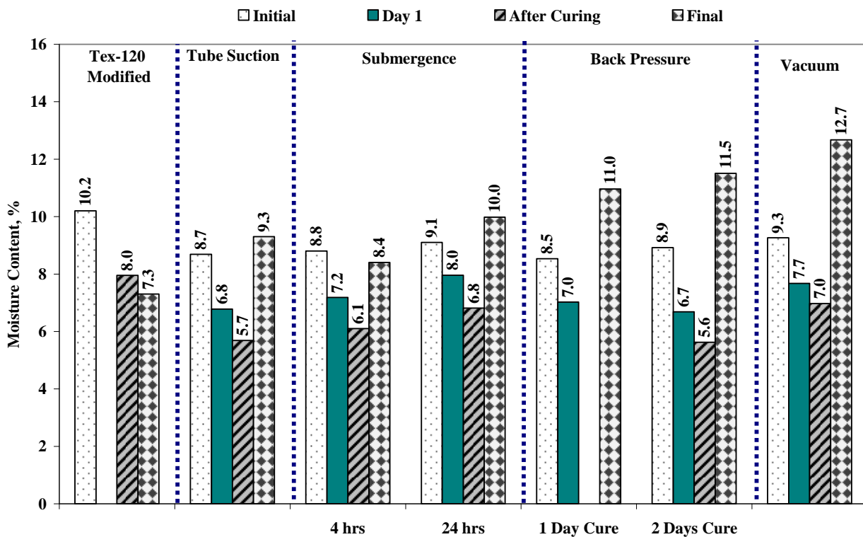
Figure 4.34 – Moisture Content Results of Moisture Conditioning Tests for Wichita Falls Material
