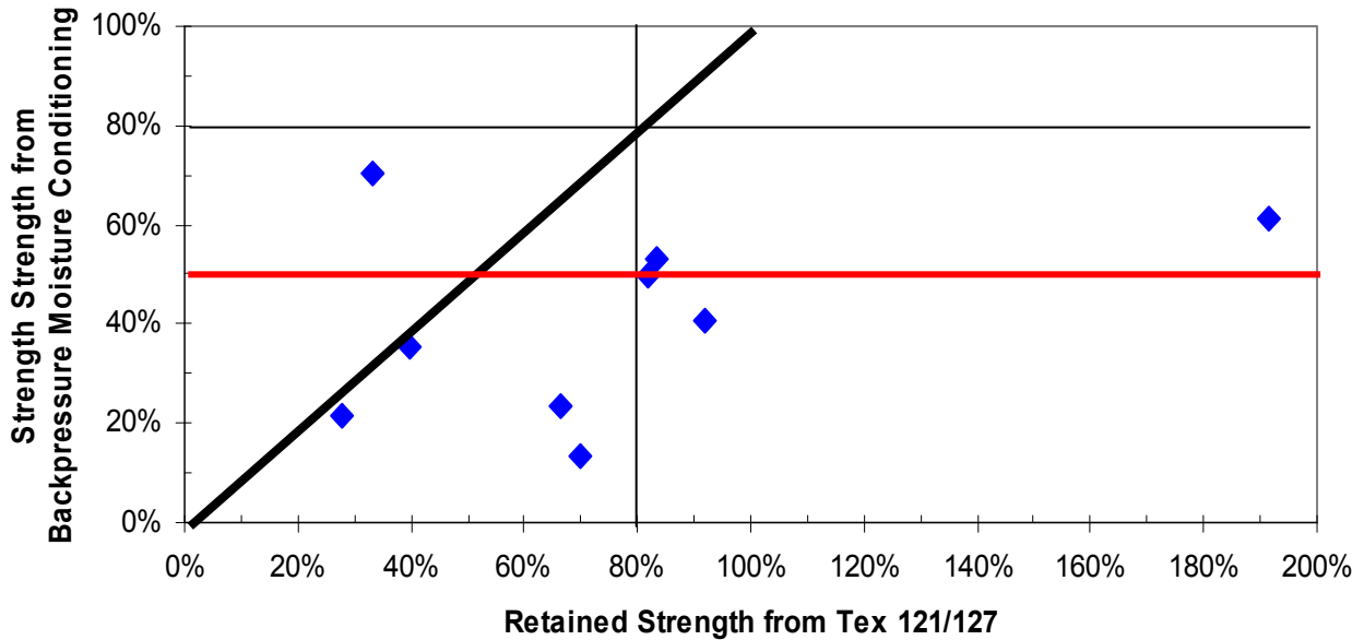
Figure 6.13 – Comparison of Retained Strengths from Current Specifications and Accelerated Methods
