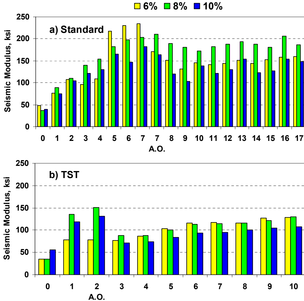
Figure 3.8 – FFRC Seismic Modulus Results for El Paso Soil-Lime Specimens
