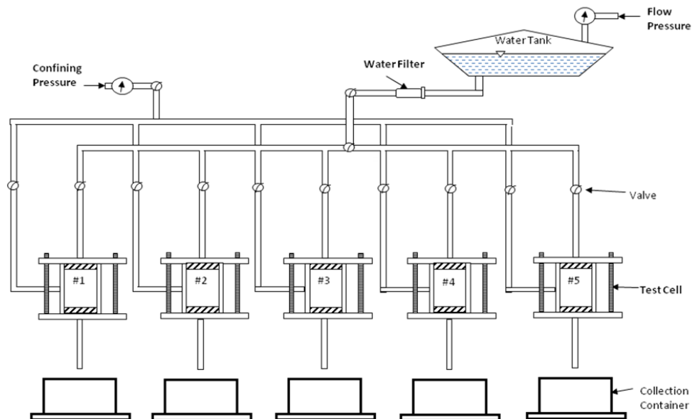
Figure 5.1 – Schematic of the Leachate Process
