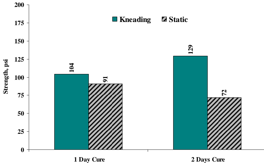
Figure 4.17 – Strengths for Different Curing Times after Moisture Conditioning
