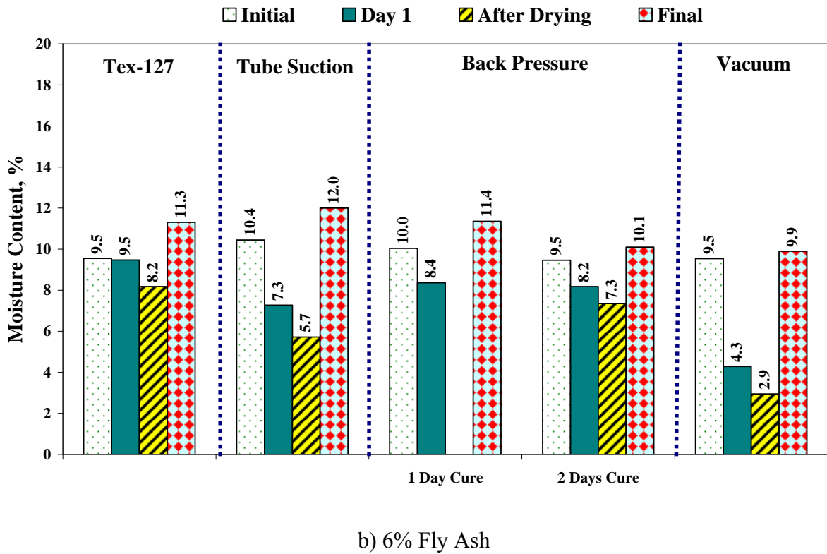
Figure 4.38 – Moisture Content Results of Moisture Conditioning Tests for Bryan Sand Material
