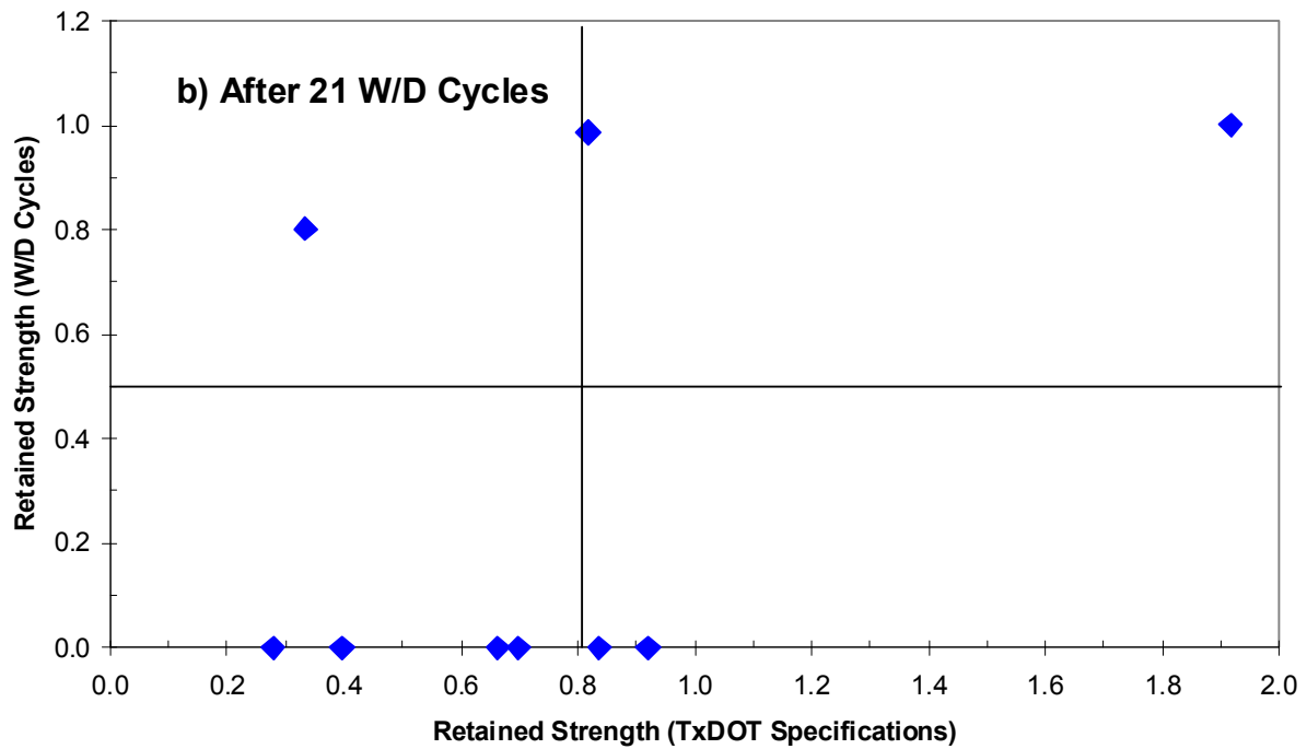
Figure 6.14 – Comparison of Retained Strengths of TxDOT Specifications with Wetting/Drying Cycles
