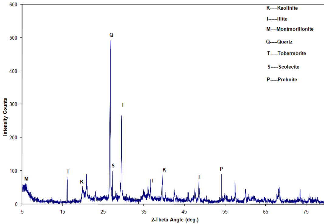
Figure B.4 – XRD Results of Fort Worth Soil after Treatment
