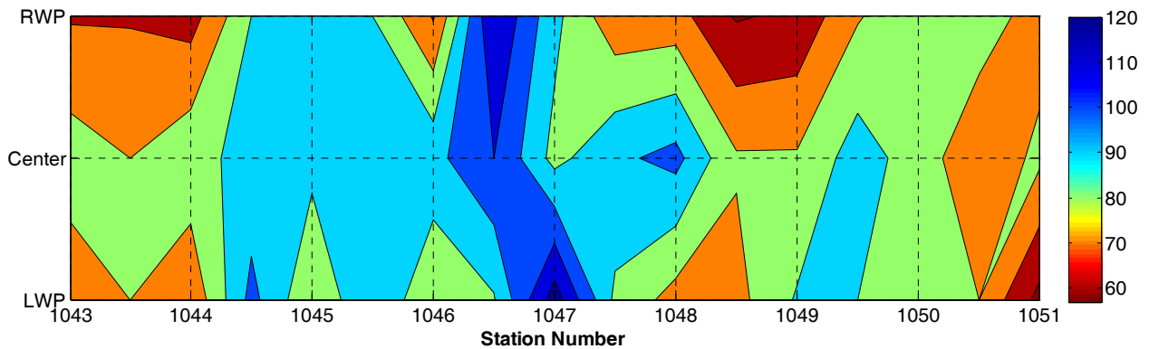
Figure D.1 – Contour Map of Field Seismic Modulus of Austin Site
