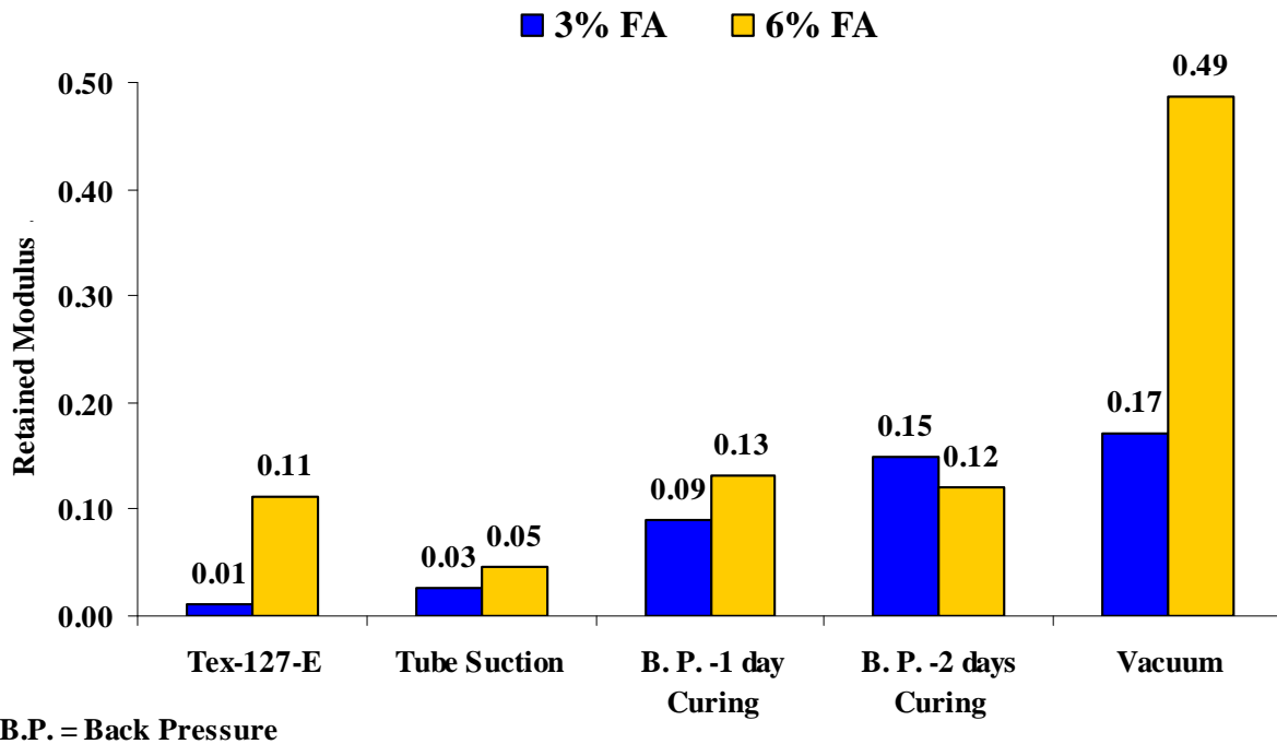
Figure 4.40 – Seismic Moduli Ratios between Specimens after Moisture Conditioning and after Curing Period
