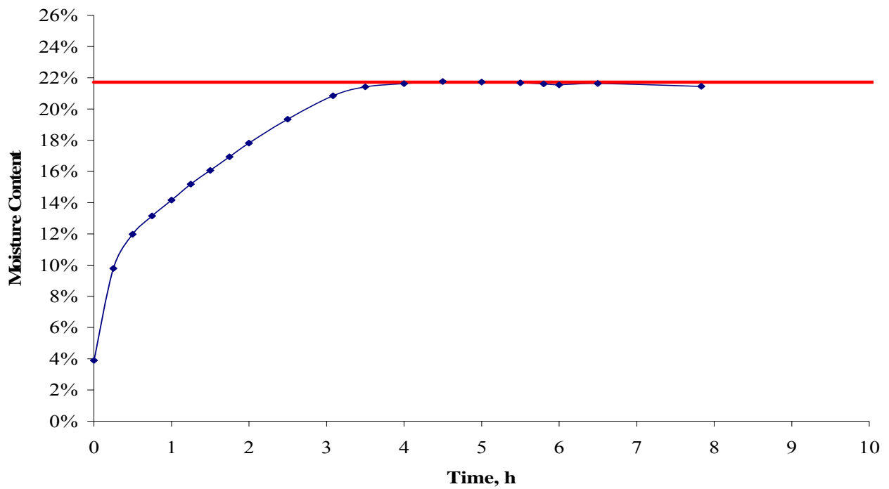
Figure 4.6 – Variation in Moisture Content with Time for Back Pressure Moisture Conditioning
