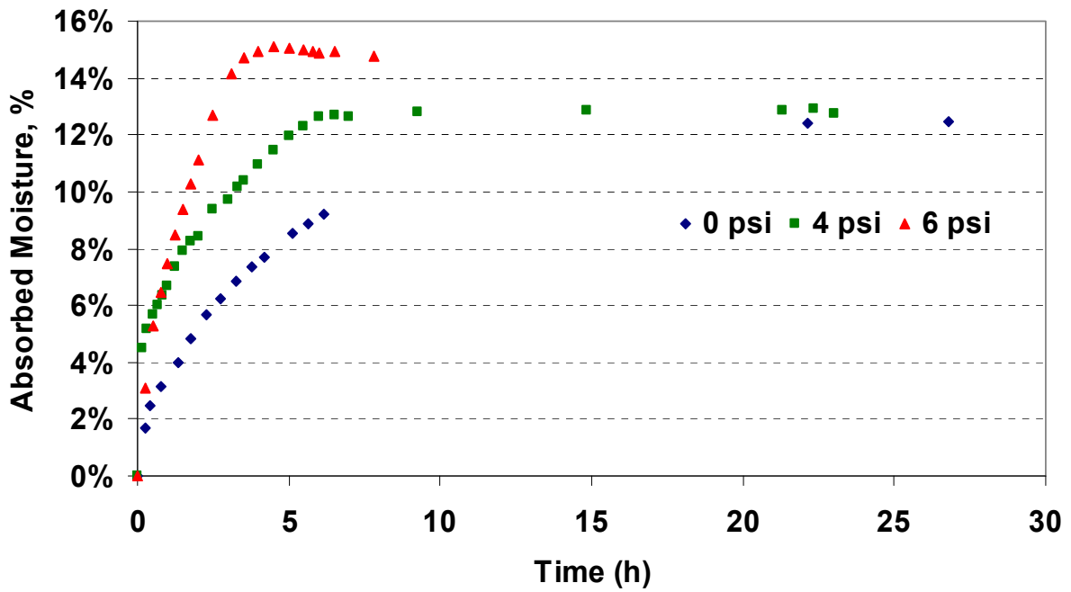
Figure 4.10 – Variations in Moisture Content with Time for Different Back Pressures
