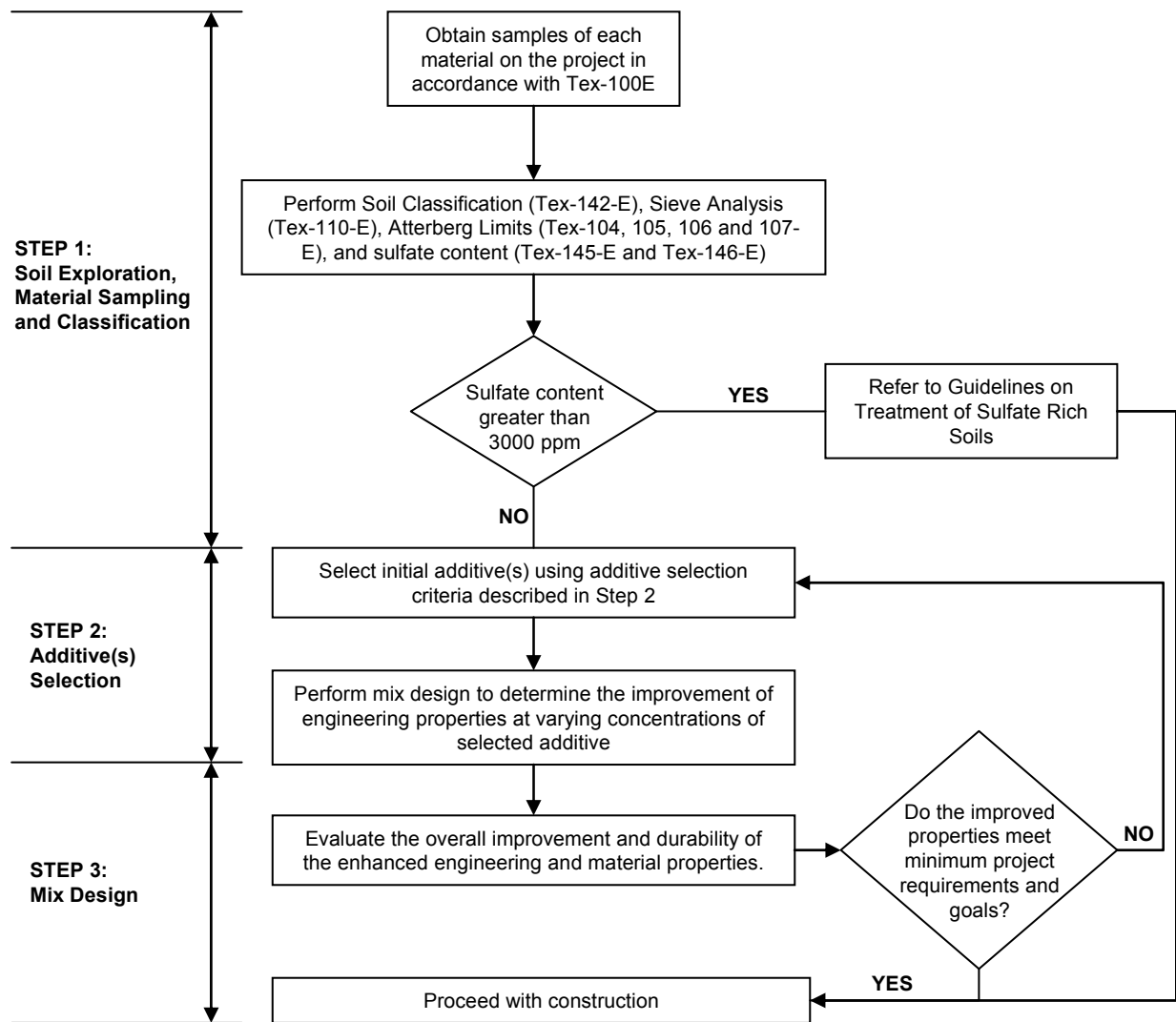
Figure 2.2 – Flowchart for Subgrade Soil Treatment (from TxDOT Guidelines)
