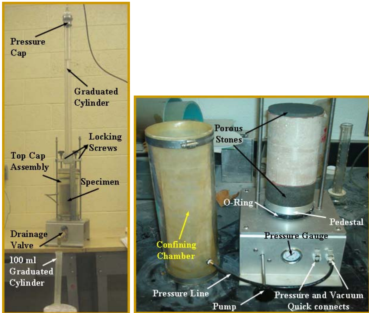
Figure 4.3 – Back Pressure Test Apparatus
