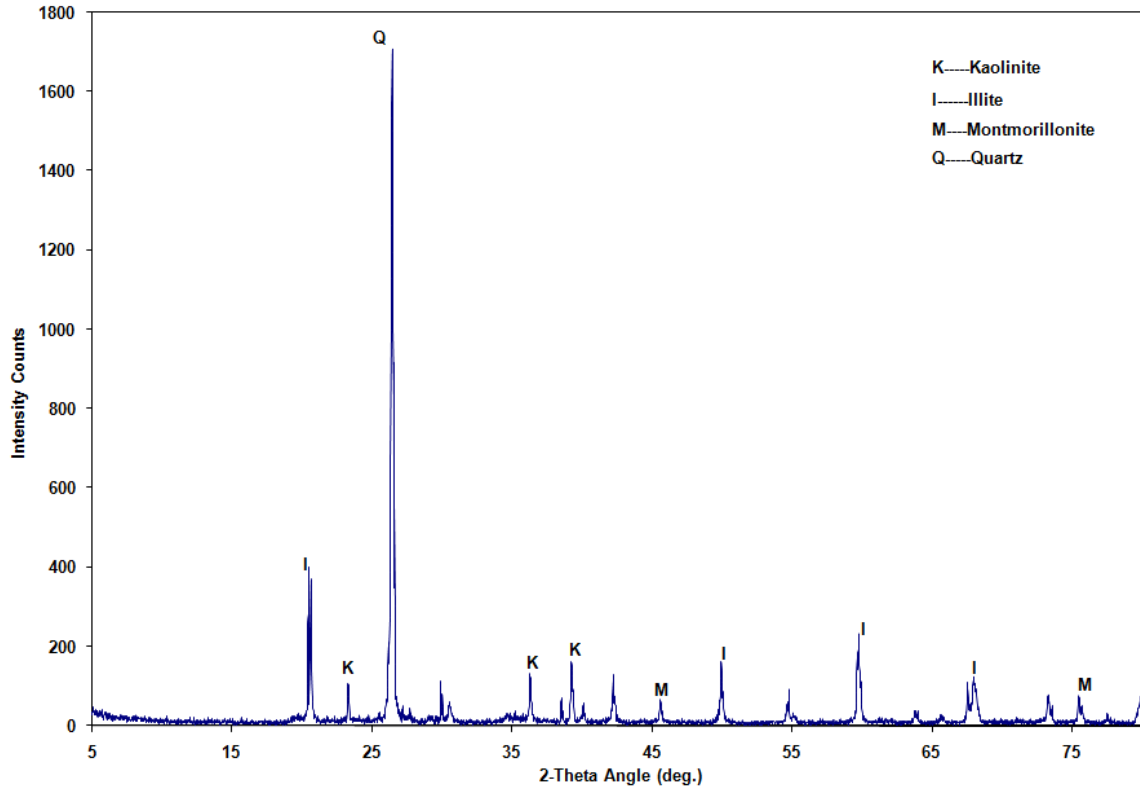
Figure B.5 – XRD Results of Wichita Falls Soil before Treatment
