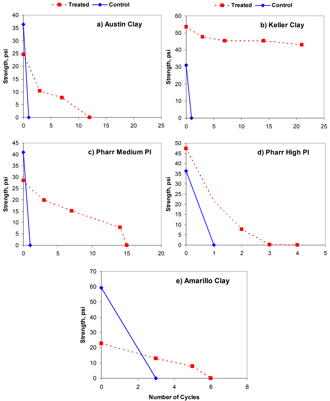
Figure 6.11 – Variation of UCS Strength with the Number of W/D cycles for Validation Soil Samples
