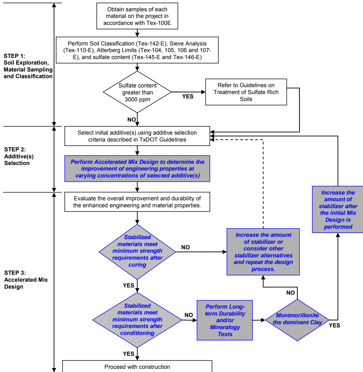
Figure 7.1 – Proposed Flowchart for Subgrade Soil Treatment
