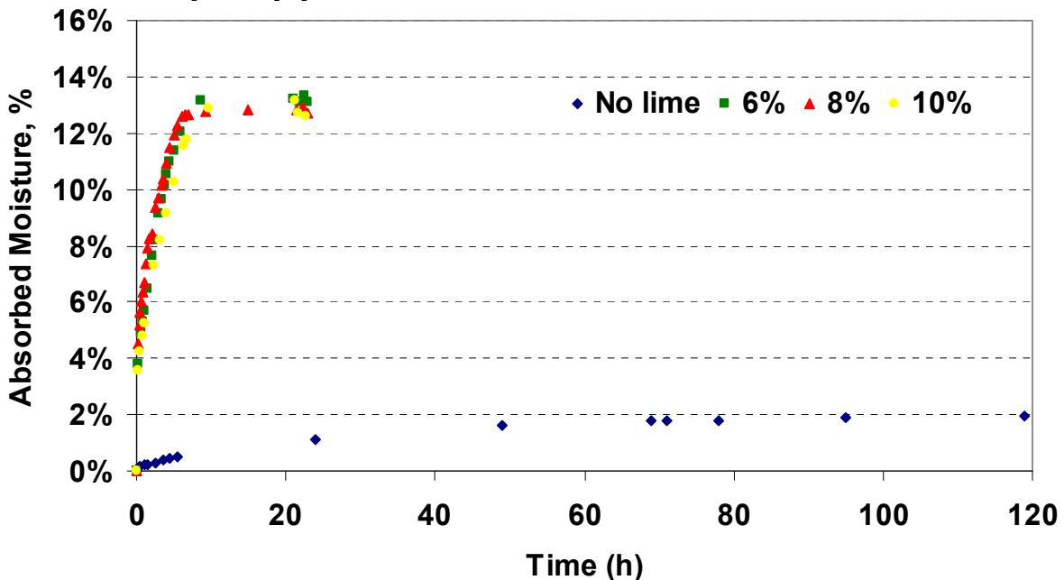
Figure 4.11 – Variations in Moisture Content with Time for Different Additive Contents
