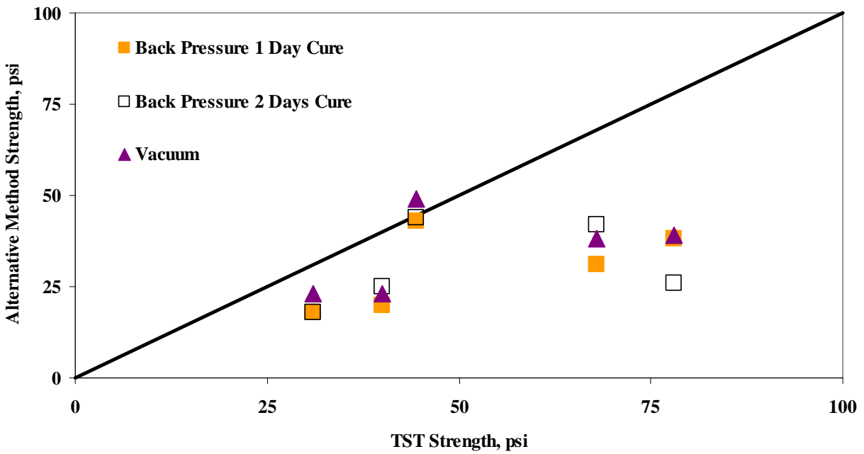
Figure 6.5 – Comparison of Strengths from Different Moisture Conditioning Methods
