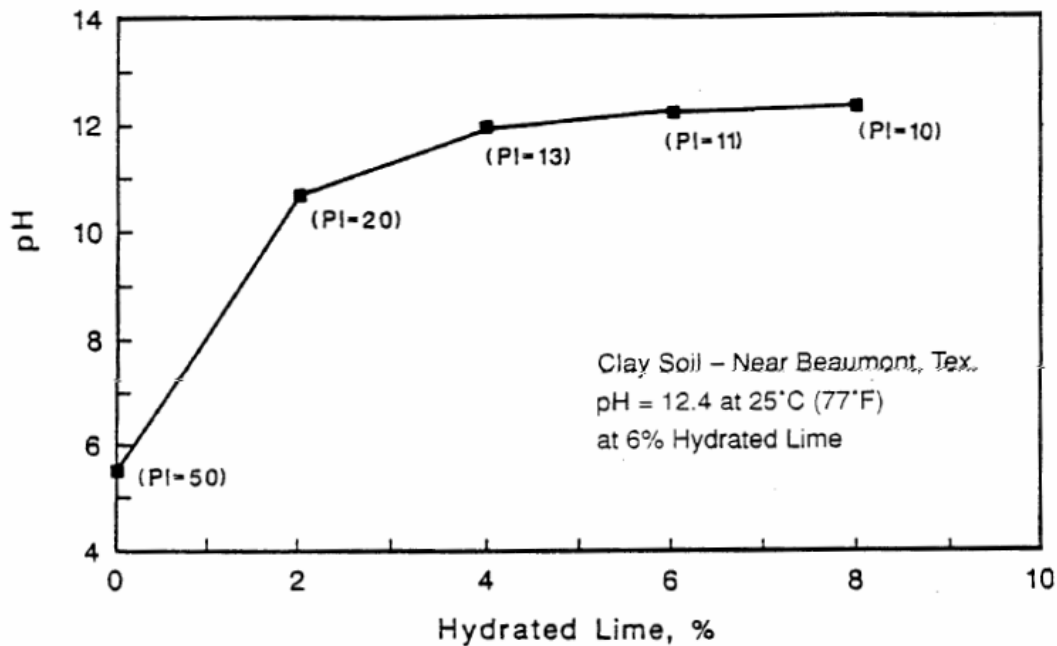
Figure 2.7 – Example of Eades and Grim Test for Different Lime Contents (Little, 1995)
