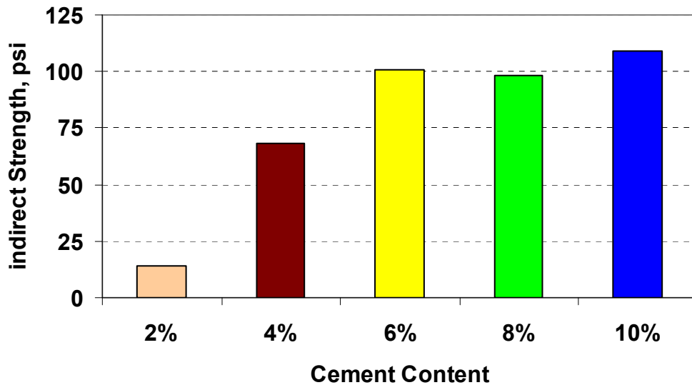
Figure 3.10 – Indirect Tensile Strengths for Wichita Falls Sand with Standard Curing
