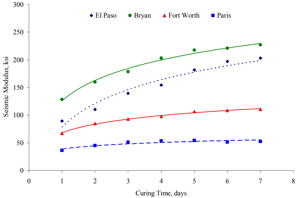
Figure 4.26 – Variation in Moduli with Curing Time for Four Lime-Stabilized Clays
