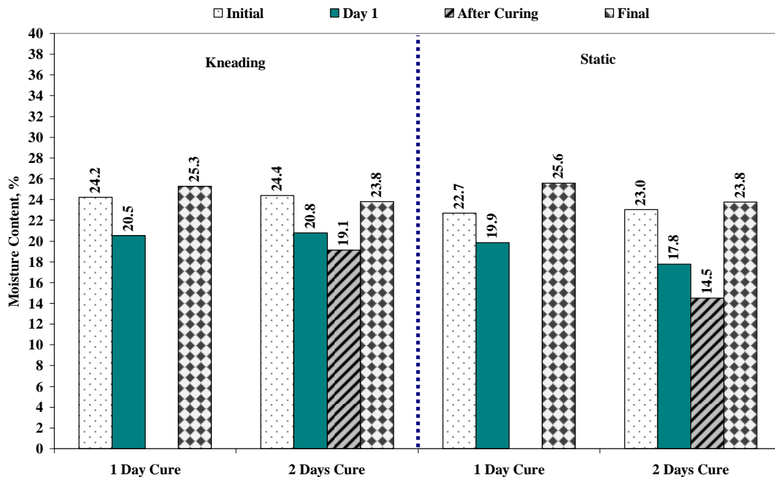
Figure 4.18 – Moisture Contents for 1 Day and 2 Day Cured Specimens
