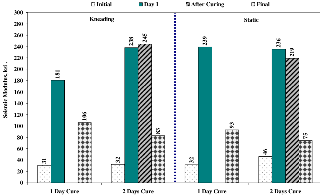
Figure 4.19 – Seismic Moduli for 1 Day and 2 Day Cured Specimens
