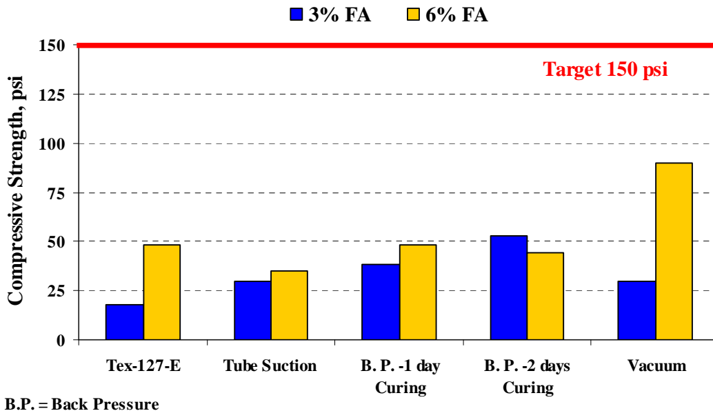
Figure 4.37 – Strength Results of Moisture Conditioning Tests for Bryan Sand Material
