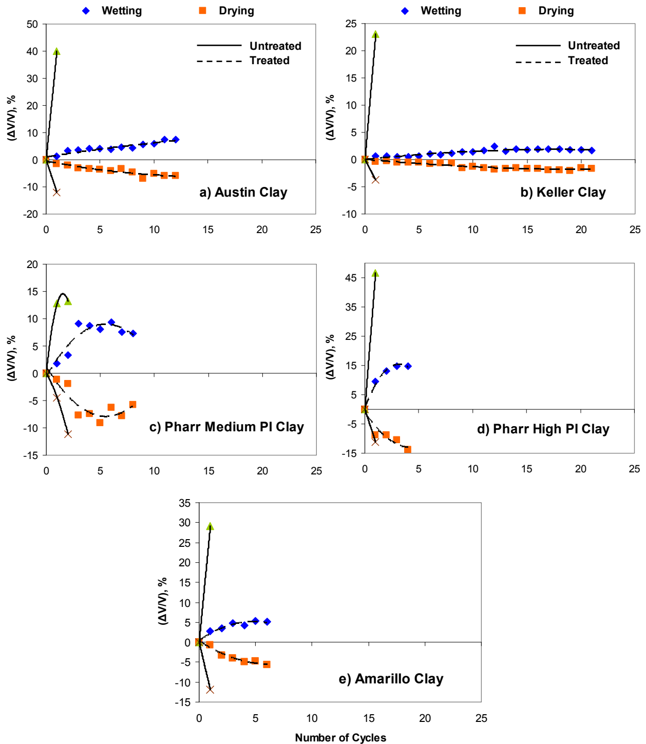
Figure 6.10 – Variation of Volumetric Strains with the Number of W/D Cycles for Validation Soil Samples
