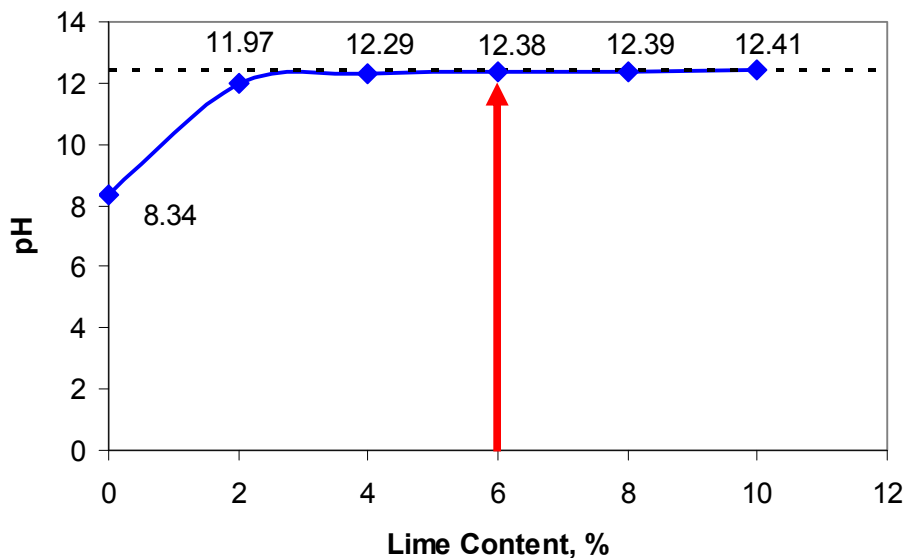
Figure 3.1 – Variation in pH with Lime Content for El Paso Clay
