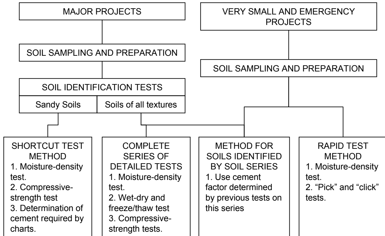
Figure 2.6 – Flowchart for Soil-Cement Laboratory Tests (after PCA, 1995)
