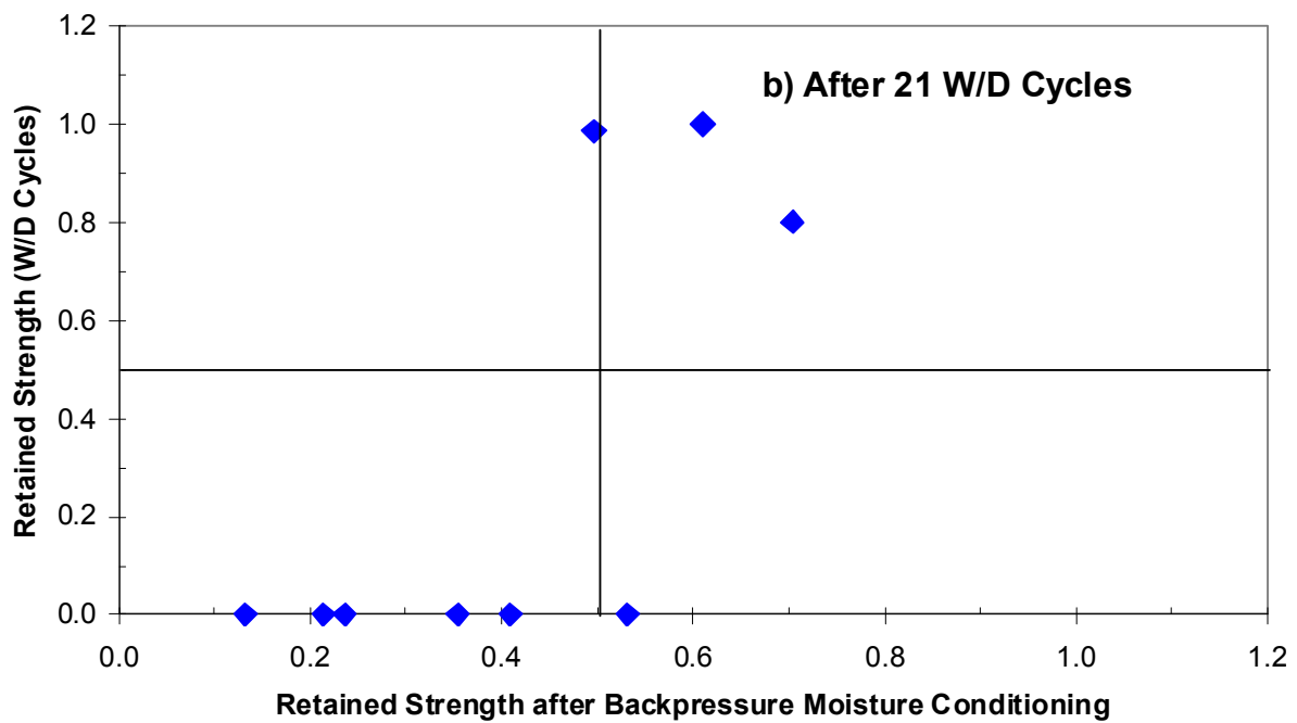
Figure 6.15 – Comparison of Retained Strengths of Accelerated Moisture Conditioning with Wetting/Drying Cycles
