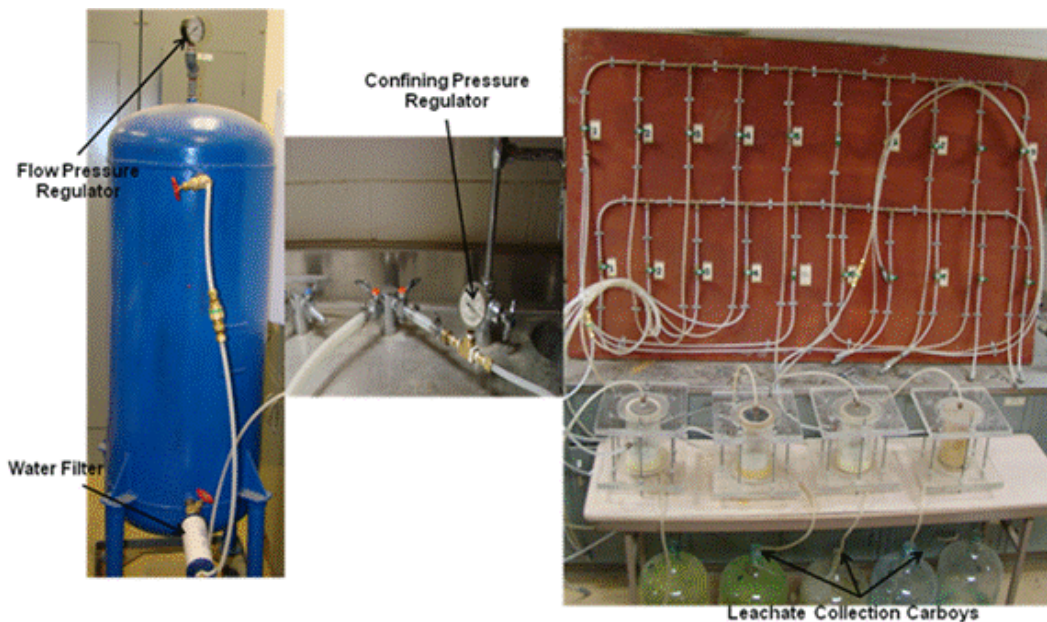
Figure 5.4 – Apparatus Used to Conduct Leachate Studies
