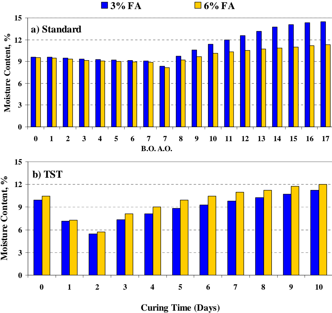
Figure 3.13 – Variation in Moisture Content for Bryan Sand-Fly Ash Specimens (B.O. = before specimen placed in the oven, A.O. = after specimen was removed from the oven)
