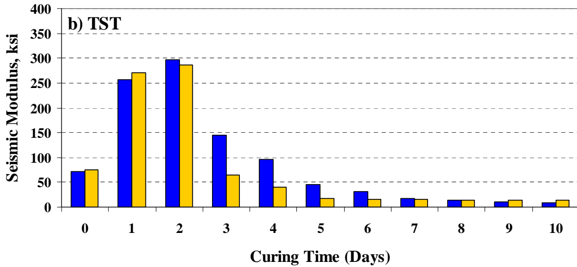
Figure 3.14 – FFRC Seismic Modulus Results for Bryan Sand-Fly Ash Specimens (B.O. = before specimen placed in the oven, A.O. = after specimen was removed from the oven)
