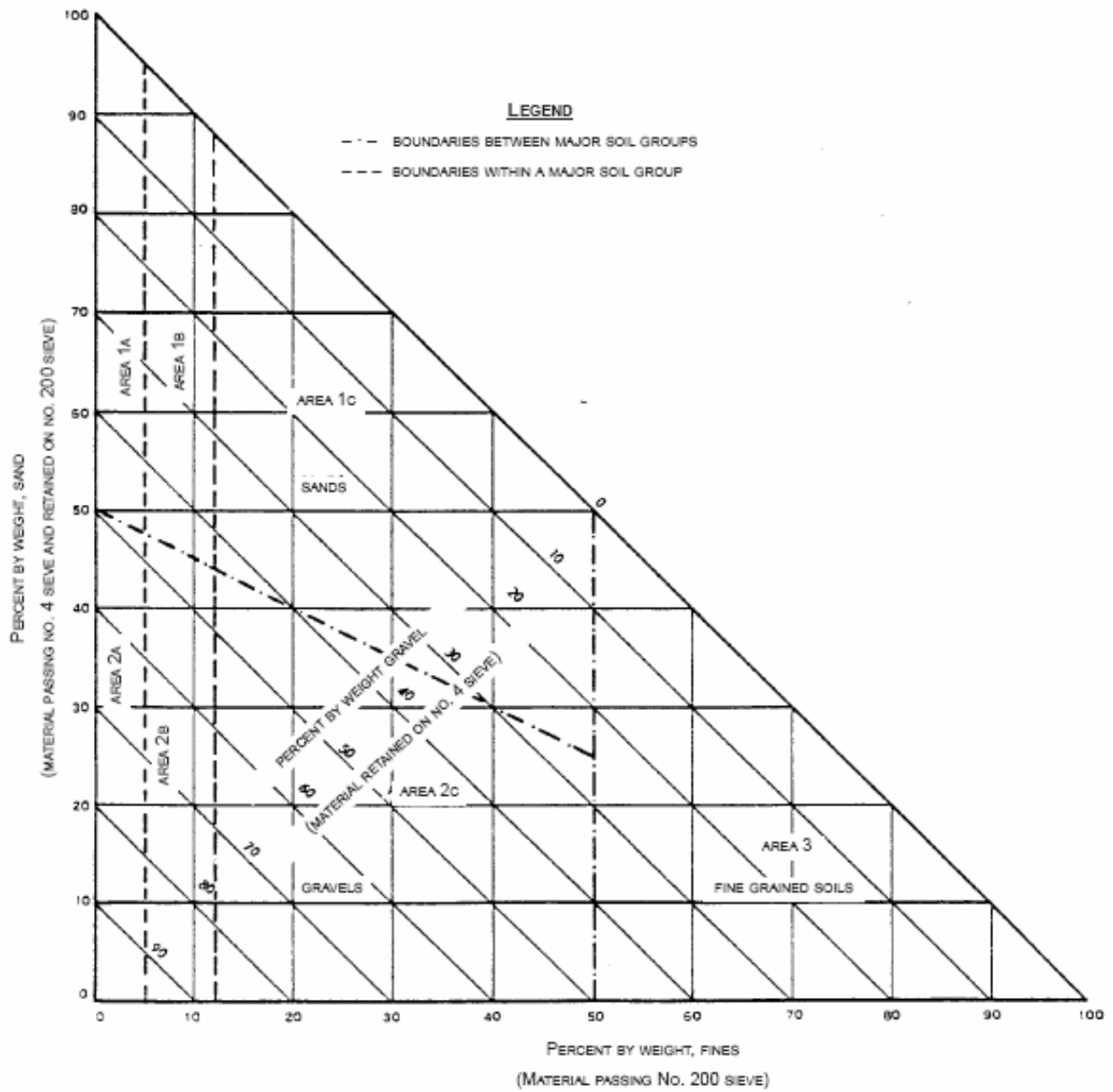
Figure 2.4 – Gradation Triangle to Select a Commercial Stabilizing Agent
