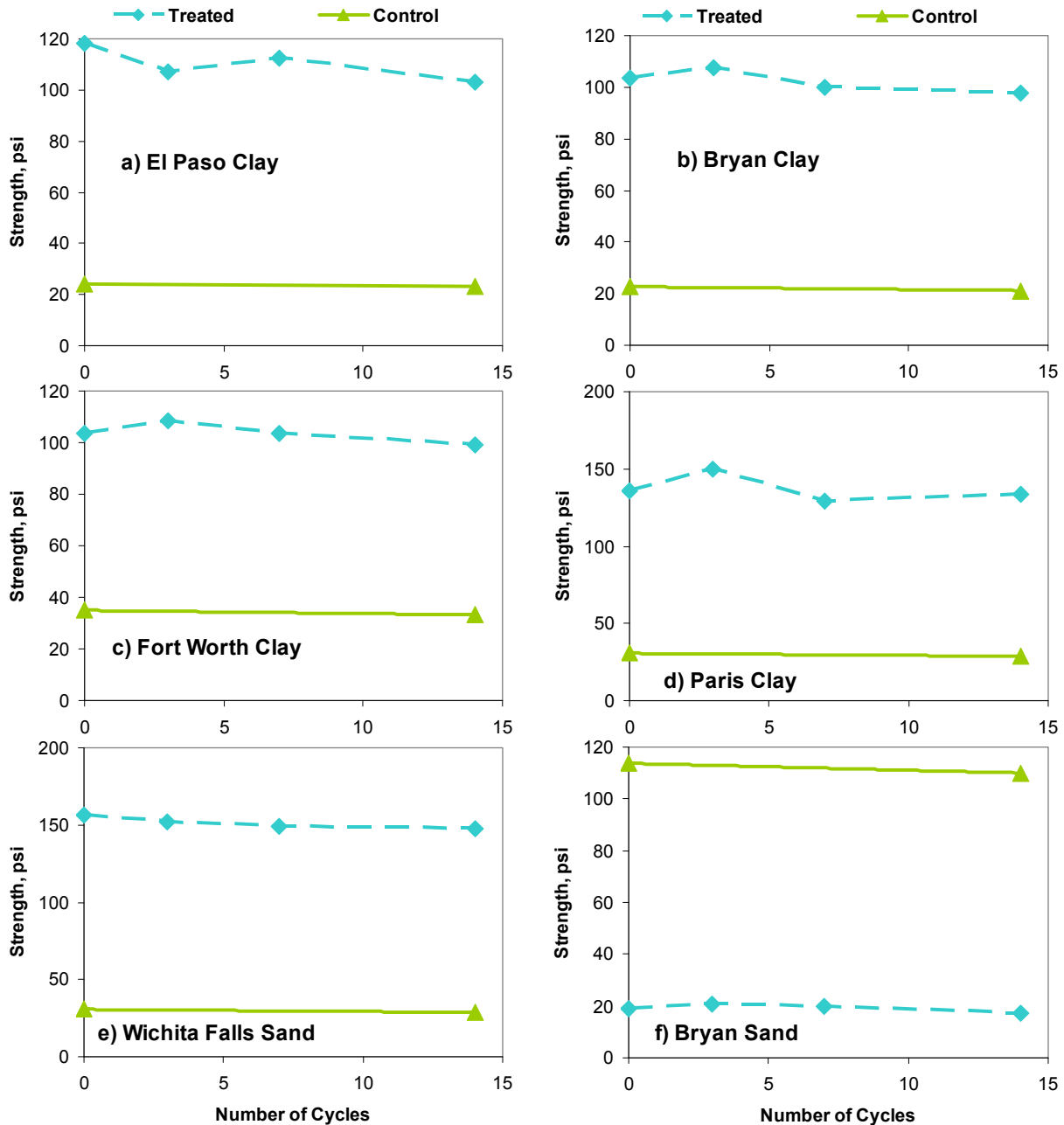
Figure 5.9 – Variation of UCS Strength with the Number of Leaching Cycles for Different Soil Samples
