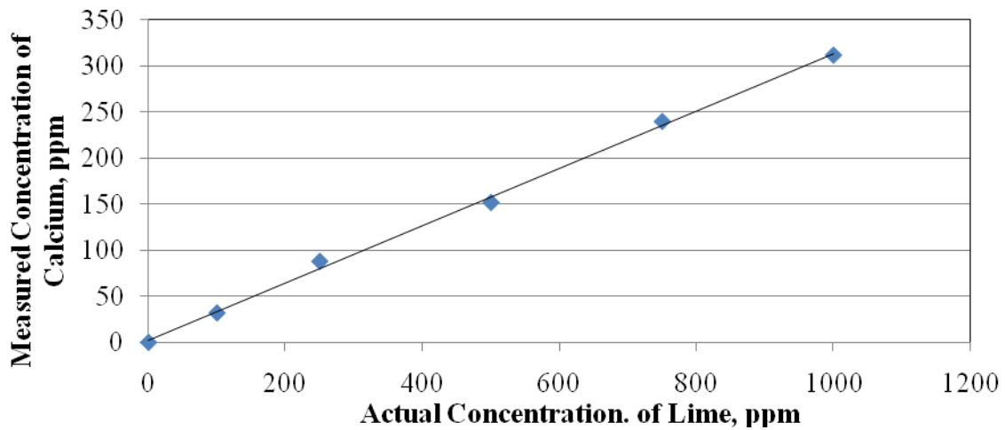
Figure 5.6 – Calibration Curve for Obtaining the Concentration of Lime from Concentration of Ca
