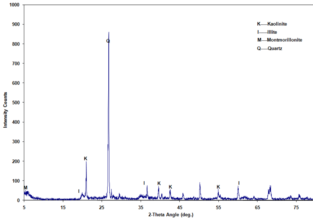
Figure B.1 – XRD Results of Bryan Soil before Treatment
