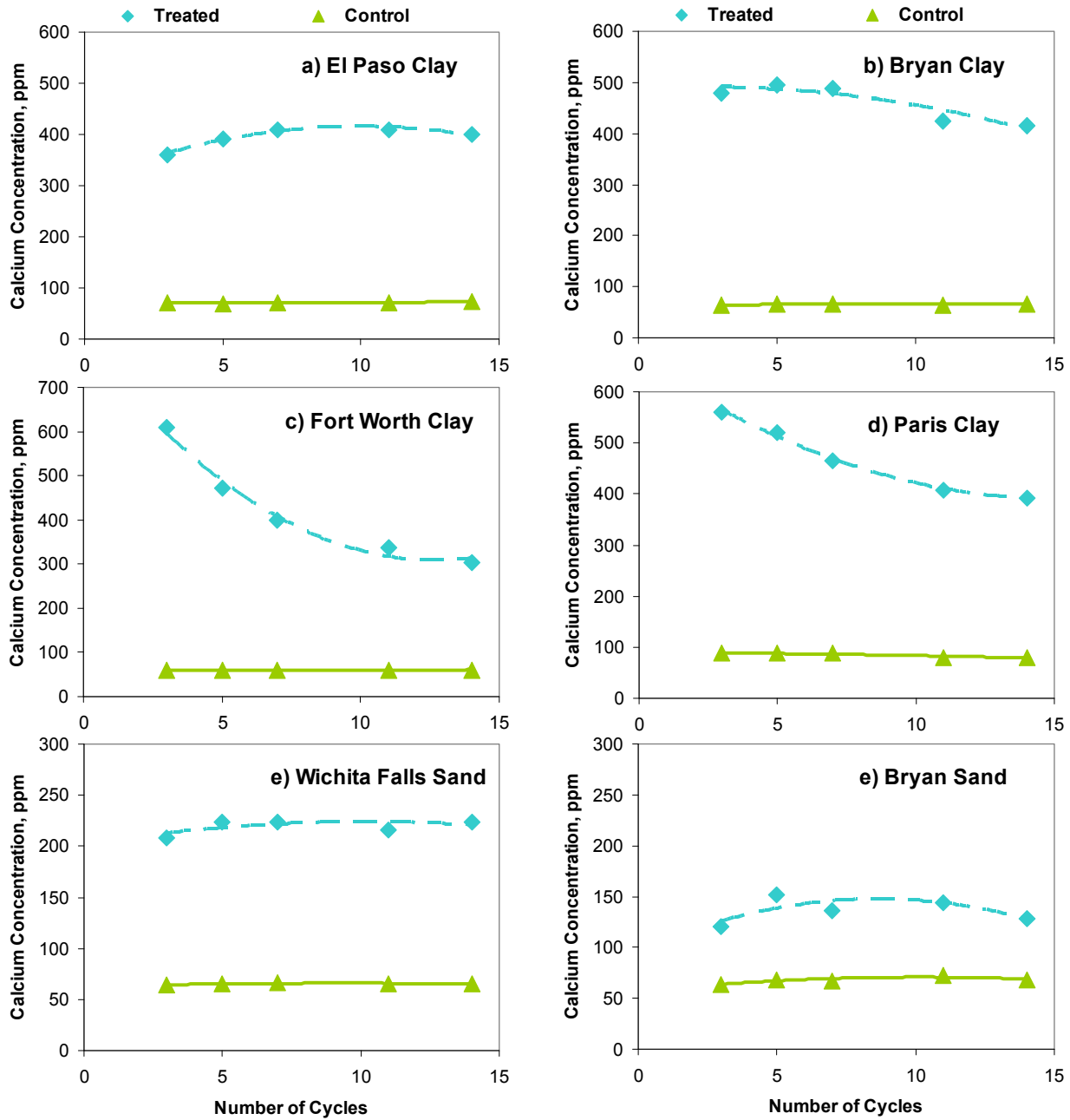
Figure 5.5 – Variation of Calcium Concentration of Different Soil Samples
