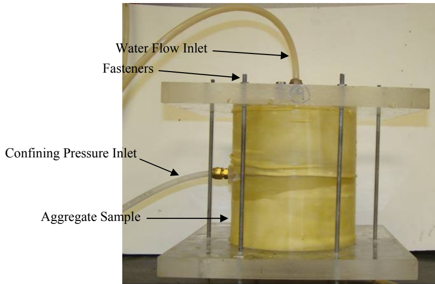
Figure 5.3 – Leachate Cell
