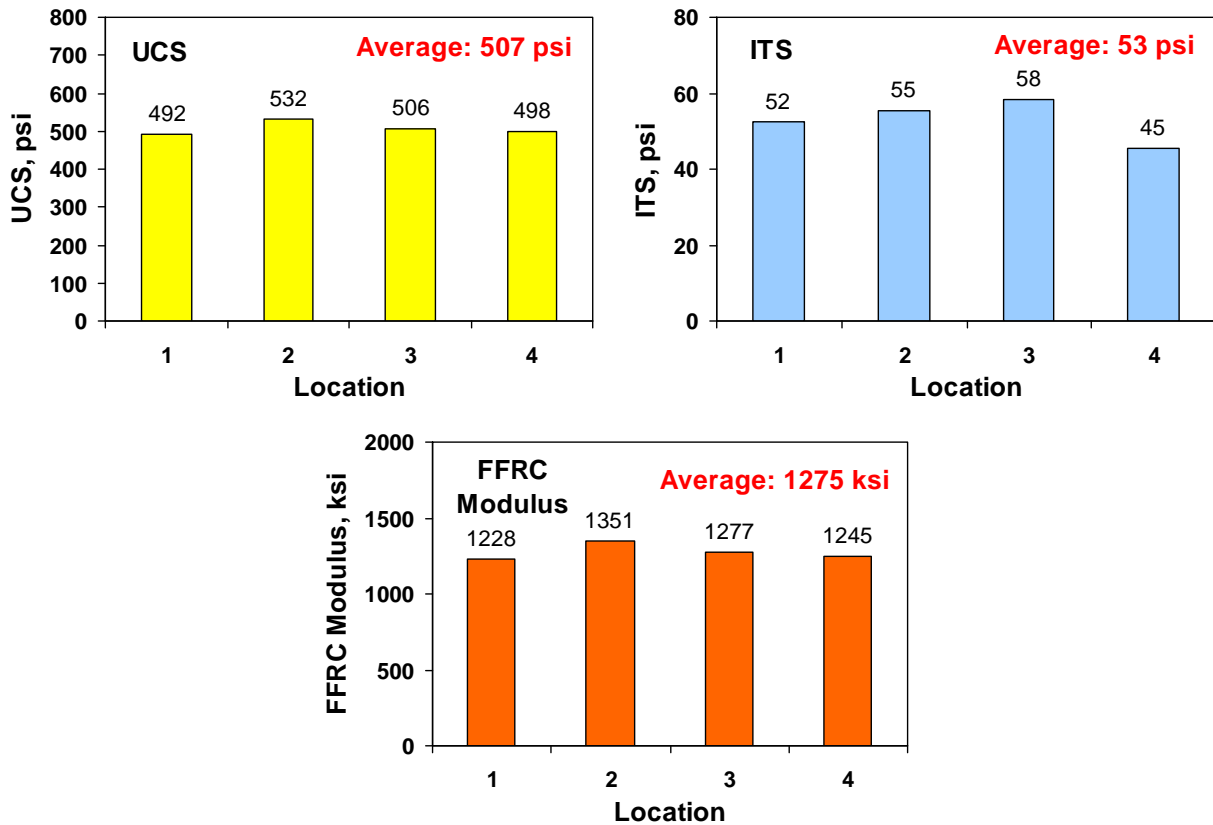
Figure 6.13 – Strengths and Modulus of 4% Cement-Treated Mix Used in the FM 2415 Project
