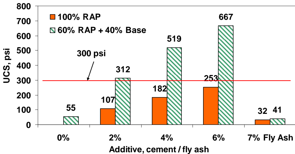
Figure 4.21 – UCS Values of Cement-Treated and Fly Ash-Treated El Paso RAP Mixes
