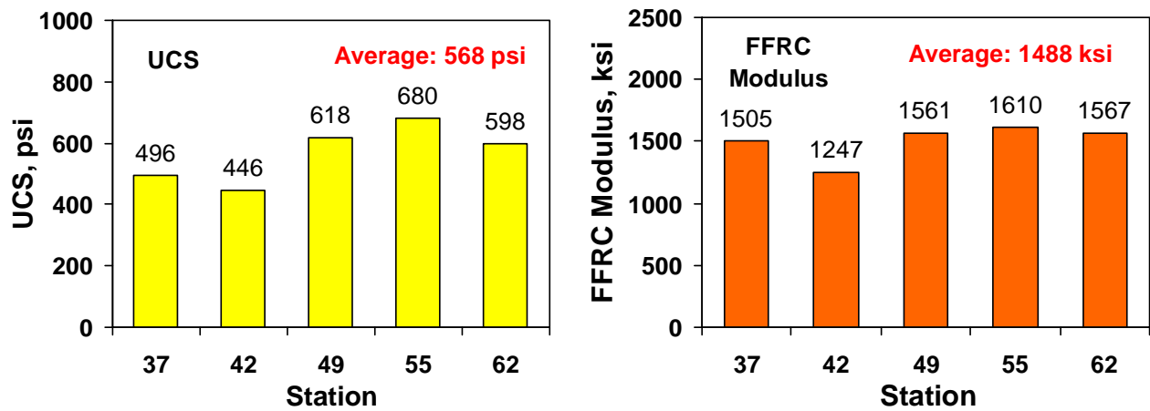
Figure 6.15 – UCS and FFRC Modulus of Cores from the New Base of the FM 2415 Project
