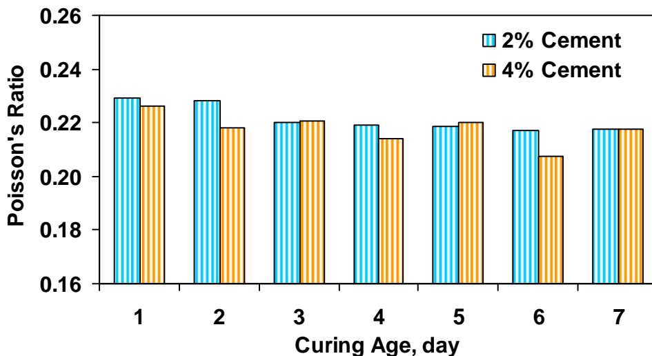
Figure 6.1 – Variations of Poisson's Ratio with Curing Age
