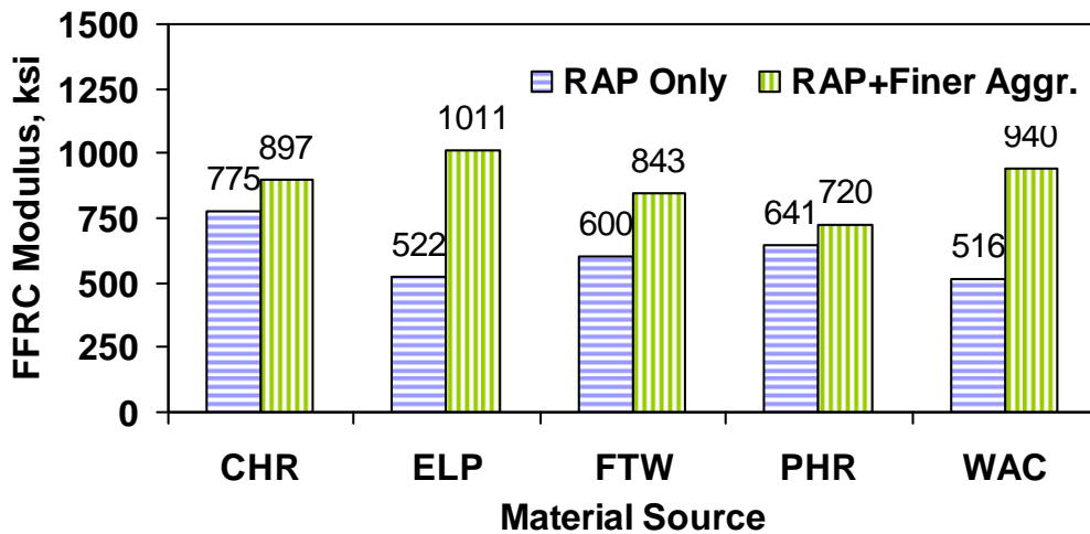
Figure 4.17 – Strength and Modulus of Mixes of RAP only and RAP Blended with Finer Aggregates
