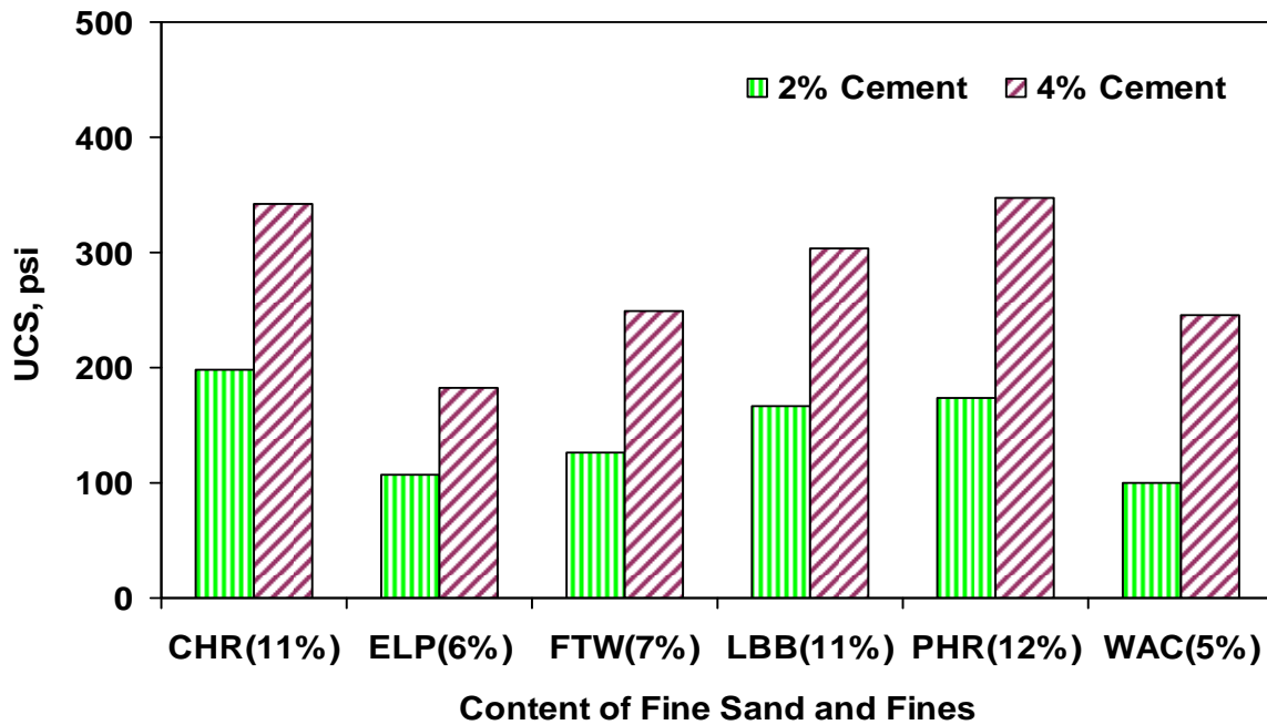
Figure 4.14 – Effect of Finer Aggregates (Passing #40 Sieve) on UCS of Mixes of 100% RAP
