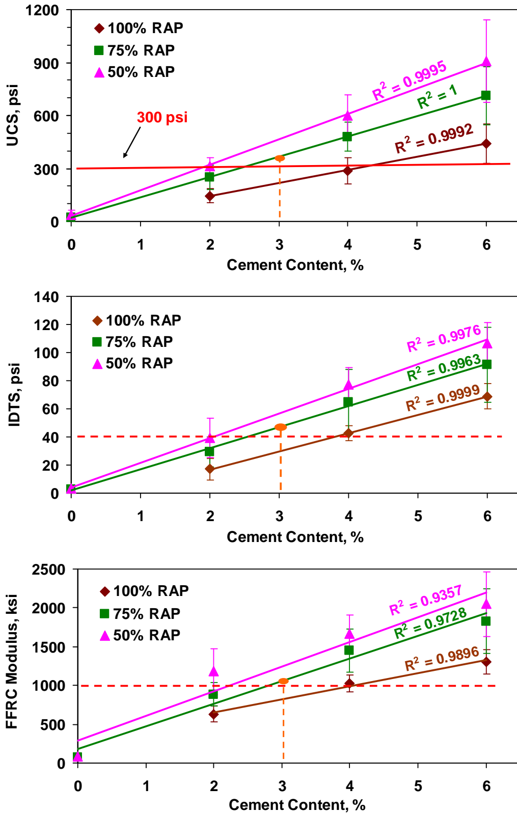
Figure 4.8 – Relationships between of Average UCS, ITS and Modulus and Cement Content
