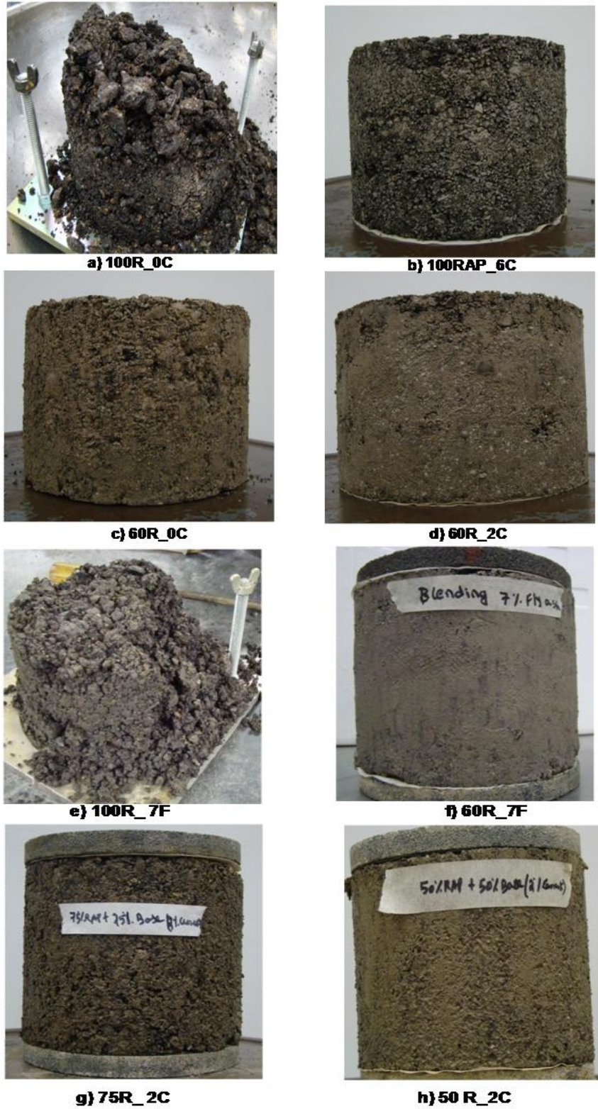
Figure 5.10 – Typical RAP and RAP Blends from El Paso District Prior to Wetting/Drying
