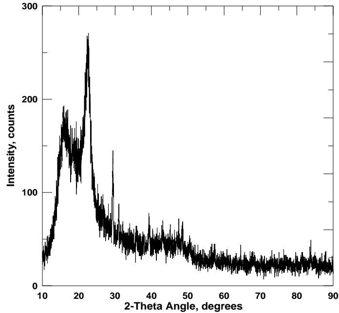
Figure 5.12 – Typical XRD Plot for 60R_2C Mix (Powered) from El Paso District
