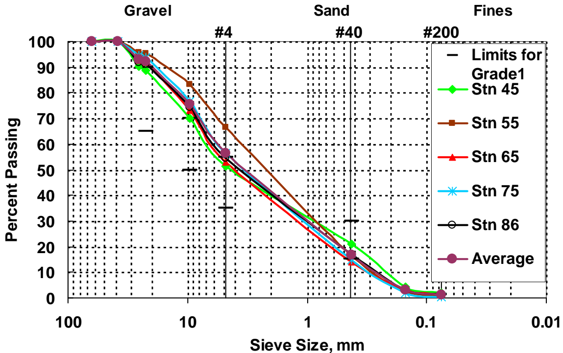
Figure 6.8 - Gradation of the Mix Used in the FM 448 Project
