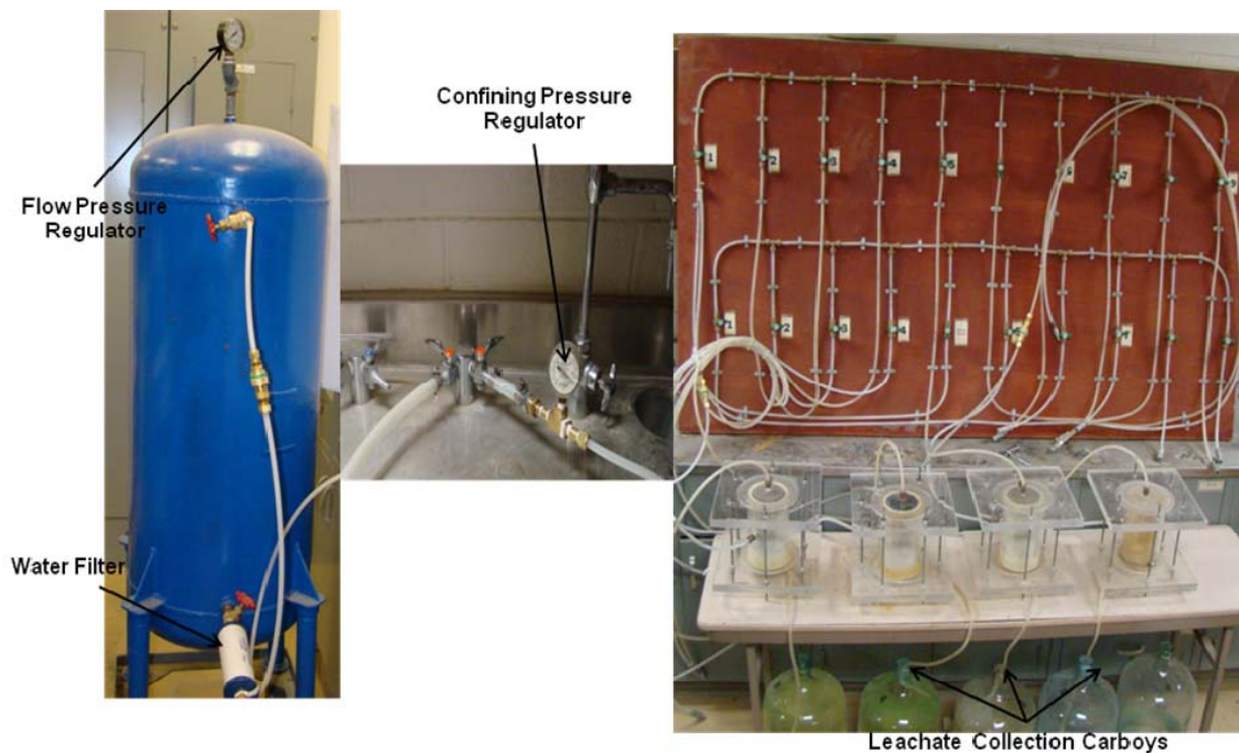
Figure 5.4 – Test Setup for Leachate Studies (Chittoori, 2008)
