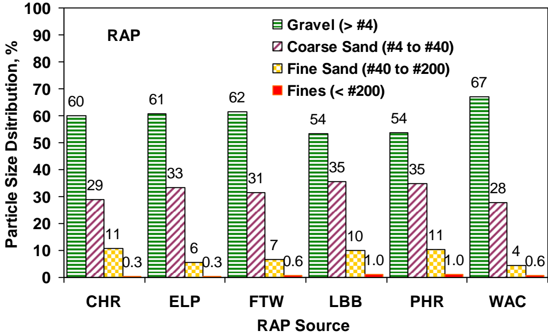
Figure 3.6 – Average Particle Size Distributions of RAP Materials
