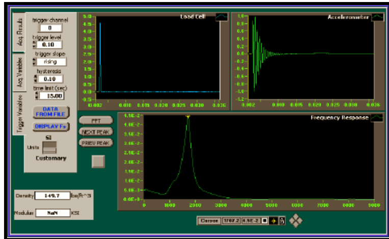
b) Records from a FFRC Test
