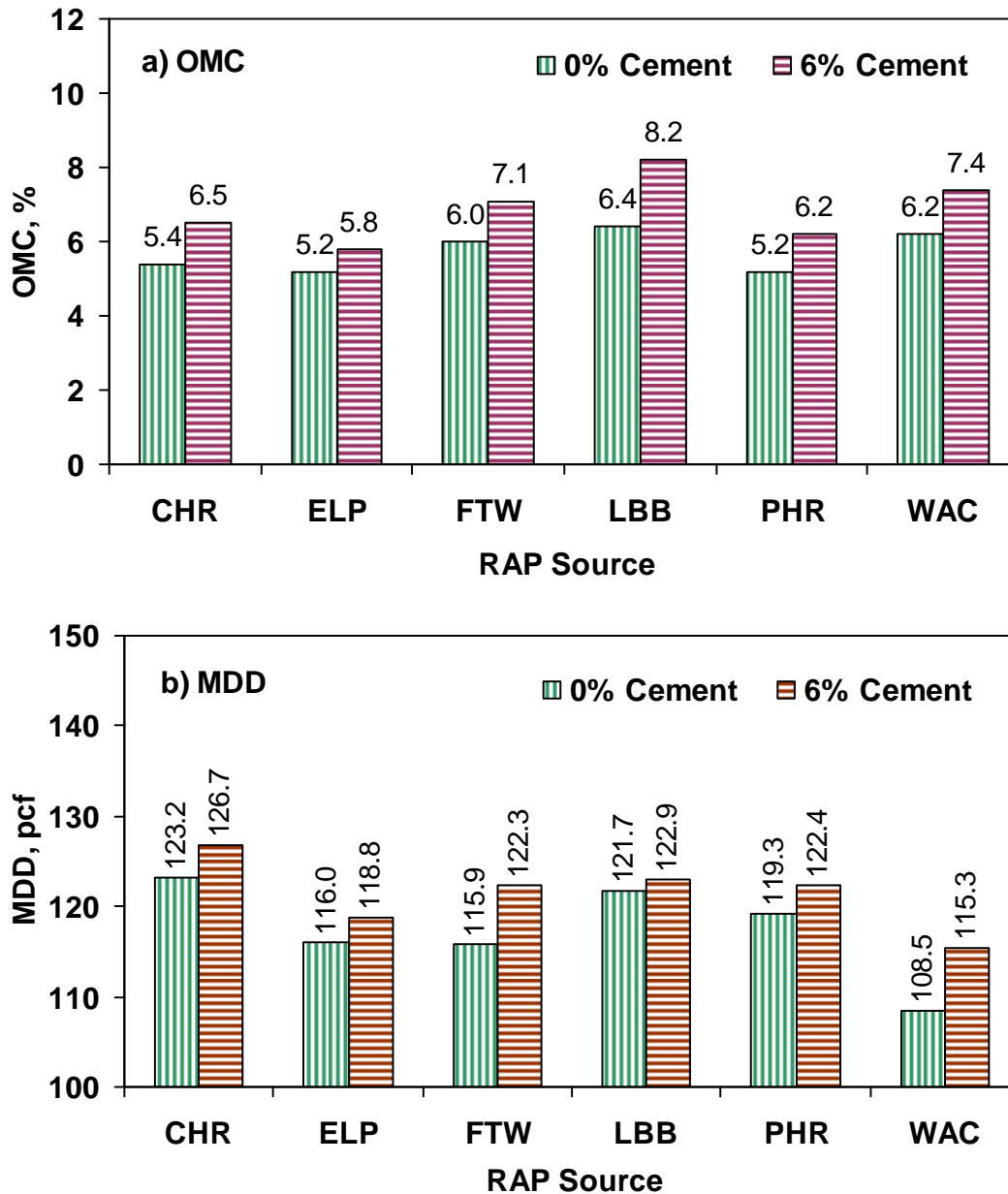
Figure 4.6 – Comparisons of OMC and MDD of 100% RAP Mixes without Treatment and Treated with 6% Cement
