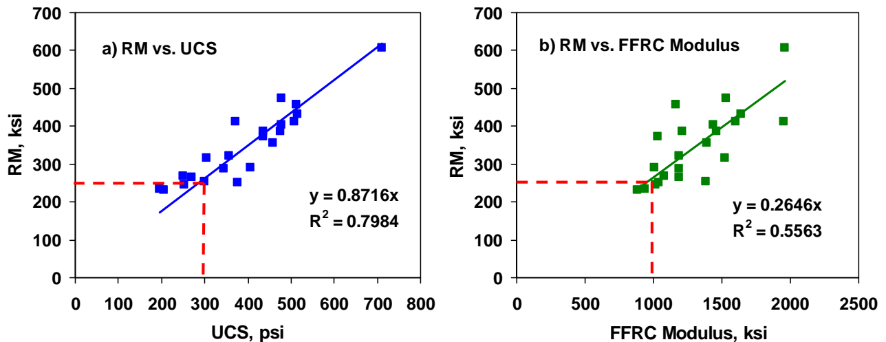
Figure 4.9 – Resilient Modulus vs. UCS and FFRC Modulus
