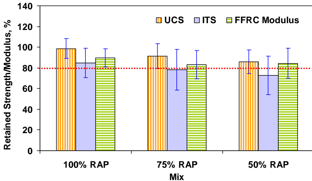
Figure 4.10 – Average Retained Strengths and Modulus
