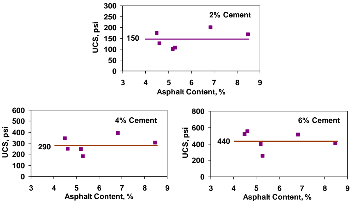
Figure 4.12 – Variations of UCS with Asphalt Content in Mixes of 100% RAP
