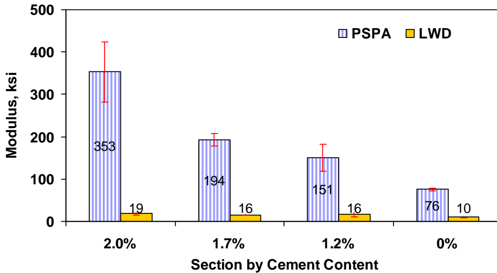
Figure 6.6 – Moduli Measured with PSPA and LWD on the New Base of FM 378
