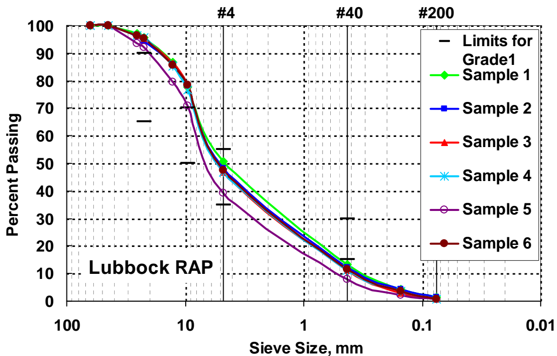
Figure 3.4 – Gradations of RAP Collected from Different Locations at Lubbock Stockpile
