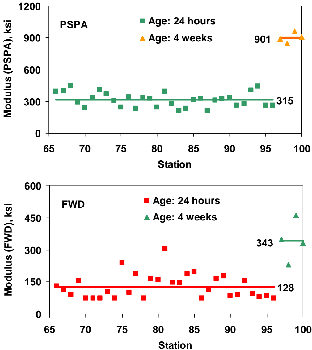
Figure 6.10 – Moduli from PSPA and FWD Tests on the New Base of the FM 448 Project
