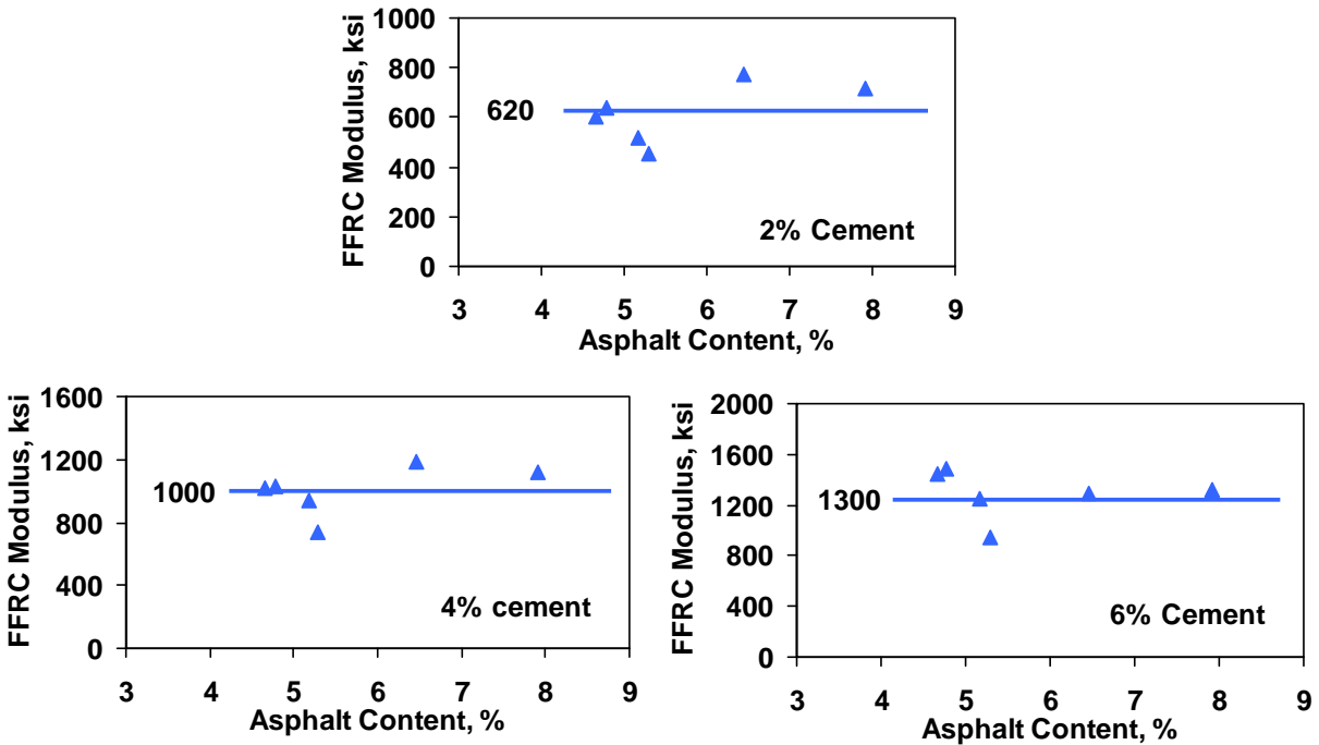
Figure 4.13 – Variations of FFRC Modulus with Asphalt Content in Mixes of 100% RAP
