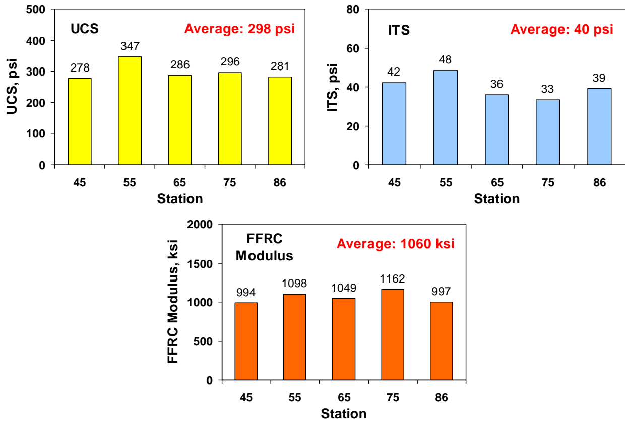
Figure 6.9 – Strengths and Modulus of 3% Cement-Treated Mix Used in the FM 448 Project
