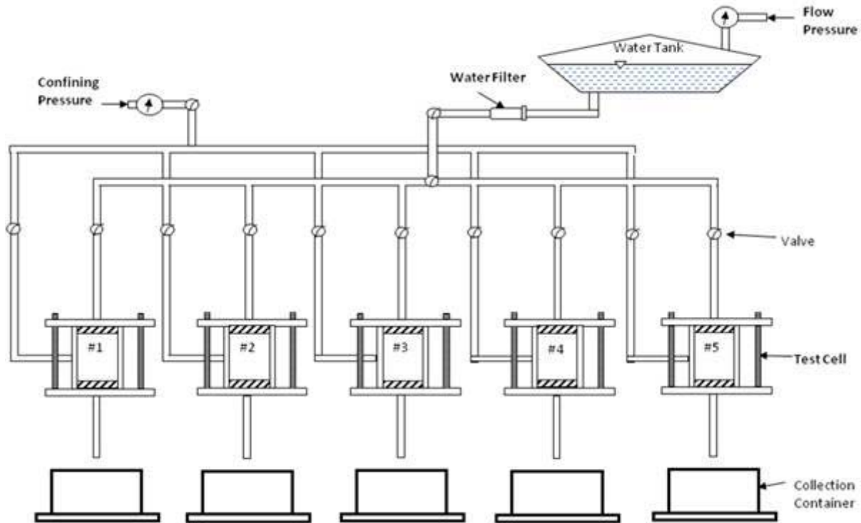
Figure 5.2 – Schematic of Leachate Process (Chittoori, 2008)
