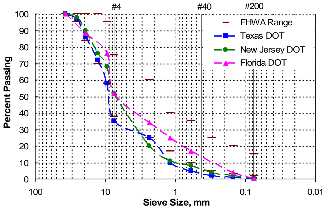
Figure 2.2 – Typical RAP Gradations
