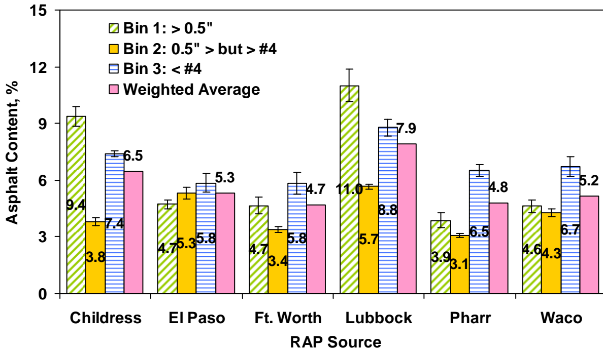
Figure 3.2 – Comparison of Asphalt Contents of RAP Materials from All Six Stockpiles
