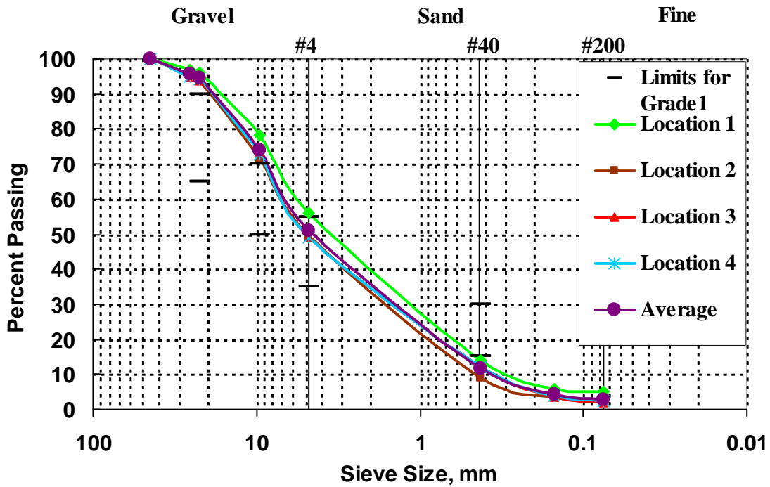
Figure 6.12 - Gradation of the Mix Used in the FM 2415 Project
