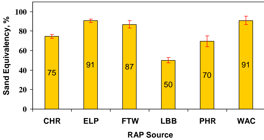
Figure 3.9– Sand Equivalent Values of RAP Materials from all Six Stockpiles
