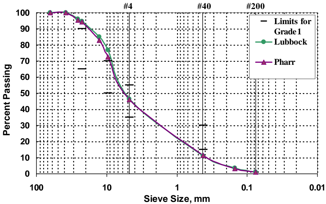
Figure 3.7 – Comparison of Gradations of RAP
