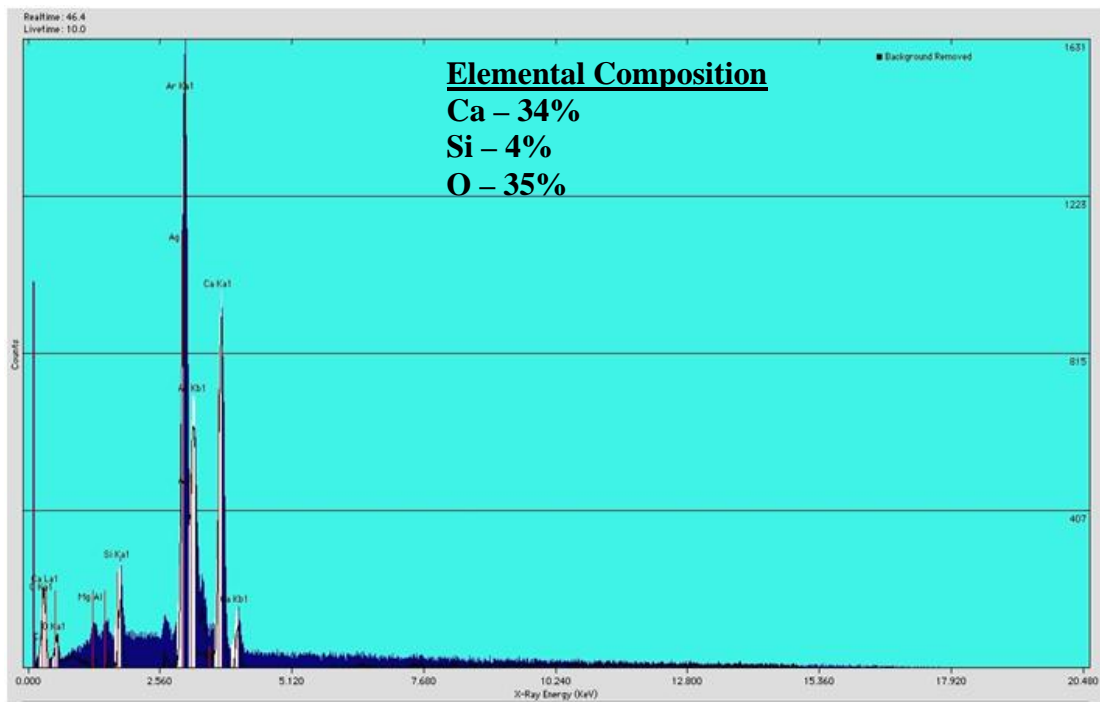
Figure 5.20 – Typical EDS Plot for 100R_6C Mix (Powered) from El Paso District
