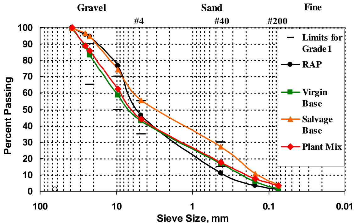
Figure 6.4 – Gradation of the Mix Used in the FM 378 Project
