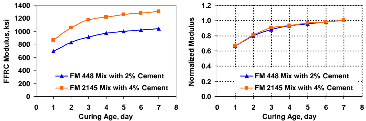
Figure 6.2 – FFRC Modulus Gain with Curing Age
