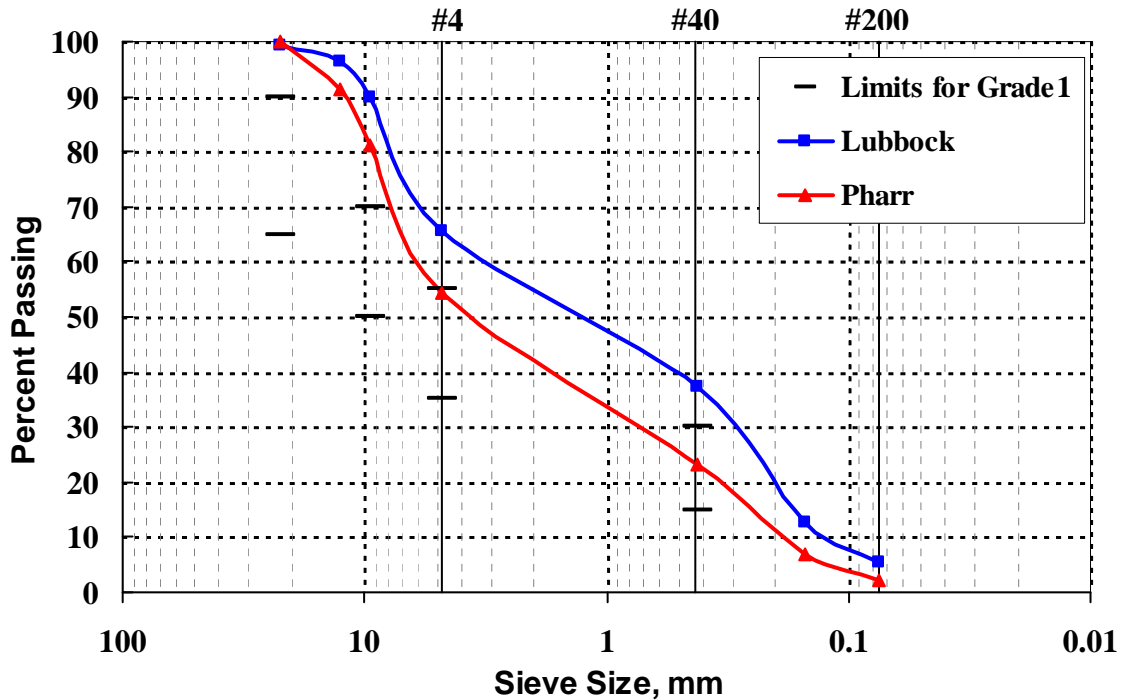
Figure 3.8 – Comparison of Gradations of Recovered Aggregates of RAP
