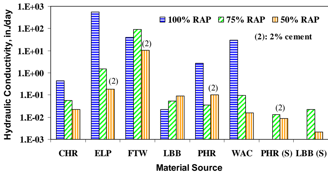
Figure 4.11– Hydraulic Conductivities of Different Mixes
