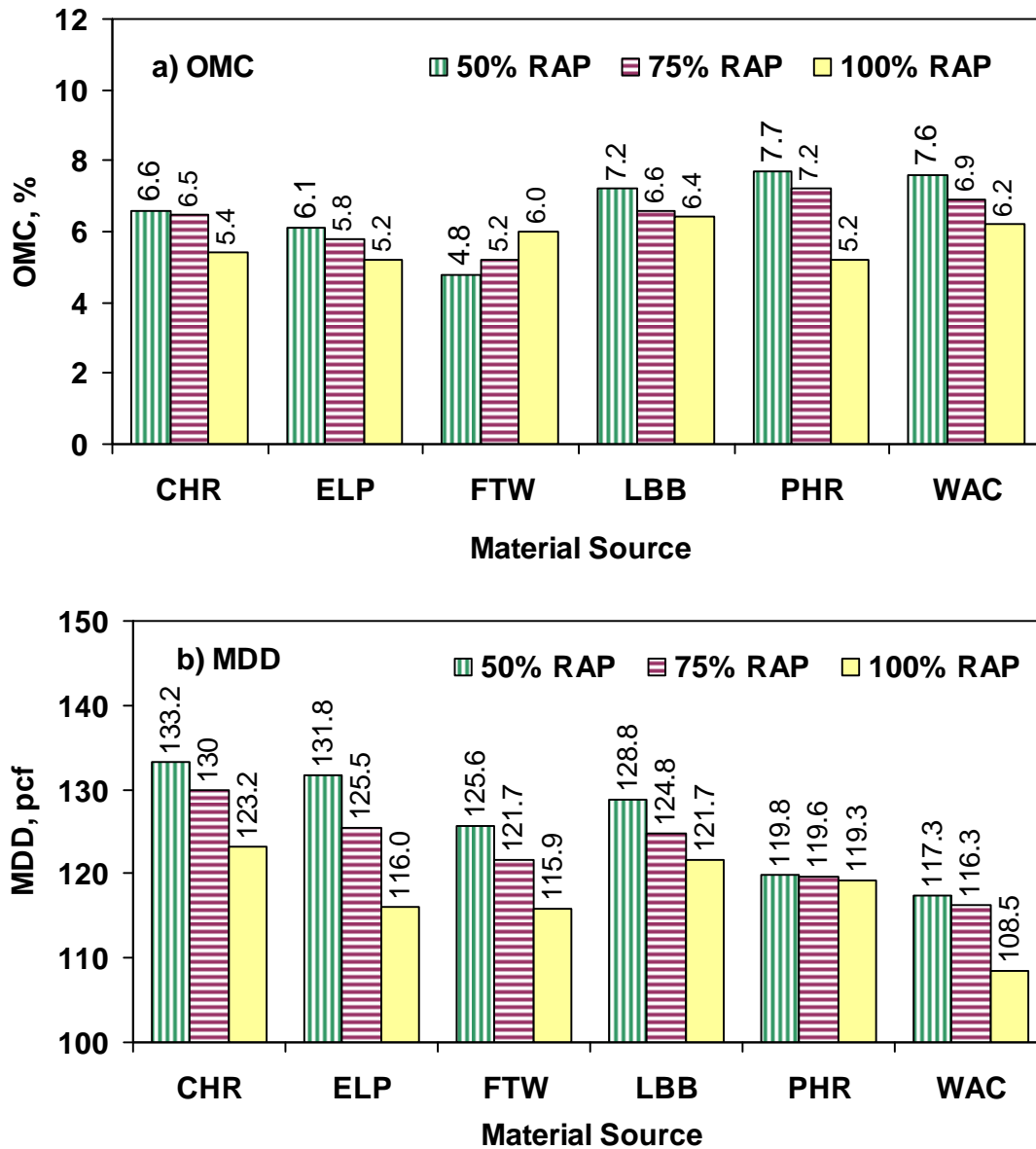
Figure 4.5 – Variations of OMC and MDD with RAP Content in Untreated Mixes
