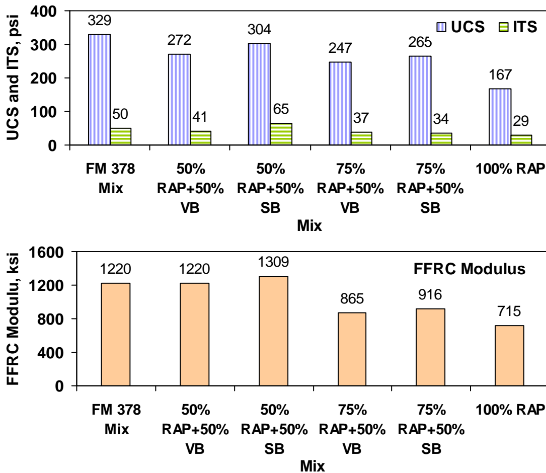
Figure 6.5 – Comparison of Strength/Modulus of Mixes of Different RAP Contents and Different Granular Materials Treated with 2% Cement
