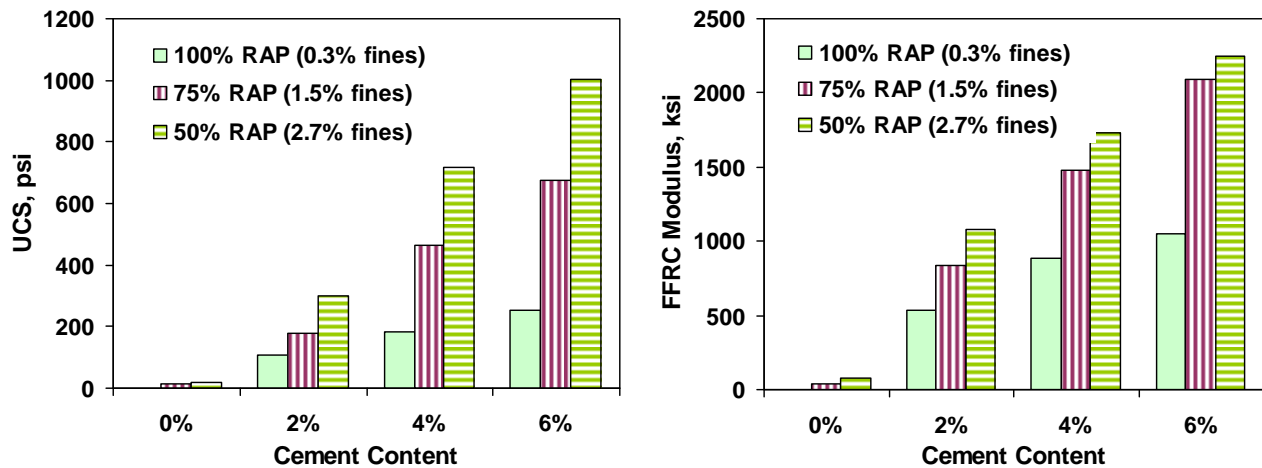
Figure 4.15 – Effect of Fines (Passing #200 Sieve) Content on UCS and FFRC Modulus of El Paso Mixes
