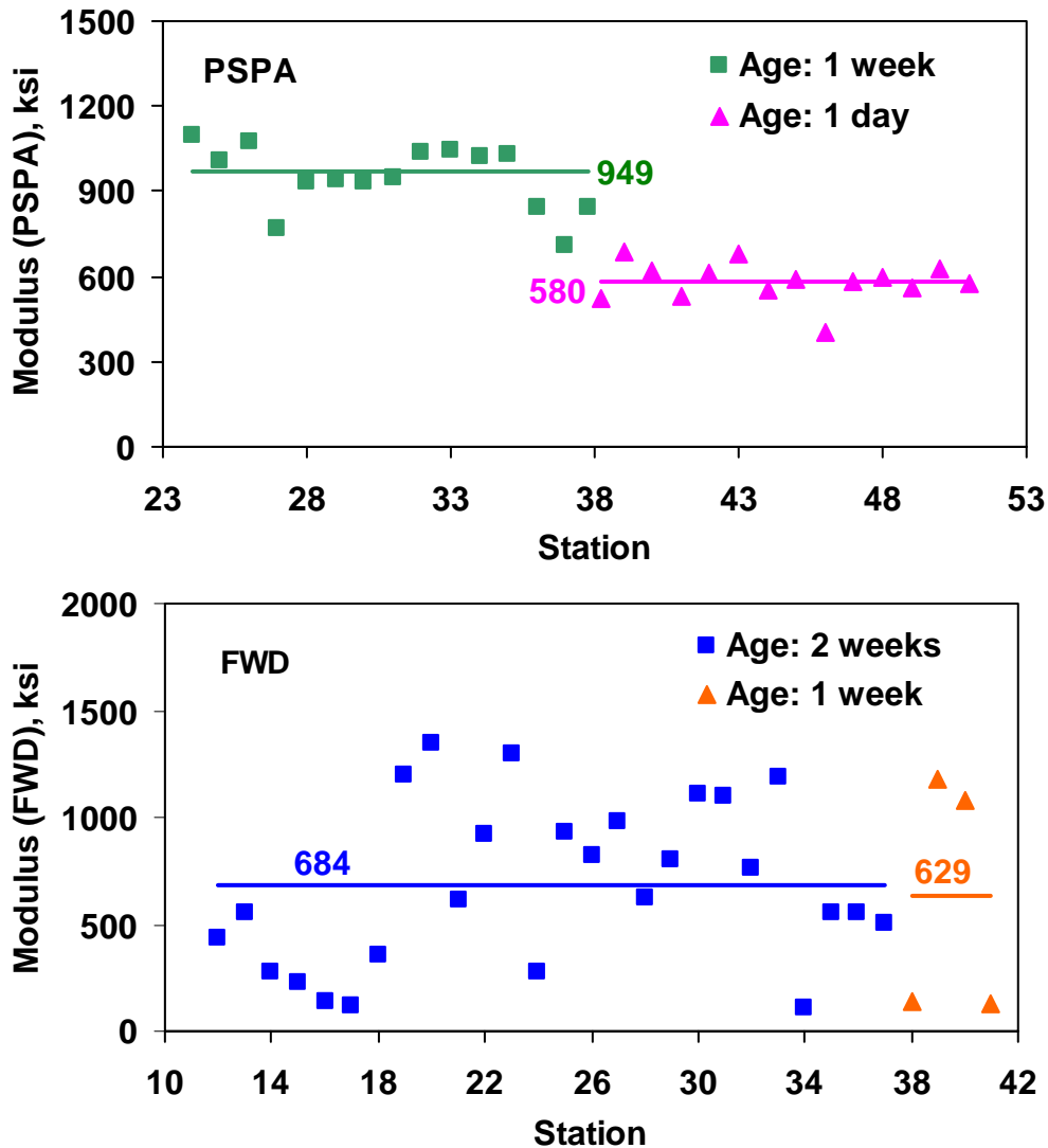
Figure 6.14 – Moduli from PSPA and FWD Tests on the New Base of the FM 2415 Project
