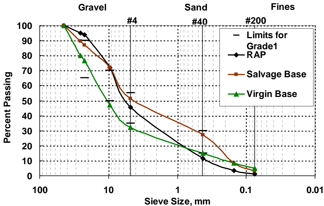
Figure 4.18 – Gradations of RAP, Salvage Base and Virgin Base from Pharr District
