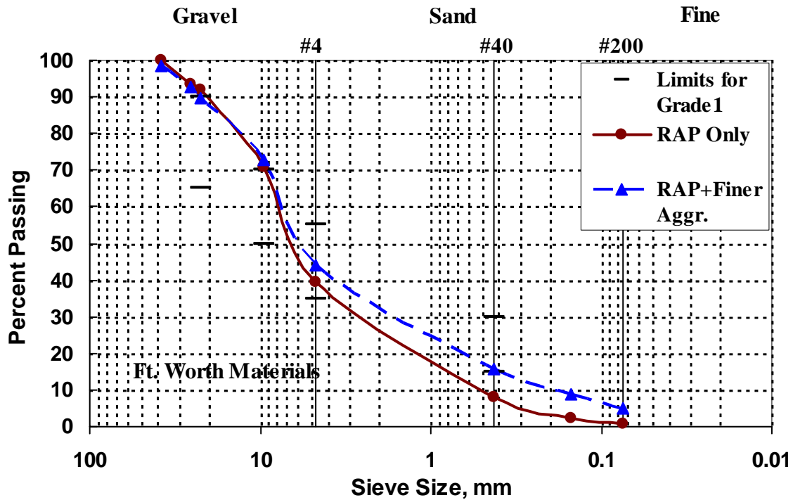
Figure 4.16 – Comparison of Gradations of Natural RAP and Modified RAP Mixes
