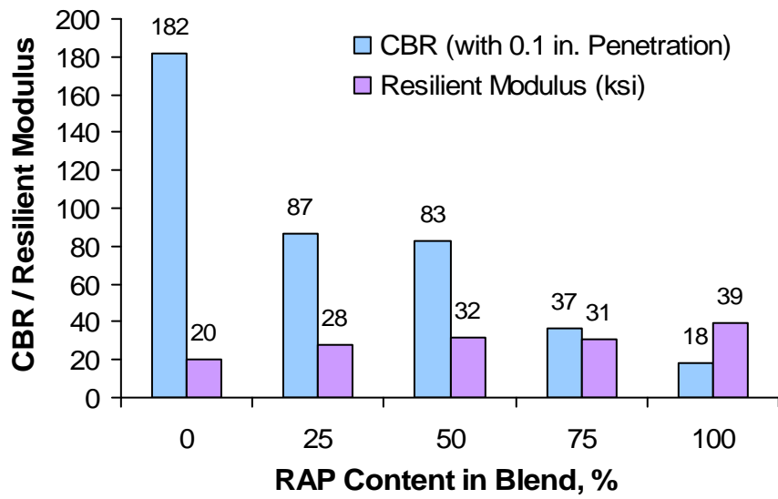
Figure 2.3 – Variations of CBR and Resilient Modulus with RAP Content (from Bennett and Maher, 2005)
