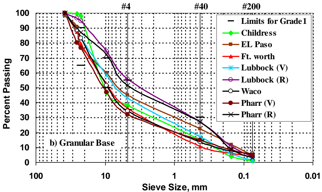
Figure 3.5 – Comparison of Gradations of RAP and Granular Base Materials
