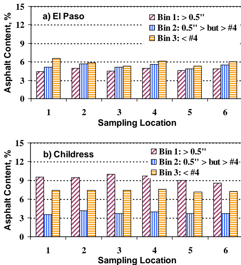
Figure 3.1 – Asphalt Contents of RAP Materials by Bin and Sampling Location
