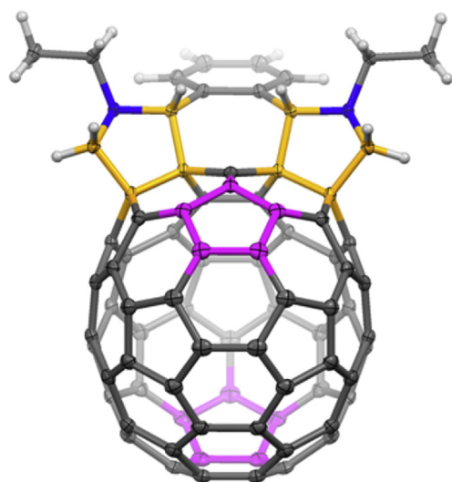
Fig. 6. Crystallographically determined structure of compound 1 ( meso - \beta -2- \beta endo-endo ) from the solvate, 1 -toluene. The apical pentagons of C_{70} are shown in pink and the pyrrolidine rings attached to the \beta -bonds are yellow. Nitrogen atoms are blue. Thermal ellipsoids are drawn at the 0.50 level. (A colour version of this figure can be viewed online.)
