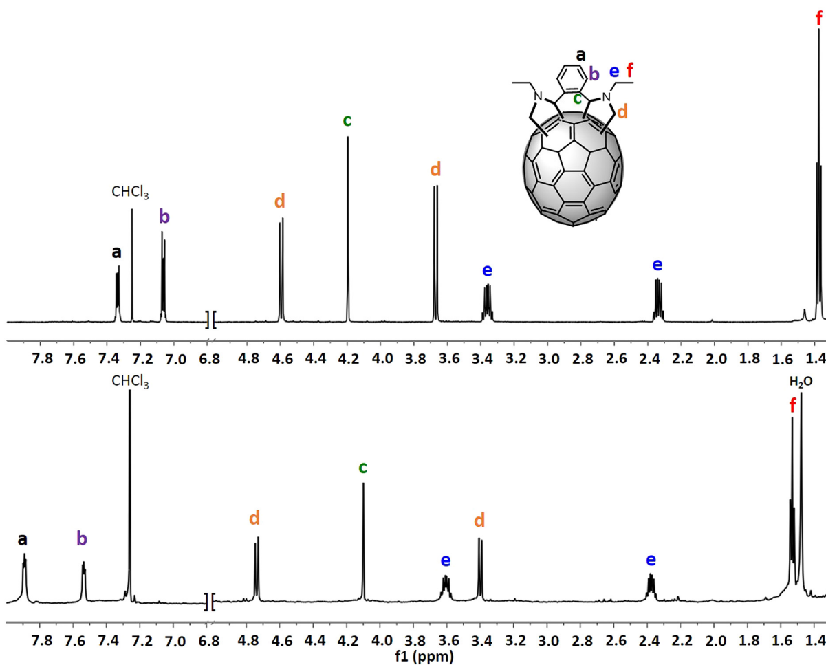
Fig. 4. ^1\text{H} NMR spectrum of compound 1 (top) and compound 2 (bottom) (600 MHz, 298 K, \text{CS}_2:\text{CDCl}_3 1:1). (A colour version of this figure can be viewed online.)
