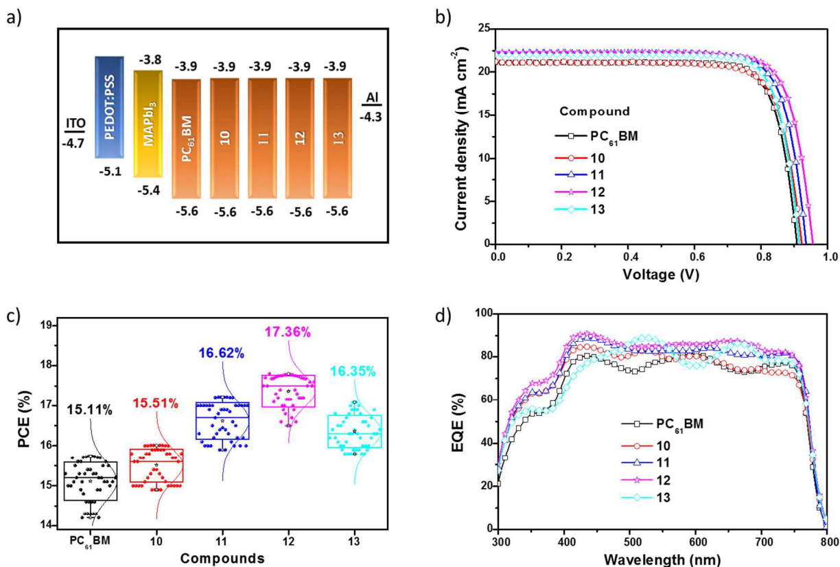
Figure 3. a) Schematic illustration of the estimated HOMO and LUMO energy levels, calculated from CV and UV-vis. b) J-V curves under 1 sun illumination (100 mW/cm 2 ) in forward voltage scans. c) The PCE histograms measured for 48 independent cells. d) EQE spectra for the PSCs fabricated using compounds 10-13 and PC 61 BM as the ETMs.
