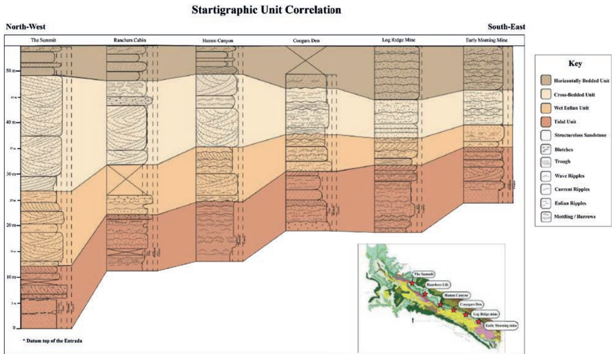
Figure 3.0 - Stratigraphic cross-section illustrating the lateral thickness distribution of individual stratigraphic units documented
