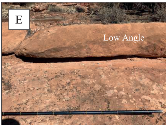
Figure 2.2.4 Small Eolian Dune Facies Association
