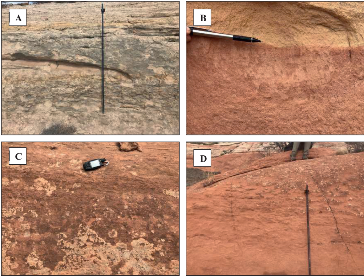
Figure 2.1.7 – A) Meter scale beds of white bioturbated sandstone (Photo taken at the Hamm Canyon section). B) Individual bed of well defined vertical burrows in contact with a bed of featureless sandstone above (Photo taken at Little Gypsum Valley). C) Close up view of burrowed sandstone lichen cover (Photo taken at the Log Ridge Mine section). D) Red-peach colored bed of bioturbated sandstone (Photo taken at the Ranchers Cabin section).
