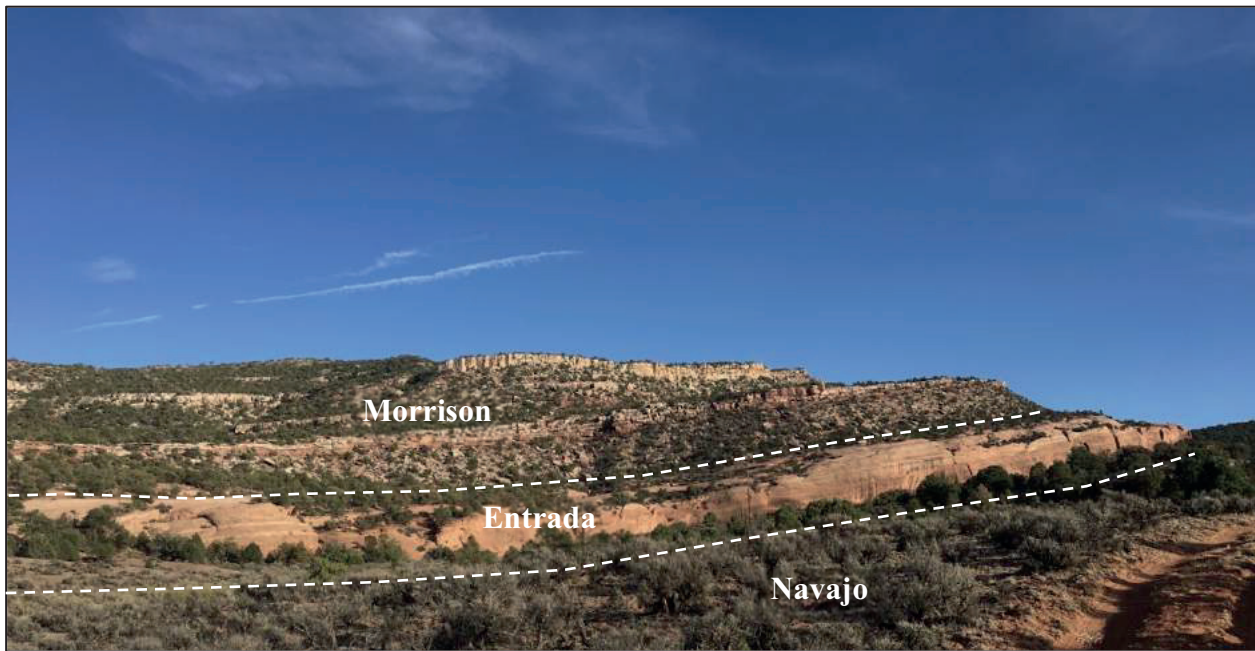
Figure 5.2 Outcrop photo taken on the southern end of Hamm Canyon showing the wedge geometry of the Entrada Sandstone along the flank of the Gypsum Valley salt wall.
