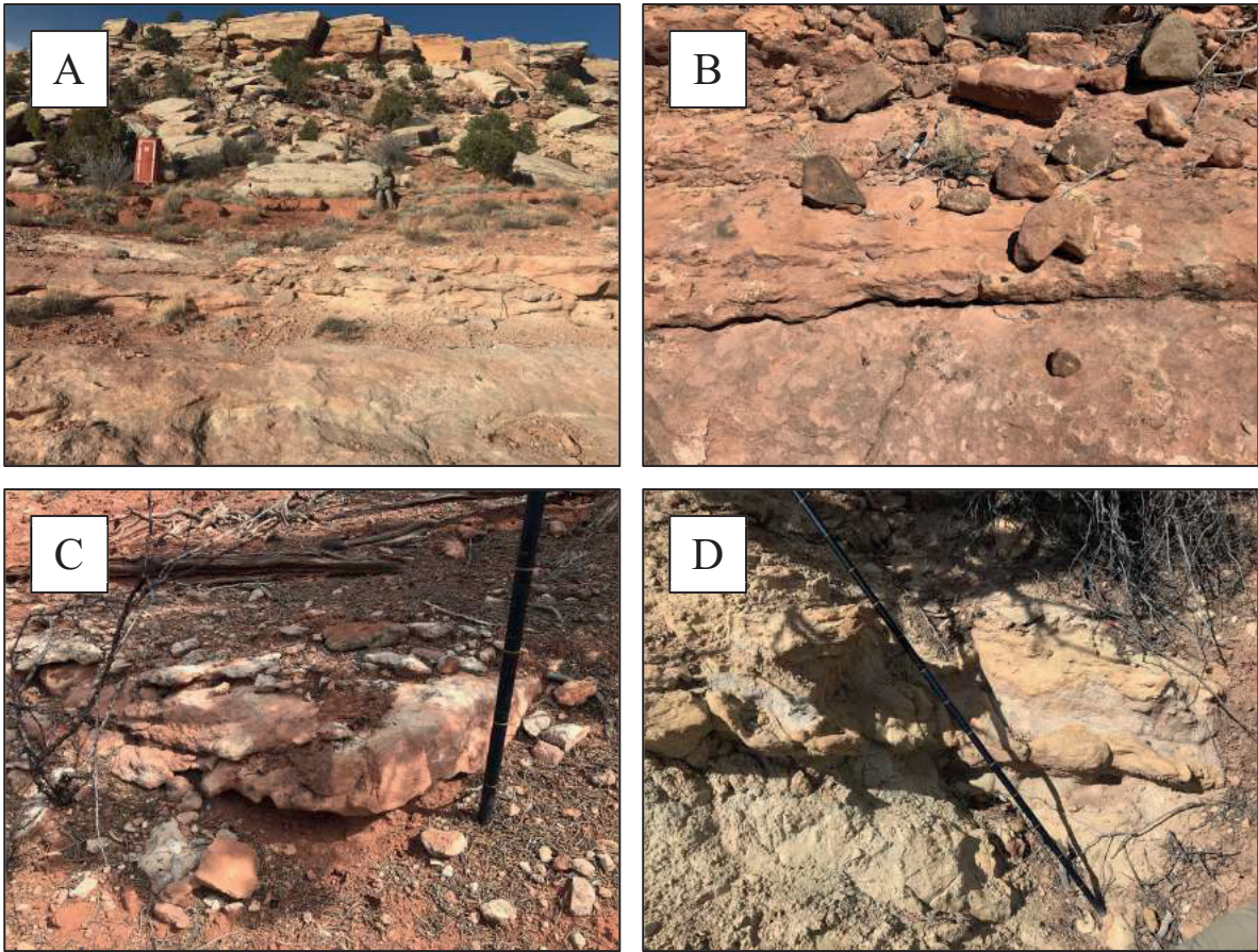
Figure 2.2.5 Scoured Eolian Facies Association: A) Outcrop exposure of small ledges of scoured eolian sediments that have a variety of colors produced by variability in oxidation (Photo from the Ranchers Cabin section). B) Close up view of a scoured bed lacking any sedimentary structures (Photo taken at the Hamm Canyon section). C) Example of varying degrees of oxidation (Photo taken at the Summit section). D) Small exposure of scoured sands that are white-tan in color (Photo taken at the Log Ridge Mine section).
